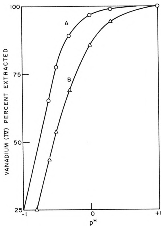
Fig. 5. Extraction of Vanadium (IV) Cupferrate into Ethyl Acetate from HCl Solution. Cupferron Concentration in Organic Phase: Curve A, 9 \times 10^{-2} M; Curve B, 6 \times 10^{-2} M.
