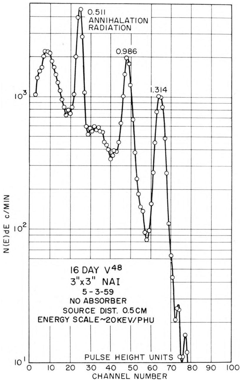
Figure 11. Gamma Spectra of Vanadium-48. The 2.30 Mev sum peak is not shown. (139)
