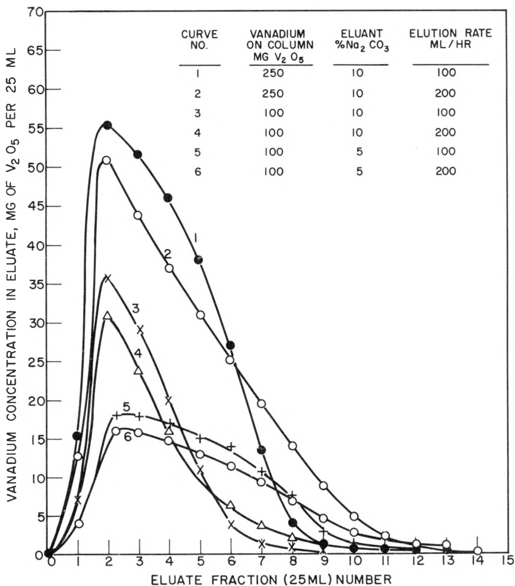
Figure 7. Elution of Vanadium(V) from IRA-400 with sodium carbonate.
