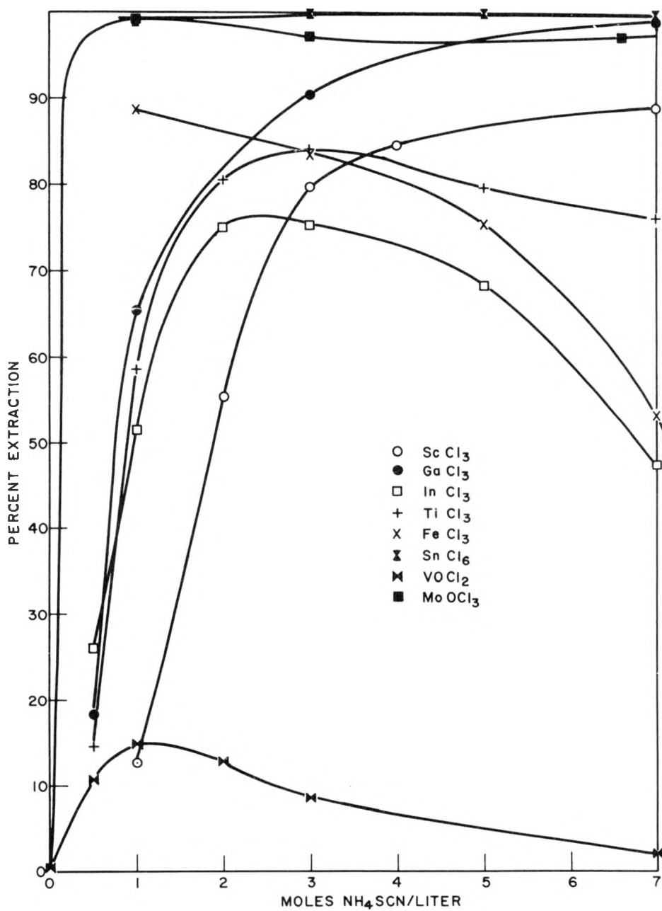
Figure 3 Extraction of Thiocyanates into Ethyl Ether.
