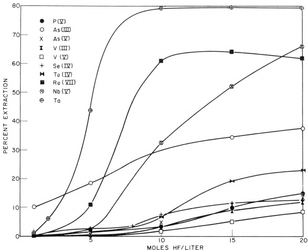
Figure 2. Distribution of fluorides between HF solution and ethyl ether.
