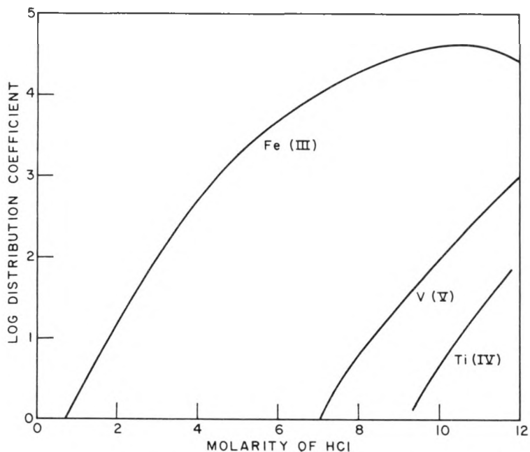
Figure 9. Distribution of Vanadium (V), Iron (III) and Titanium (IV) Between HCl Solution and Dowex-1.
