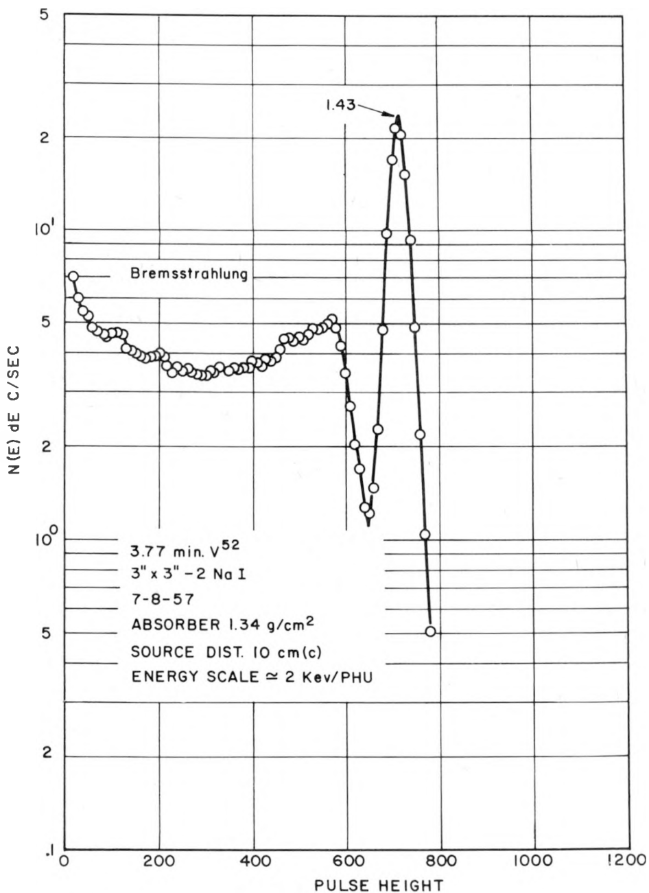
Figure 12. Gamma Spectra of Vanadium-52. (139)
