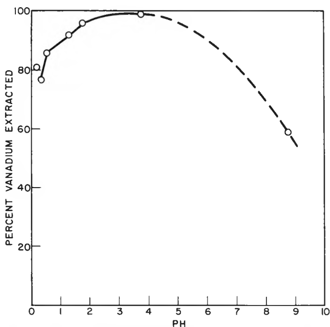
Fig. 4. Extraction of Vanadium (V) Cupferrate into Chloroform from \text{H}_2\text{SO}_4 Solution.
