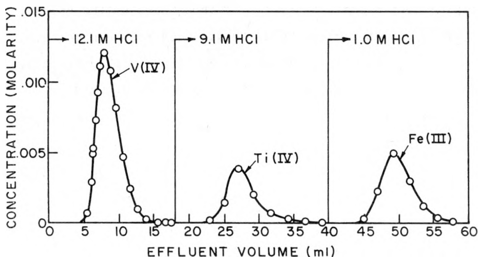
Figure 8. Separation of V(IV), Ti(IV) and Fe(III) by anion exchange (18.6 cm. x 0.49 cm 2 Dowex-1 column; 1 ml 0.05 M V(IV), 0.018 M Ti(IV), 0.025 M Fe(III) in 12 M HCl.
