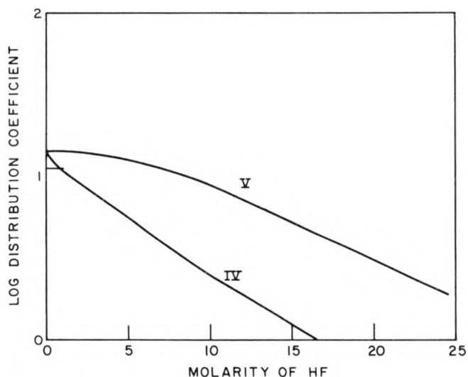
Figure 10. Distribution of Vanadium (IV and V) Between HF Solution and Dowex-1 Anion Exchange Resin.
