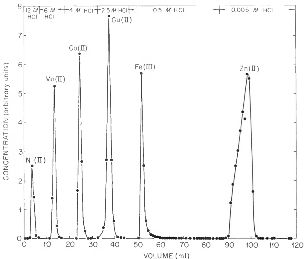
Figure 3. Separation of Transition Elements Mn to Zn. (Dowex-1 Column; 26 cm x 0.29 cm., flowrate = 0.5 cm/min.). Taken from Kraus, K. A. and Moore, G. E., J. Am. Chem. Soc. , 75 , 1460 (1953).
