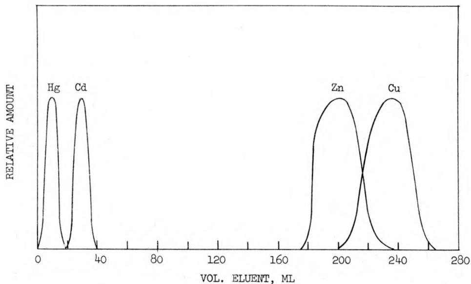
Figure 2. Elution curves for some of the divalent metal ions; 3.1 M HCl used as eluent; ion exchange resin, Dowex 50, 200-400 mesh. (Taken from UCRL-2531. (82) )
