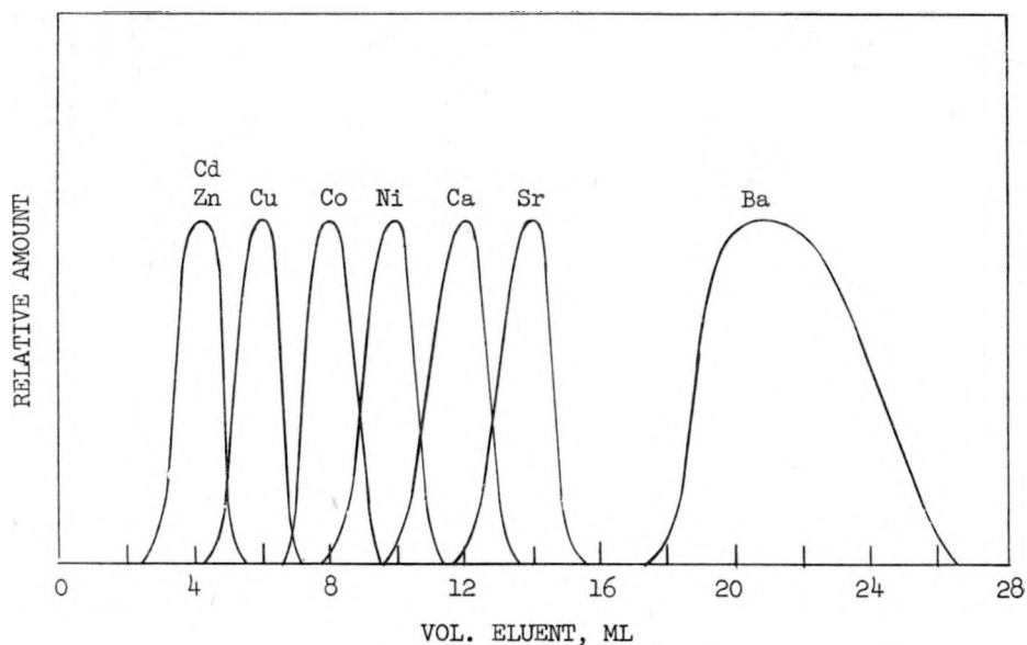
Figure 1. Elution curves for some of the divalent metal ions; 3.1 M HCl used as eluent; ion exchange resin, Dowex 50, 200-400 mesh. (Taken from UCRL-2531. (82) )
