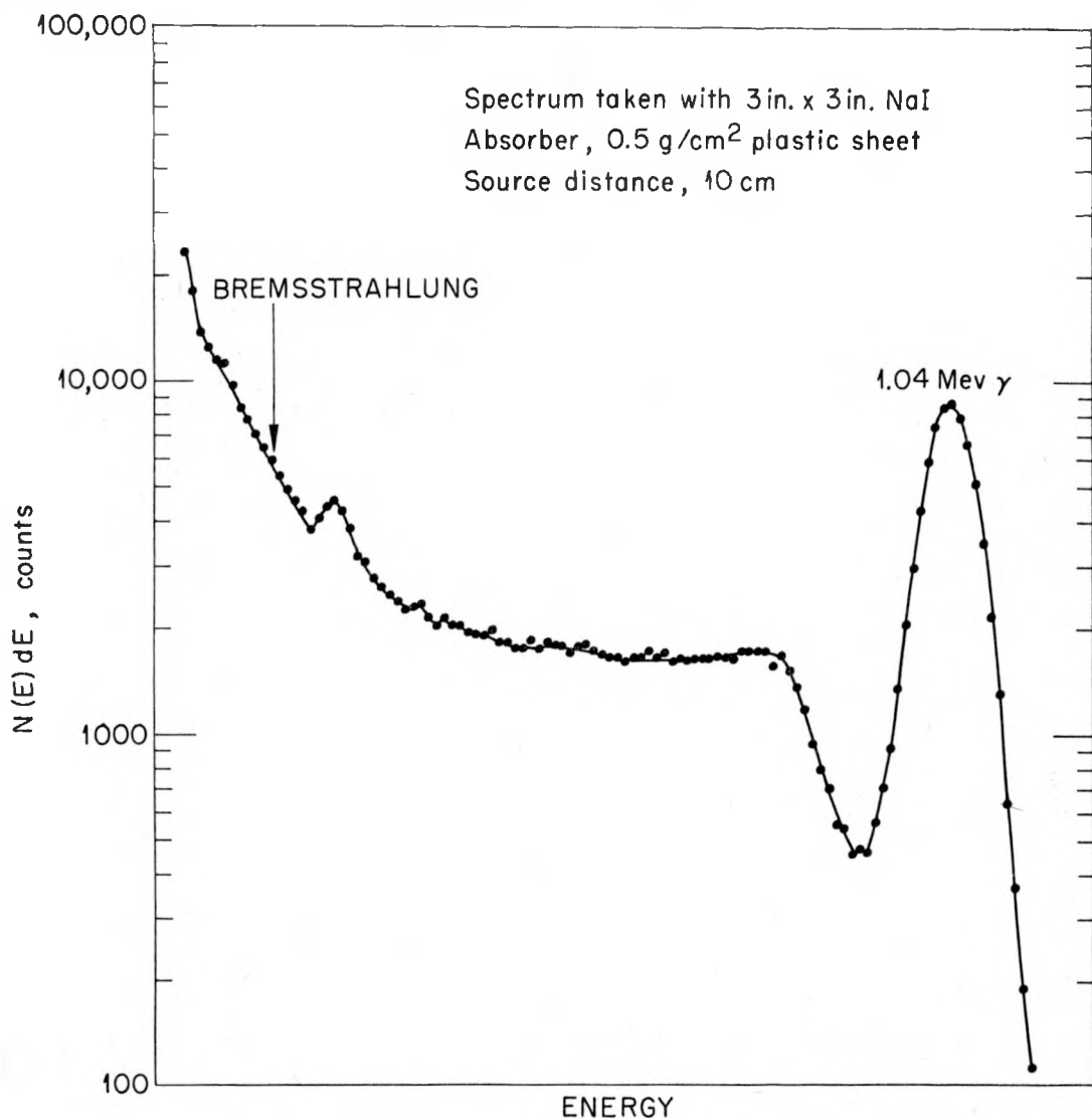
Fig. 6. Gamma-ray spectrum of \text{Cu}^{66} , half-life = 5.1 min.
