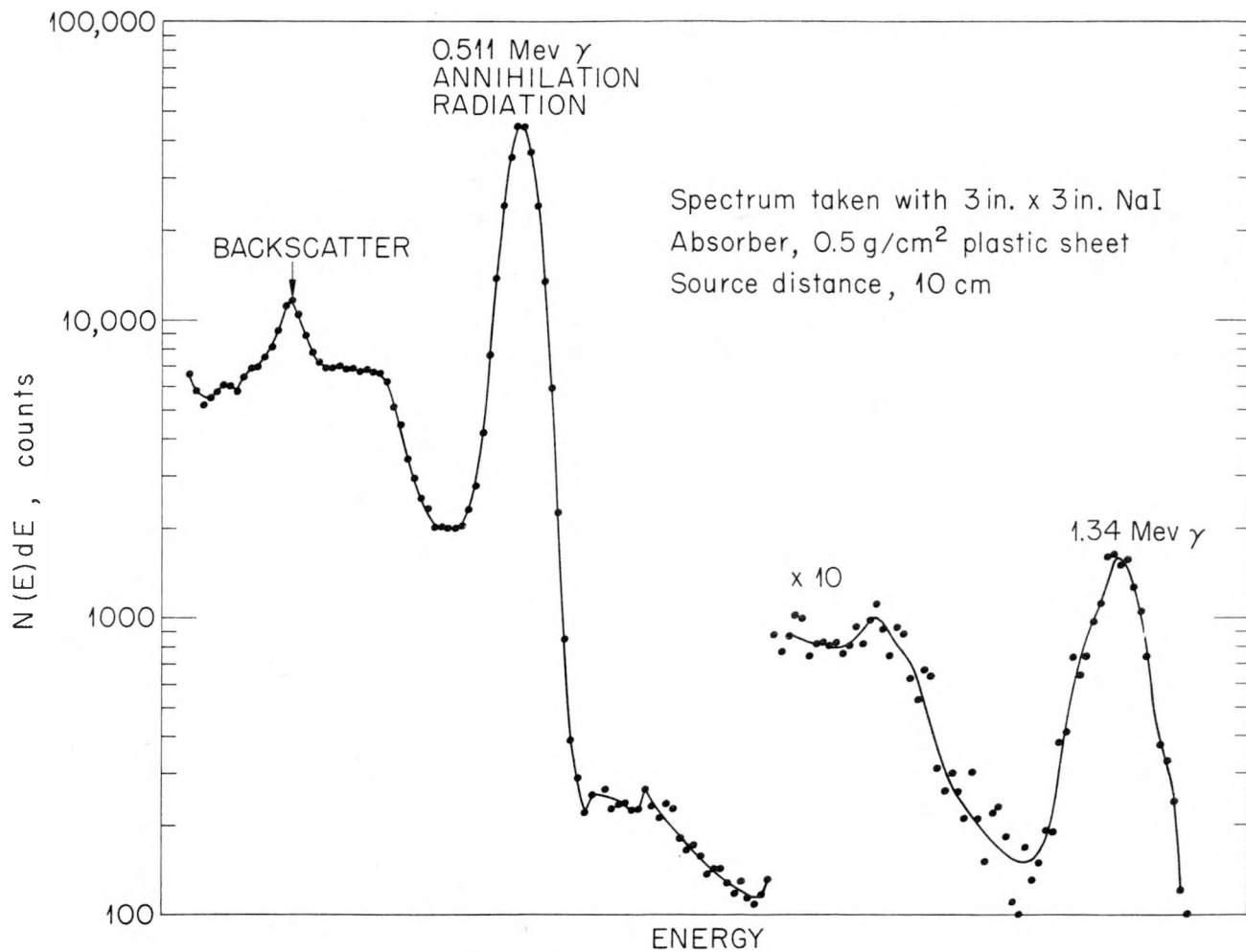
Fig. 4 Gamma-ray spectrum of Cu 64 , half-life = 12.8 hr.
