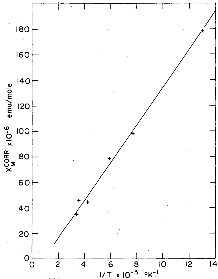
Figure 18-19. \chi^{\text{CORR}} vs 1/T for \text{Os}(\text{SC}_2\text{H}_5)_2
