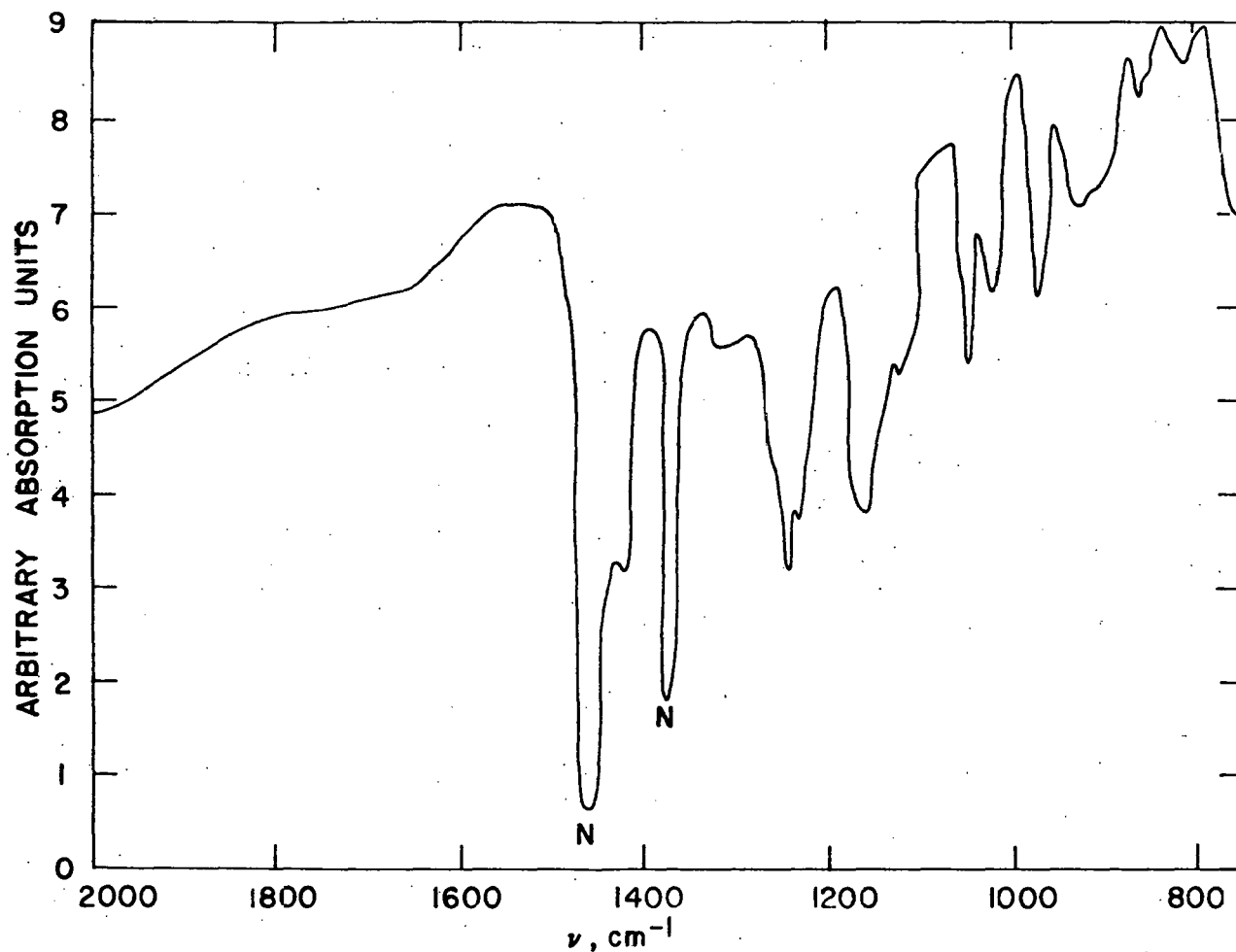
Figure 14a. The infrared spectrum of \text{Os}_2(\text{SC}_2\text{H}_5)_6 from 2000 to 800 \text{cm}^{-1}
