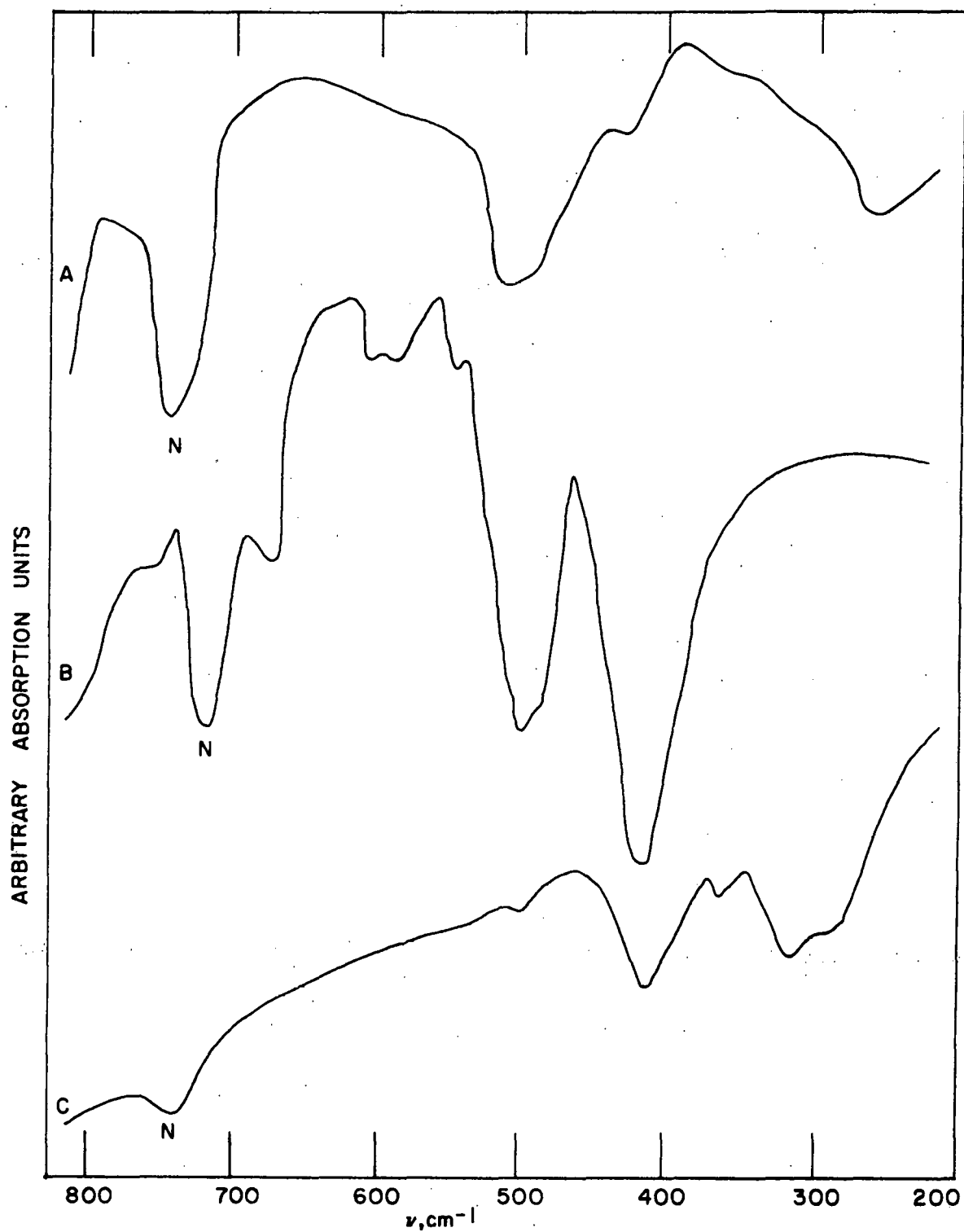
Figure 6. The infrared spectra of [\text{Os}(\text{SCH}_3)_x]_4 (A), [\text{Os}(\text{SC}_2\text{H}_5)_x]_4 (B), and [\text{Os}(\text{SC}_4\text{H}_9)_x]_4 (C) from 800-200 \text{cm}^{-1}
