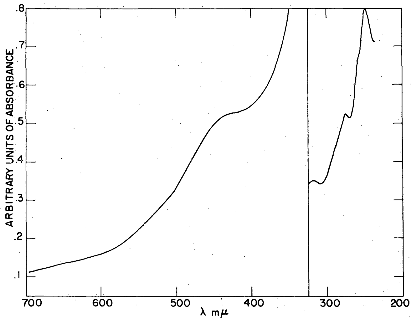
Figure 15. The electronic spectrum of \text{Os}_2(\text{SC}_2\text{H}_5)_6
