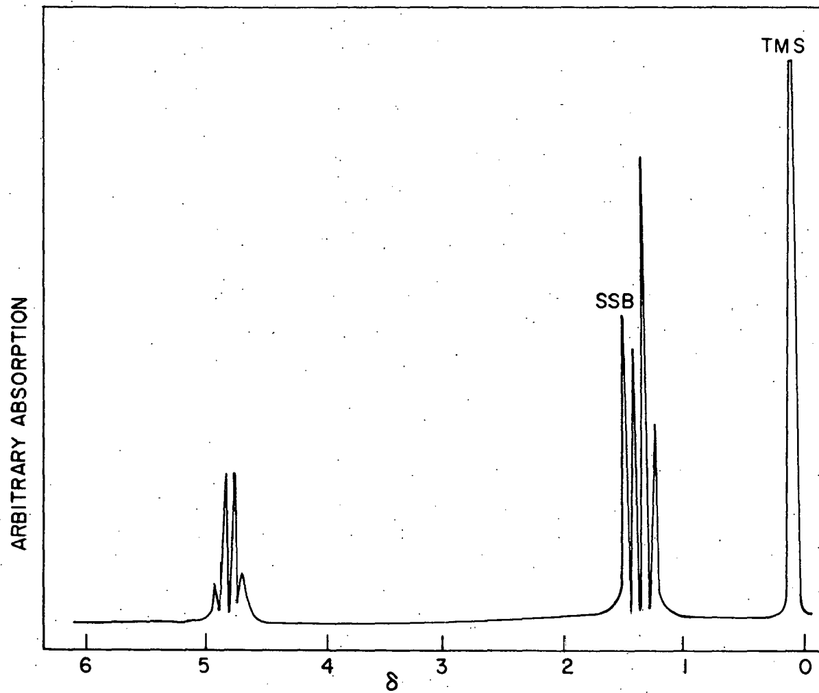
Figure 16. The proton magnetic resonance spectrum of \text{Os}_2(\text{SC}_2\text{H}_5)_6
