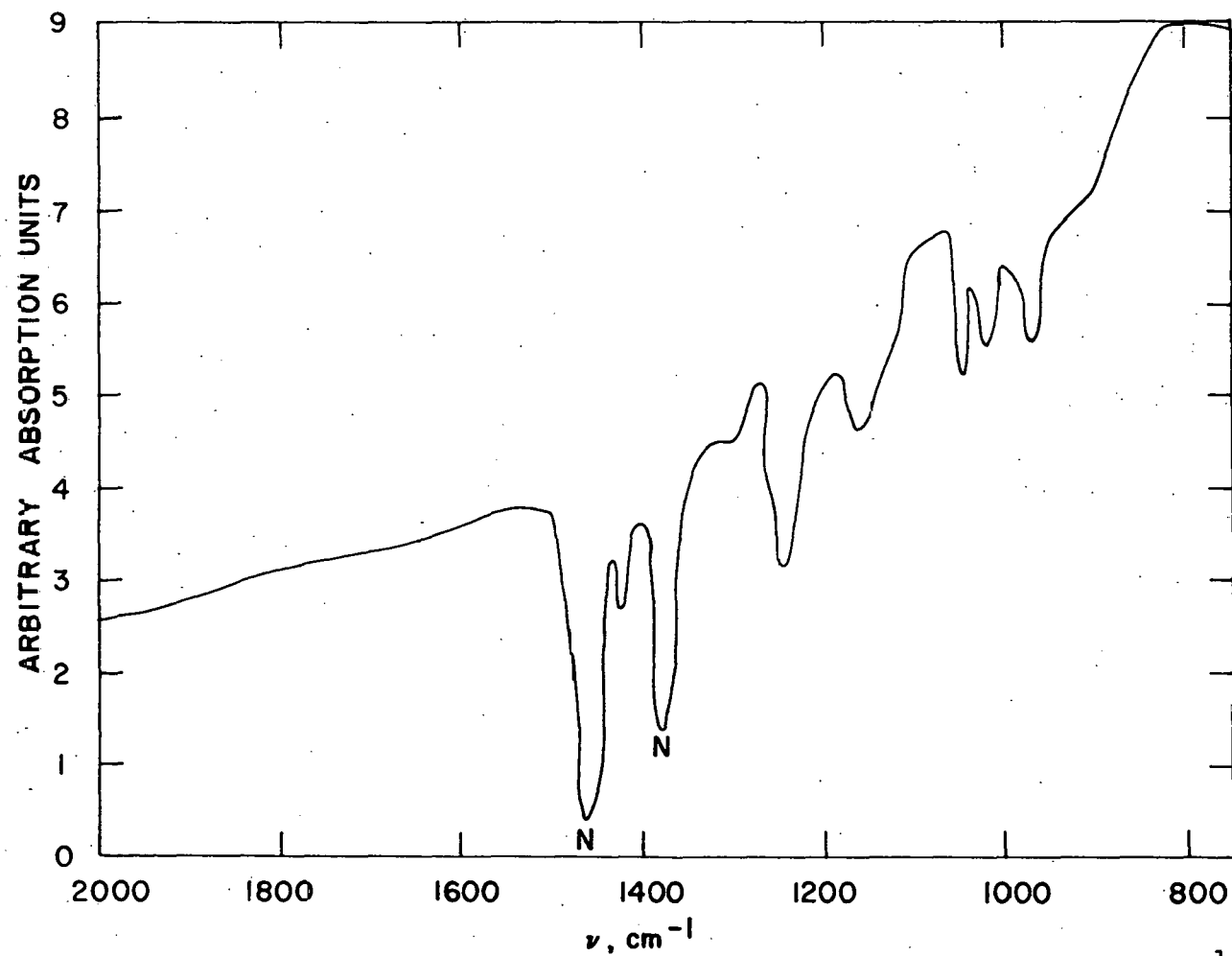
Figure 17a. The infrared spectrum of \text{Os}(\text{SC}_2\text{H}_5)_2 from 2000 to 800 \text{cm}^{-1}
