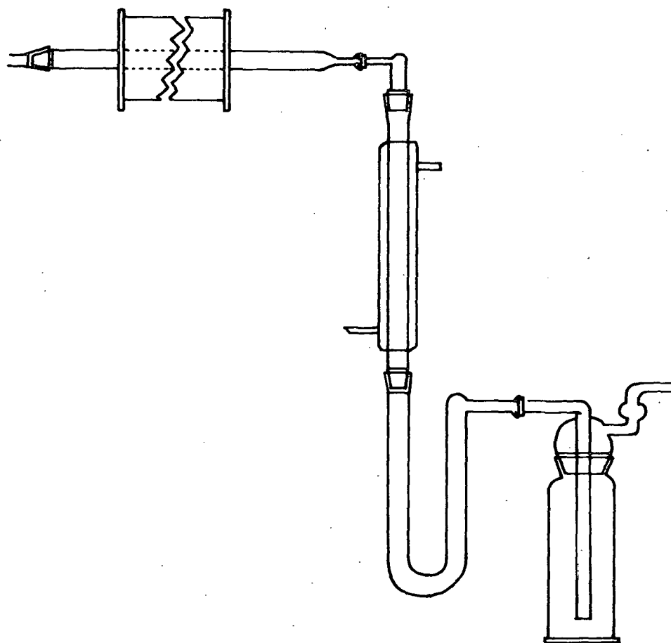
Figure 2. Apparatus for the preparation of osmium tetroxide
