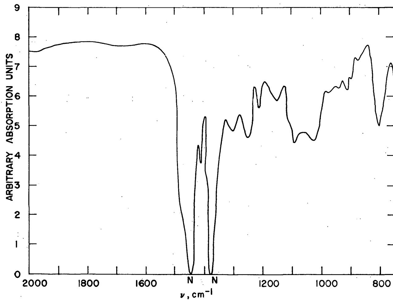
Figure 20a. The infrared spectrum of \text{Os}(\text{SC}_4\text{H}_9)_3 from 2000-800 \text{cm}^{-1}
