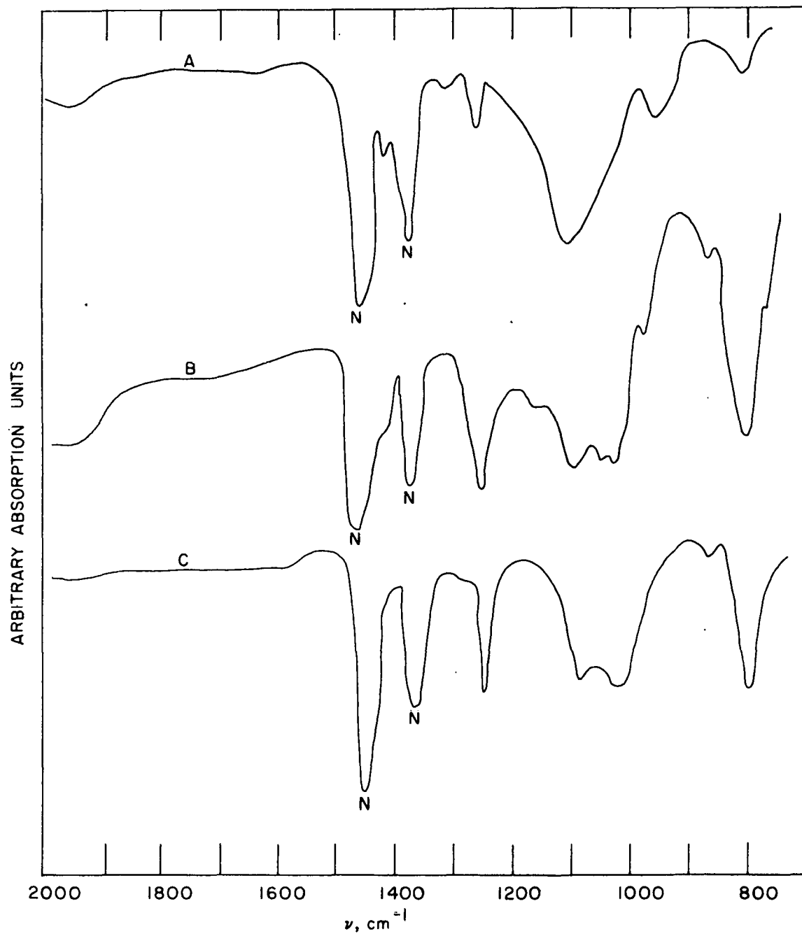
Figure 5. The infrared spectra of [\text{Os}(\text{SCH}_3)_x]_4 (A), [\text{Os}(\text{SC}_2\text{H}_5)_x]_4 (B), and [\text{Os}(\text{SC}_4\text{H}_9)_x]_4 (C) from 2000-800 \text{cm}^{-1}
