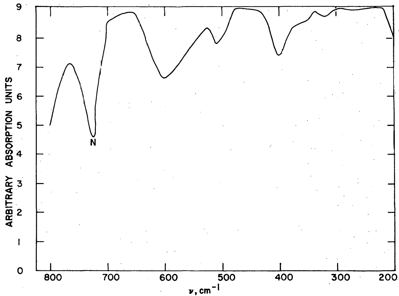
Figure 20b. The infrared spectrum of \text{Os}(\text{SC}_4\text{H}_9)_3 from 800 to 200 \text{cm}^{-1}
