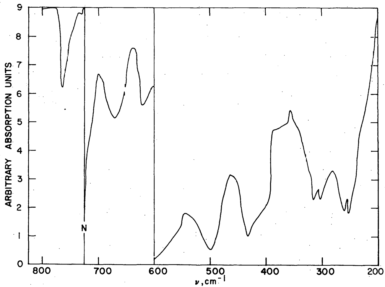
Figure 17b. The infrared spectrum of \text{Os}(\text{SC}_2\text{H}_5)_2 from 800 to 200 \text{cm}^{-1}
