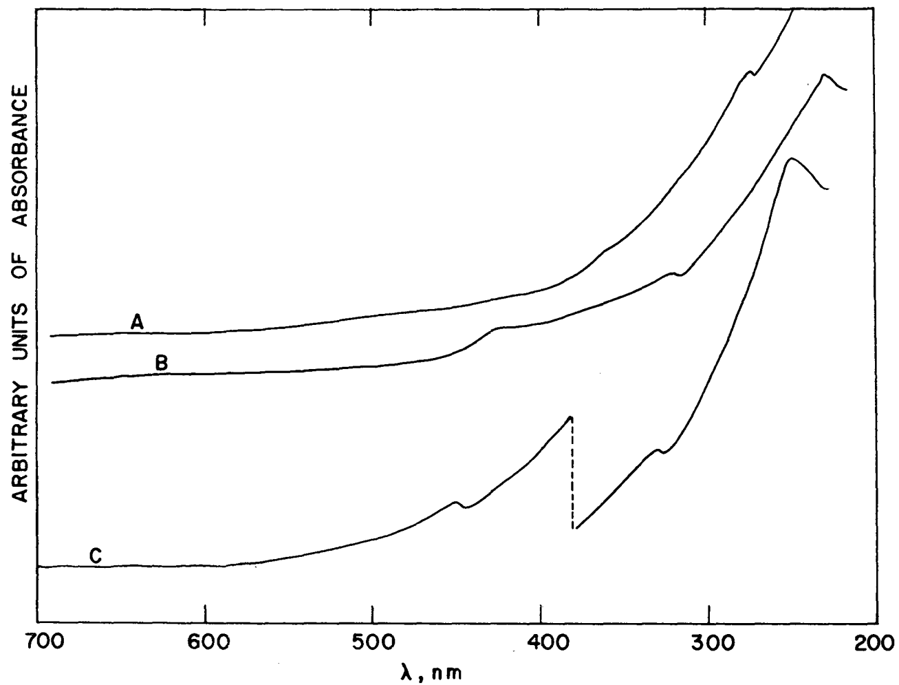
Figure 12. The electronic spectra of [\text{Os}(\text{SCH}_3)_4]_x (A), [\text{Os}(\text{SC}_2\text{H}_5)_4]_x (B), and [\text{Os}(\text{SC}_4\text{H}_9)_4]_x (C)
