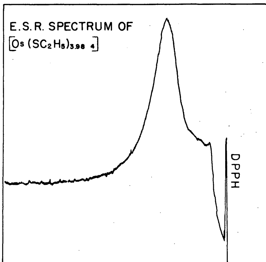
Figure 11. ESR spectrum of [\text{Os}(\text{SC}_2\text{H}_5)_{3.98}]_4
