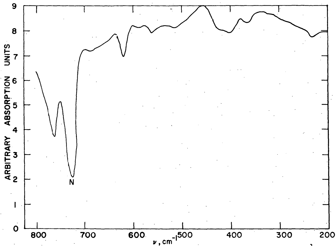
Figure 14b. The infrared spectrum of \text{Os}_2(\text{SC}_2\text{H}_5)_6 from 800 to 200 \text{cm}^{-1}
