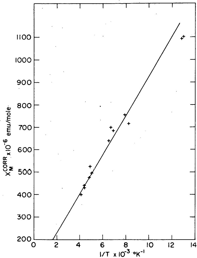
Figure 8. \chi^{\text{CORR}} vs 1/T for [\text{Os}(\text{SC}_2\text{H}_5)_{3.98}]_4
