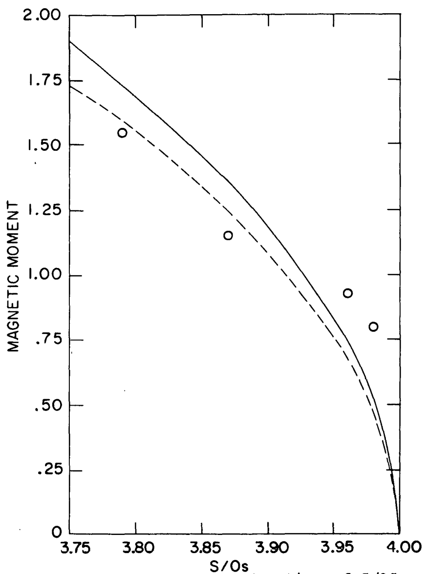
Figure 13. Magnetic moment as a function of S/OS ratio in [\text{Os}(\text{SR}_x)_4] compounds. Solid line represents \mu = 1.9 for [\text{Os}(\text{SR})_{3.75}]_4 ; dashed line represents \mu = 1.73 . Experimental points denoted by O
