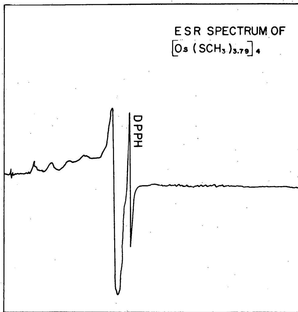
Figure 10. ESR spectrum of [\text{Os}(\text{SCH}_3)_{3.79}]_4
