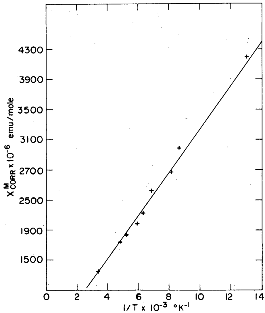
Figure 7. \chi^{\text{CORR}} vs 1/T for [\text{Os}(\text{SCH}_3)_{3.79}]_4
