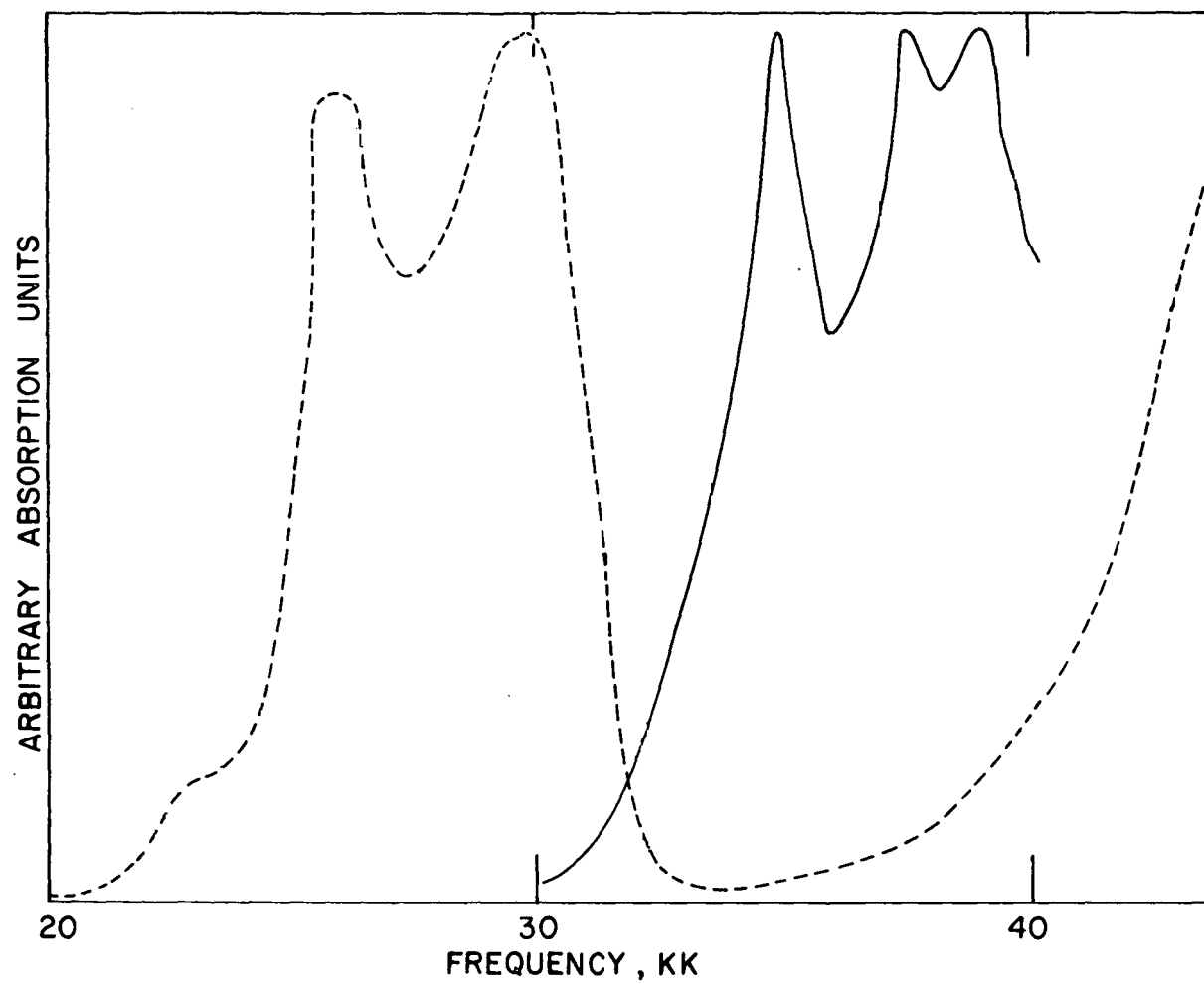
Figure 4. The electronic spectra of \text{OsCl}_6^{2-} (dashed line) and \text{OsCl}_6^{3-} (solid line)
