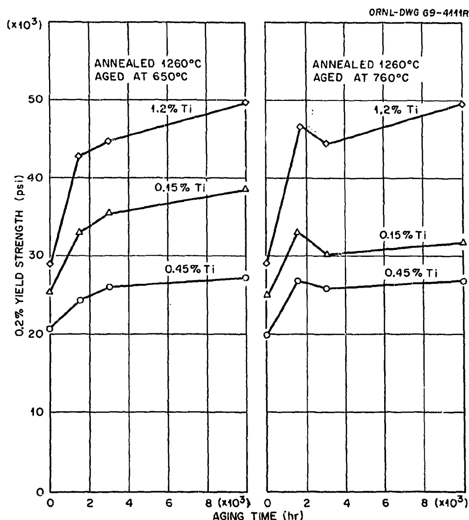
Fig. 6. Yield Strength Changes as a Function of Aging Time and Titanium Content for a 1-hr Solution Anneal at 1260°C.
