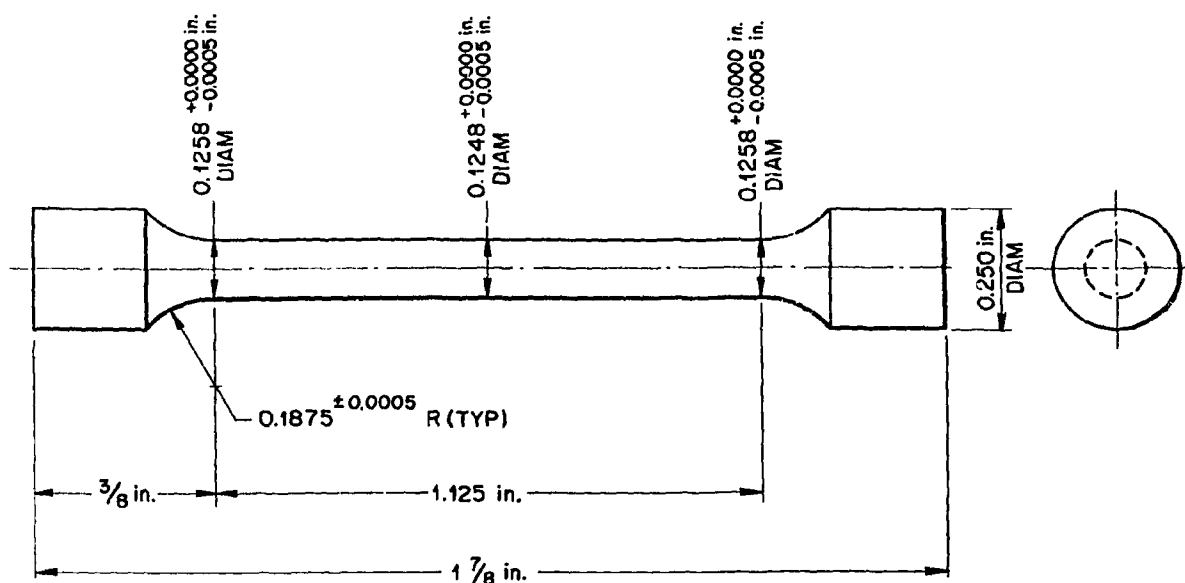
Fig. 1. Mechanical Property Test Specimen.
