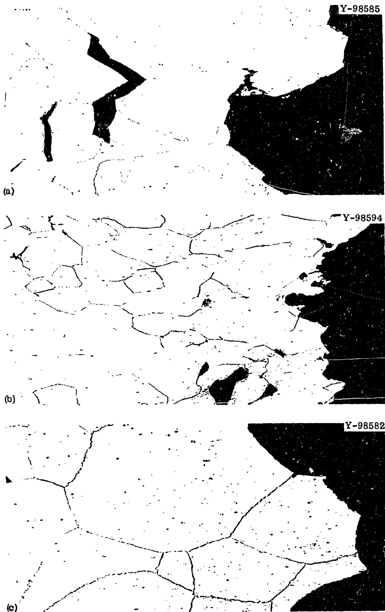
Fig. 17. Creep Fractures for Tests at 650°C and 40,000 psi in Titanium-Modified Hastelloy N for Various Heat Treatments. 100X. (a) 0.15% Ti solution annealed 1 hr at 1260°C and aged 3000 hr at 760°C, (b) 0.45% Ti solution annealed 1 hr at 1177°C and aged 1500 hr at 760°C, and (c) 1.2% Ti solution annealed 1 hr at 1260°C and aged 3000 hr at 650°C. Reduced 18%.
