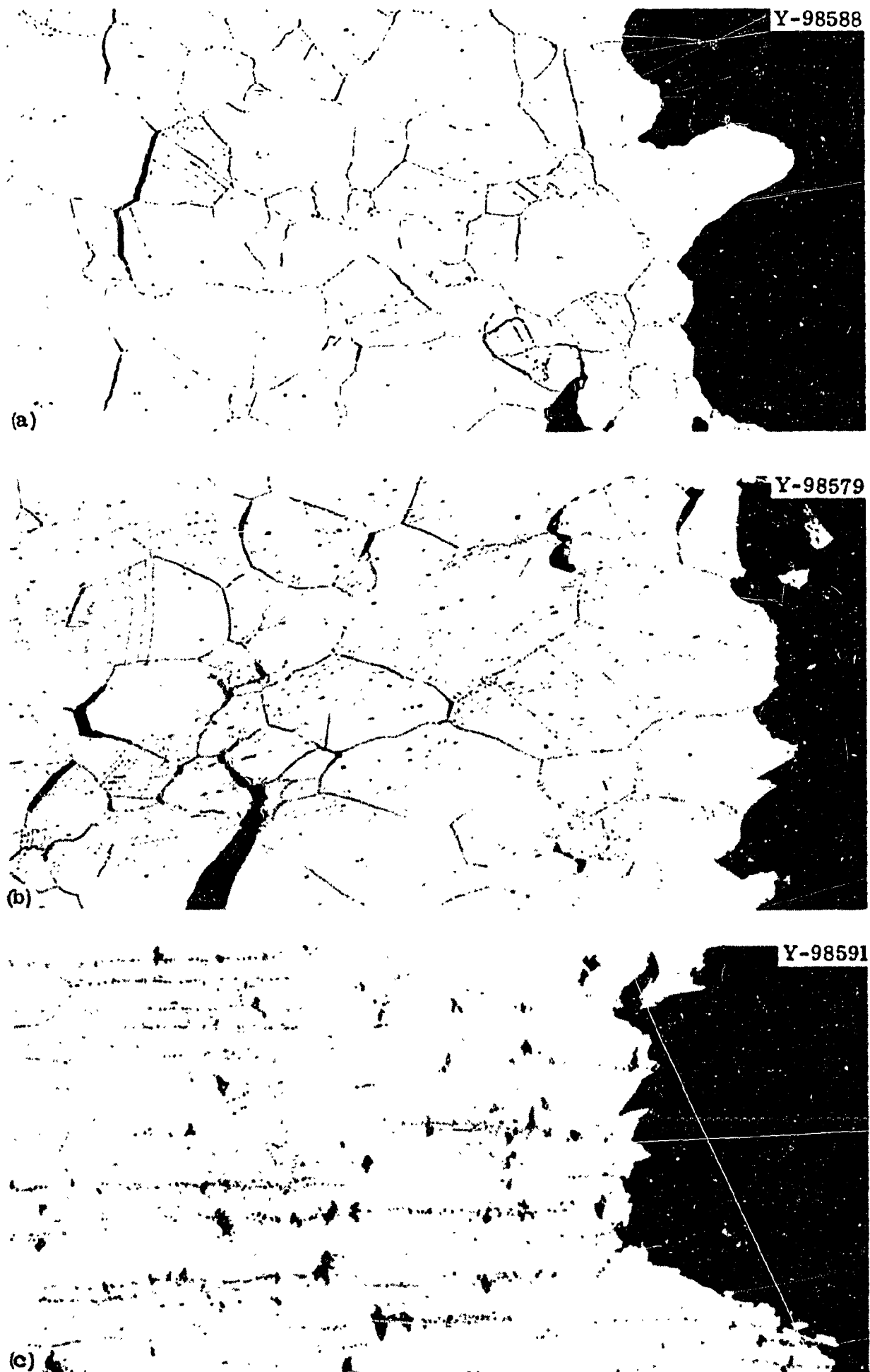
Fig. 16. Creep Fractures at 650°C and 40,000 psi for Heats of Titanium-Modified Hastelloy N After a 1 hr at 1177°C Solution Anneal and 3000 hr Age at 760°C. 100X. (a) 0.15% Ti, (b) 0.45% Ti, and (c) 1.2% Ti. Reduced 18%.
