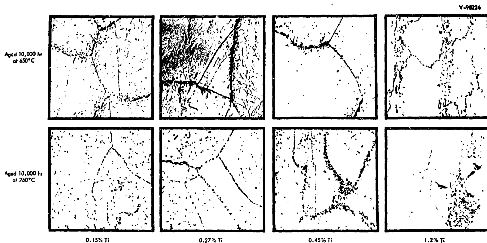
Fig. 13. Microstructures Developed in Ni-12% Mo-7% Cr-0.07% C Alloys Modified with Titanium, Solution Annealed 1 hr at 1177°C, and Aged 10,000 hr. 1000X. Reduced 65%.
