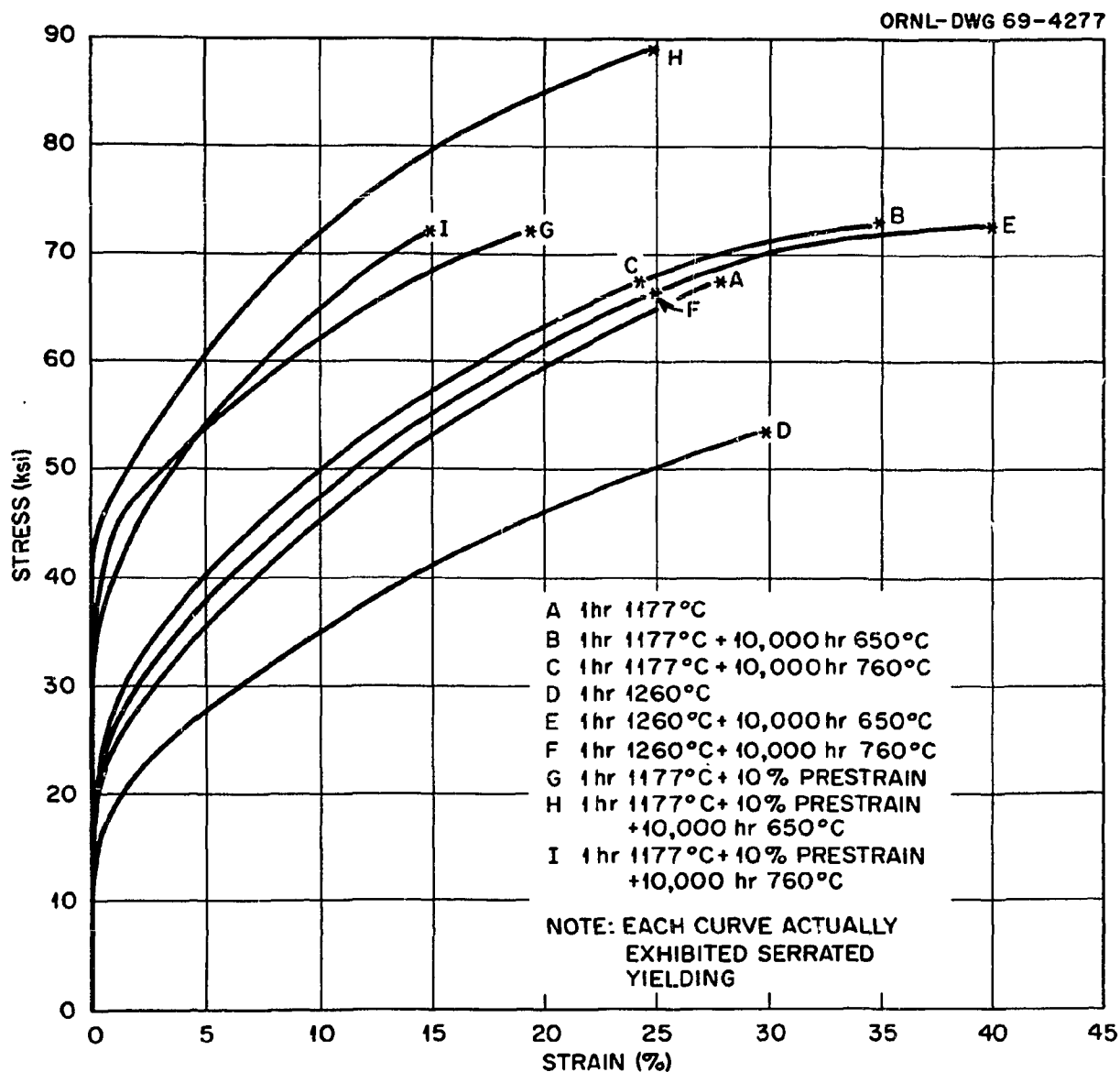
Fig. 7. Stress-Strain Curves for the 0.45% Ti Heat at 650°C for Various Heat Treatments.
