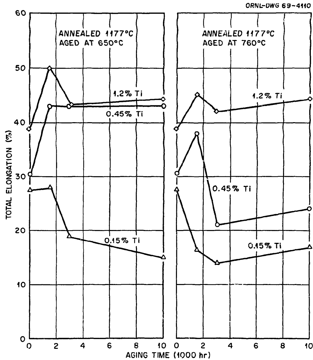
Fig. 3. Effect of Titanium Content and Aging Time on the Tensile Ductility at 650°C after a 1-hr Solution Anneal at 1177°C.
