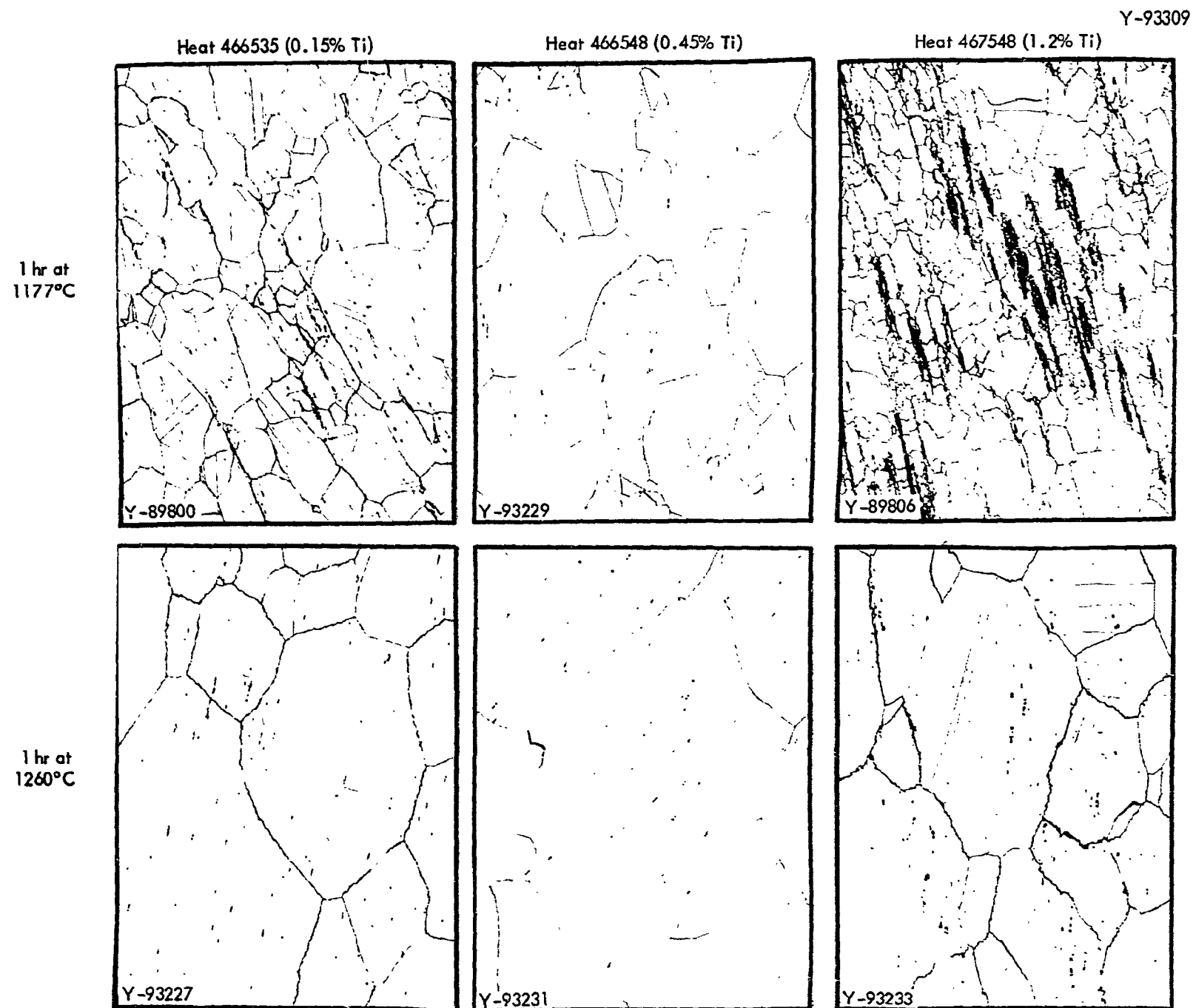
Fig. 12. Microstructures of Titanium-Modified Alloys in the Solution-Annealed Condition. 100X. Reduced 38%.
