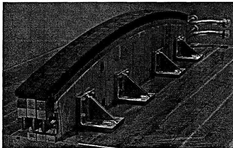
Figure 3. One-quarter-width mock-up of the vertical target. The length is 1.3 m, and the width is about 10 cm. The armor tile is unidirectional CFCs brazed on an OFHC Cu heat sink with a silver braze. The cooling tube is an OFHC Cu swirl tube.
