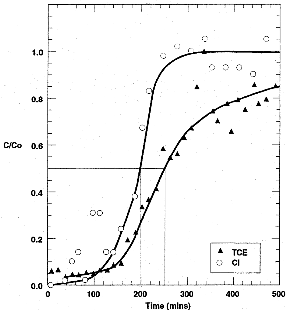
Figure 2. TCE and chloride breakthrough curves from the first TCE sorption experiment. Application of equation 1 yields an R of 1.34 and a K_d of 0.05 ml/g.
