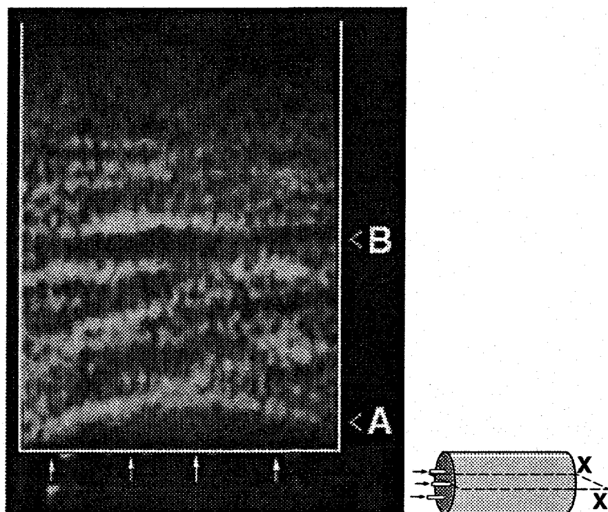
Figure 1. This MRI image was taken of the water saturated column before the introduction of the tracer. Note the prominent light-colored coarser-grained feature (A) at the entrance of the column, and the dark-colored finer-grained feature (B) about 3 cm into the column. Six cm of the sand are shown in this image.
