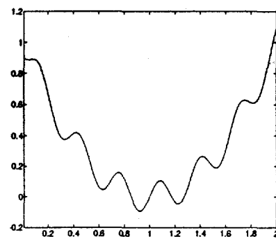
Figure 2: A class of gradually deformed functions
