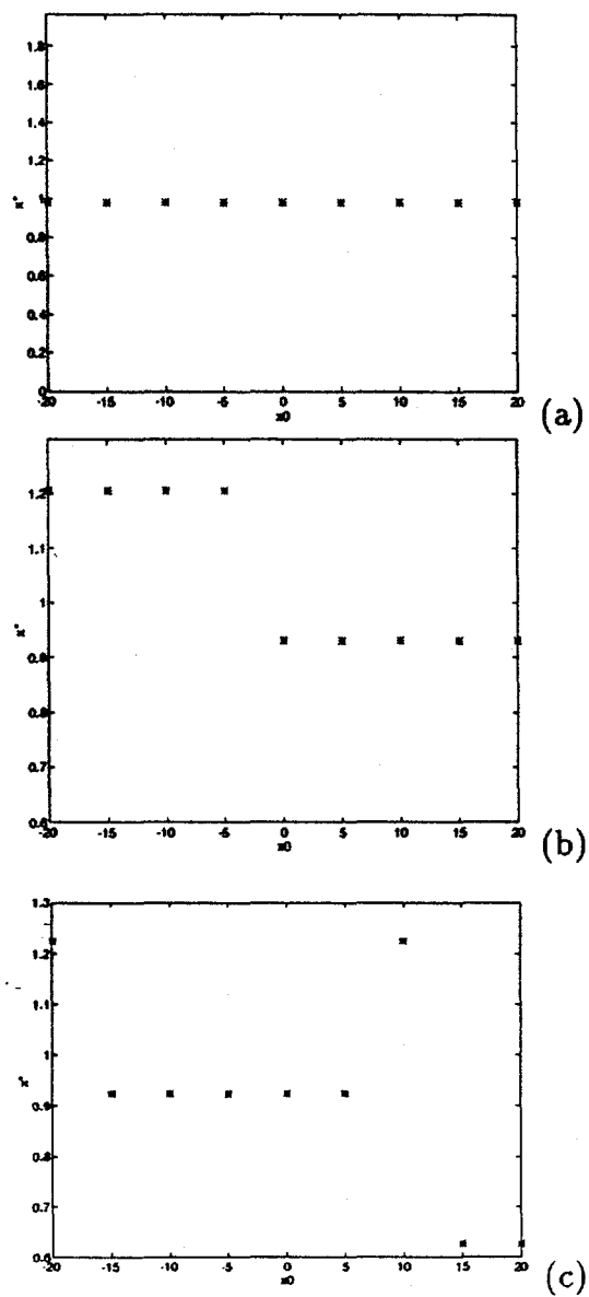
Figure 3: The solutions for the functions in Figure 2 obtained by the quasi-Newton method with different initial guesses
