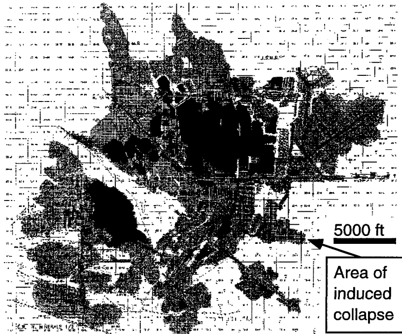
Figure 2. A plan view of the extent of underground workings at the White Pine Mine. Hachured areas indicate room and pillar mined areas while black indicates failed pillar areas in the mine. The failed area outlined in the lower left quadrant on the hanging wall of the White Pine Fault was a catastrophic event which generated regional signals in January of 1989. All other failed areas have experienced slow failure which does not generate large seismic events.
