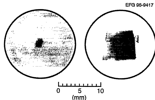
Figure 1. Photographs of small deuterium pellet (left) from centrifuge injector and large tritium pellet (right) from TPOP-II repeating pneumatic injector.
