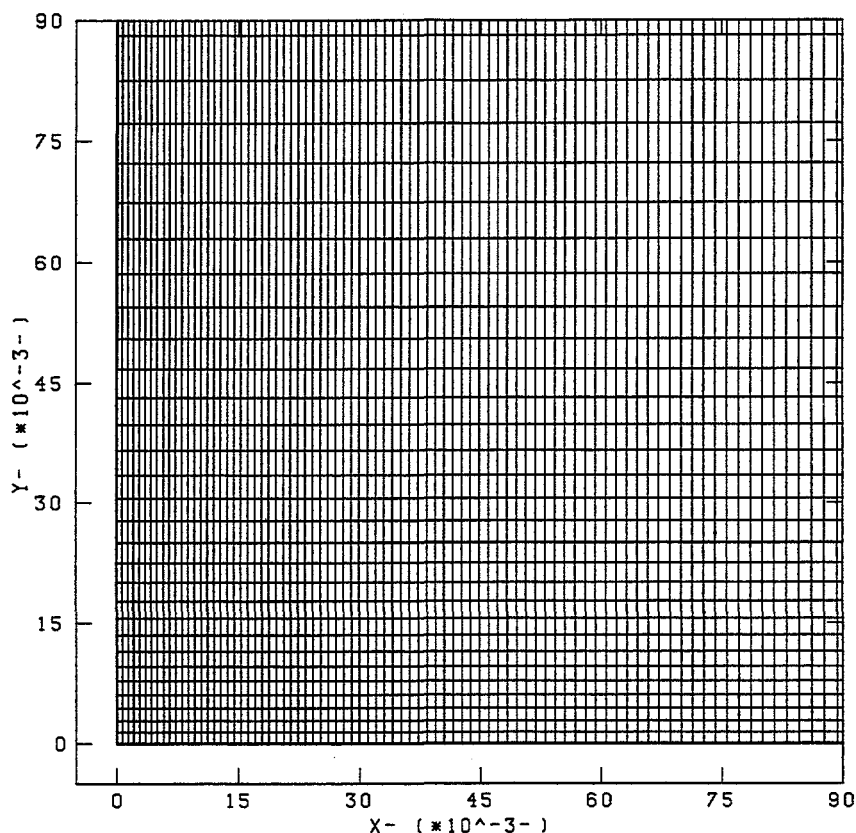
Figure C.5. Expanding mesh of the entrance region for developing flow between parallel plates.
