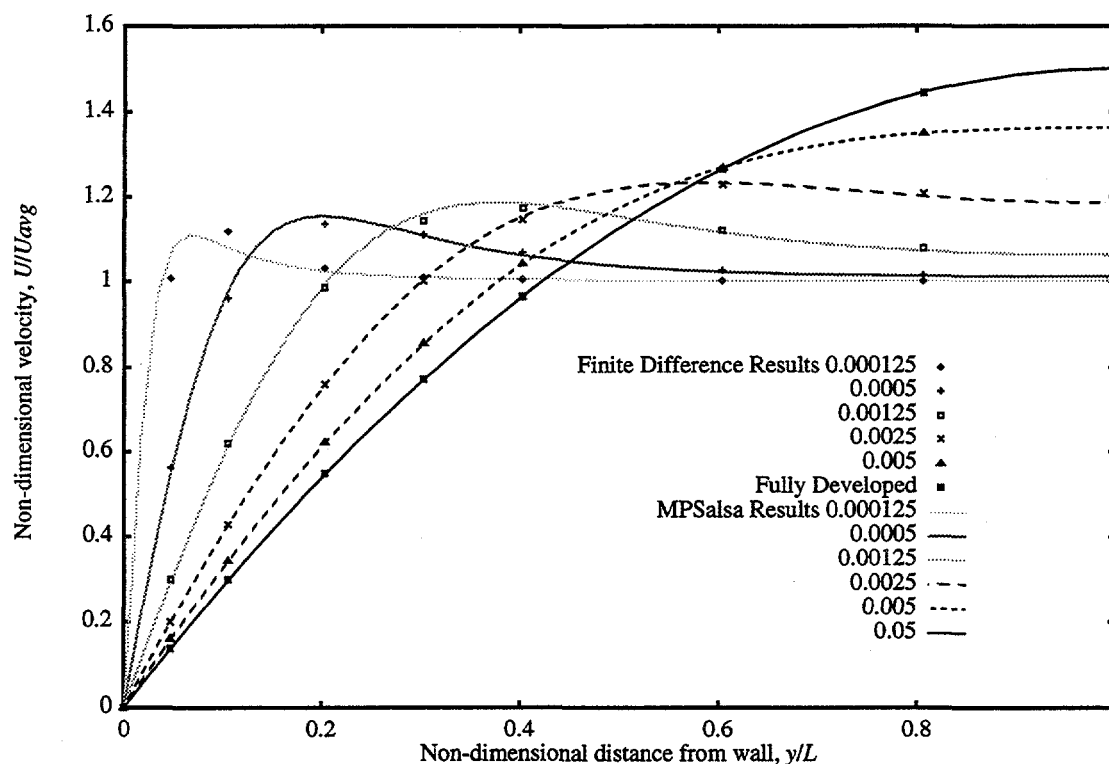
Figure C.7. Developing velocity profiles for flow entering parallel plates for a variety of non-dimensional lengths down the channel, as the flow transitions from plug flow to a parabolic profile.
