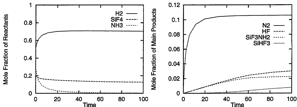
Figure B.8. Evolution in time of mole fractions of major species in the Si 3 N 4 Equilibrium problem. The first plot shows the three reactants, while the second shows the major products of the reactions. Since the pseudo time integration scheme was used, these histories are not time accurate.
