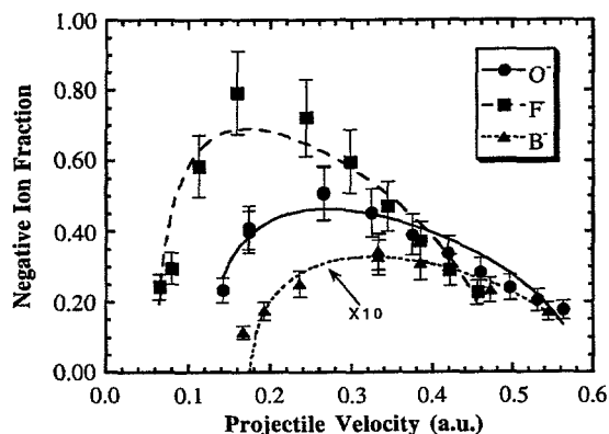
Fig.3 Projectile velocity dependence of the scattered 1^- fractions for multicharged F, O, and B projectiles grazingly incident on LiF(100). The lines are fitted curves based on Eq .2
