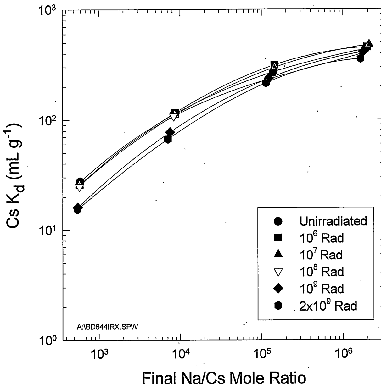
Figure 3.2. Cesium Batch Distribution Ratio as a Function of Na/Cs Ratio for Samples of the SuperLig® 644/WWL Web Irradiated in 0.5 M \text{HNO}_3
