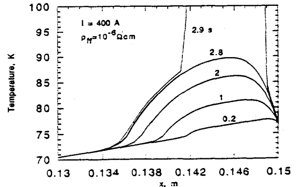
Fig. 5. Temperature distributions of BSCCO-2212 lead at different times for \rho_{ff} = 10^{-6} \Omega\text{-cm} and operating current of 400 A.
