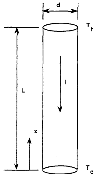
Fig. 1. Schematic diagram of current lead geometry.
