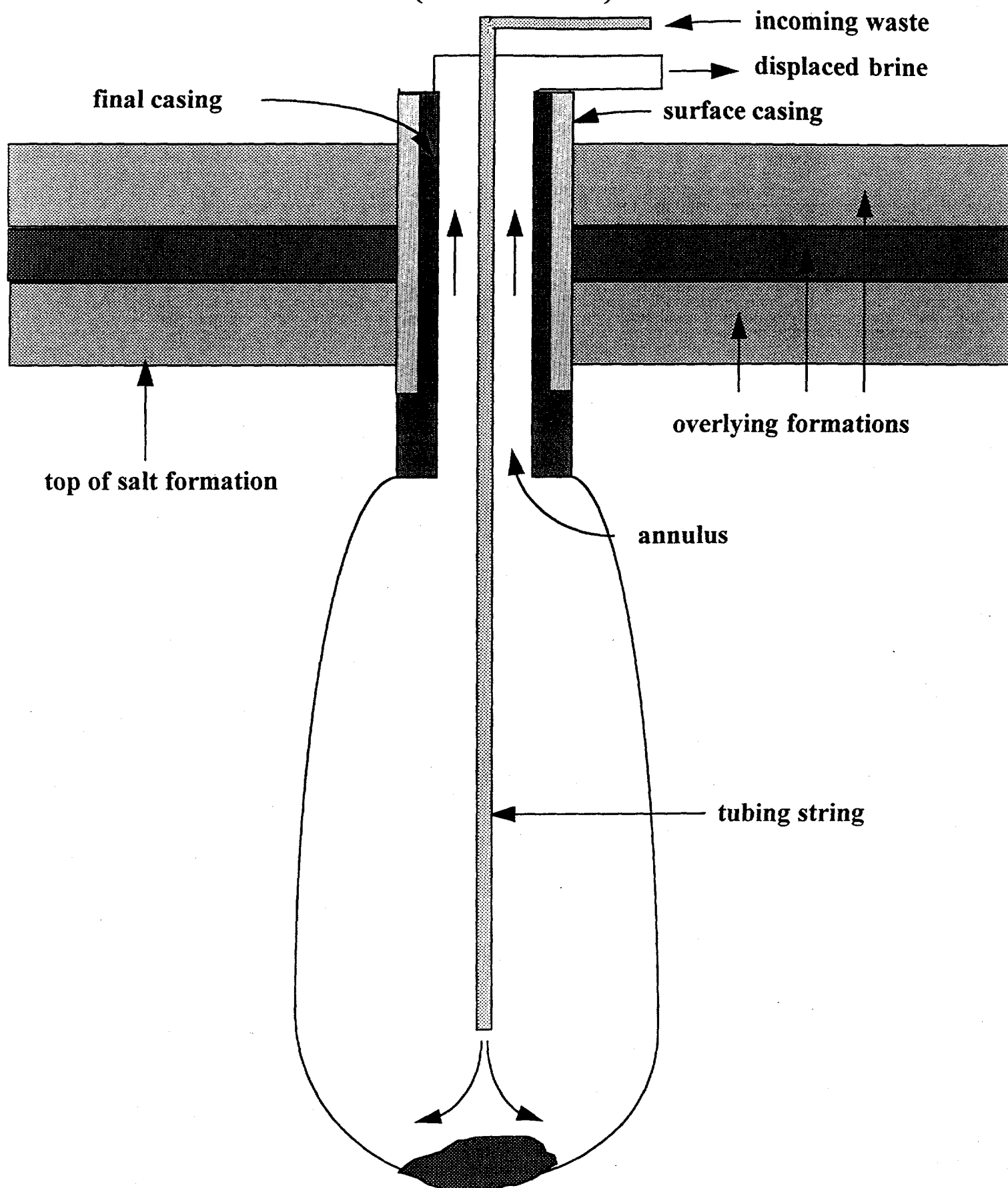
Figure 2 - Idealized Cavern in a Salt Dome Formation (not to scale)
