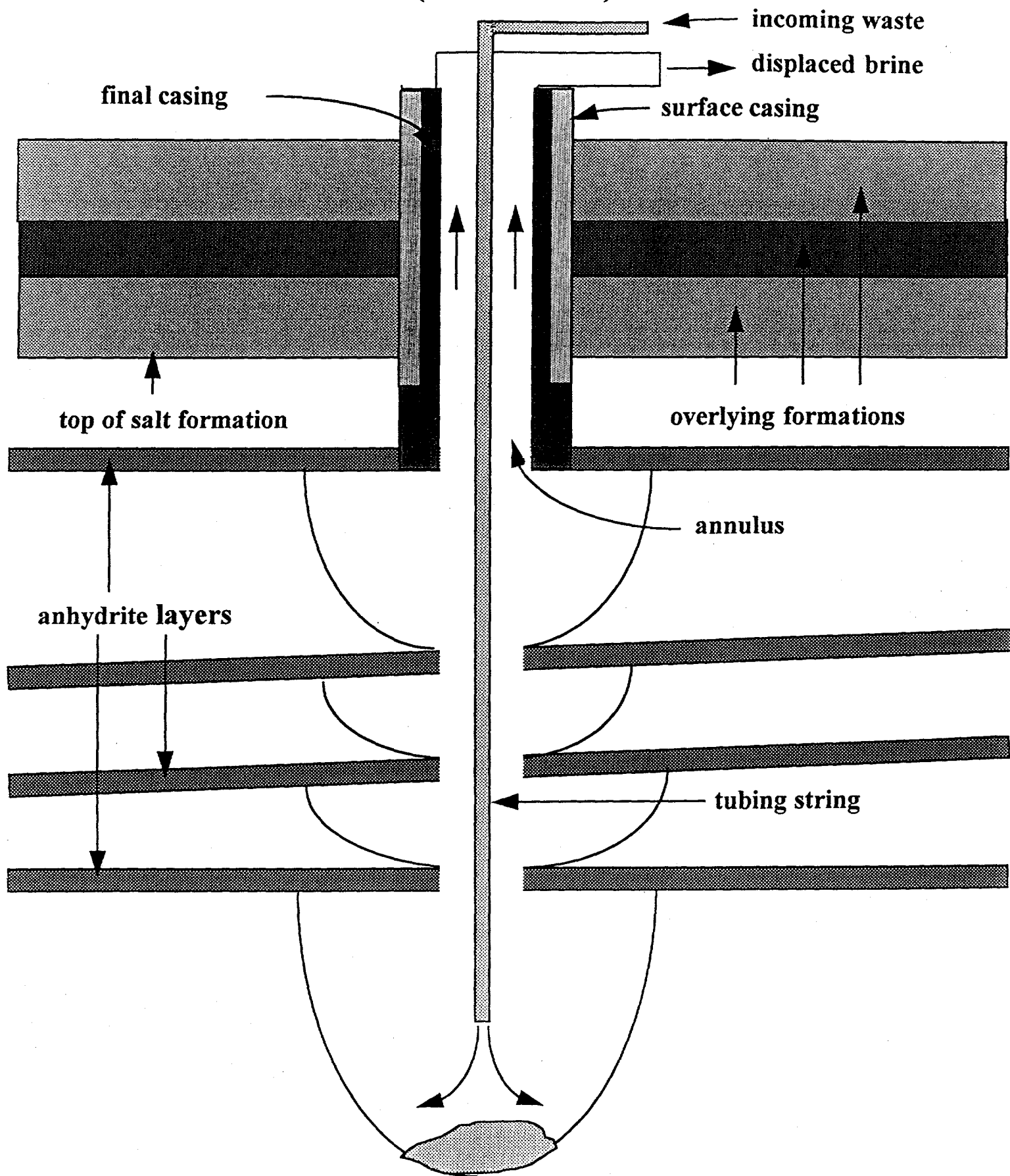
Figure 3 - Idealized Cavern in a Bedded Salt Formation (not to scale)
