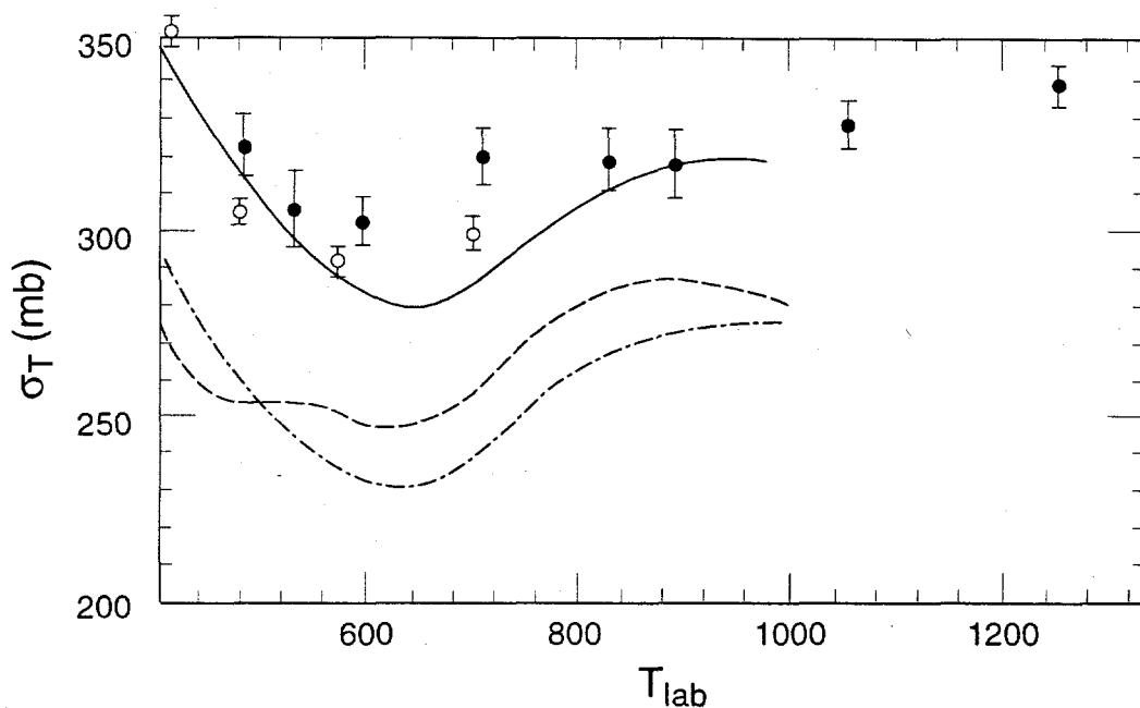
Fig. 1. Total cross section for \pi on ^{12}\text{C} . Data are from Refs. 15 and 16, and the calculations are described in the text.
