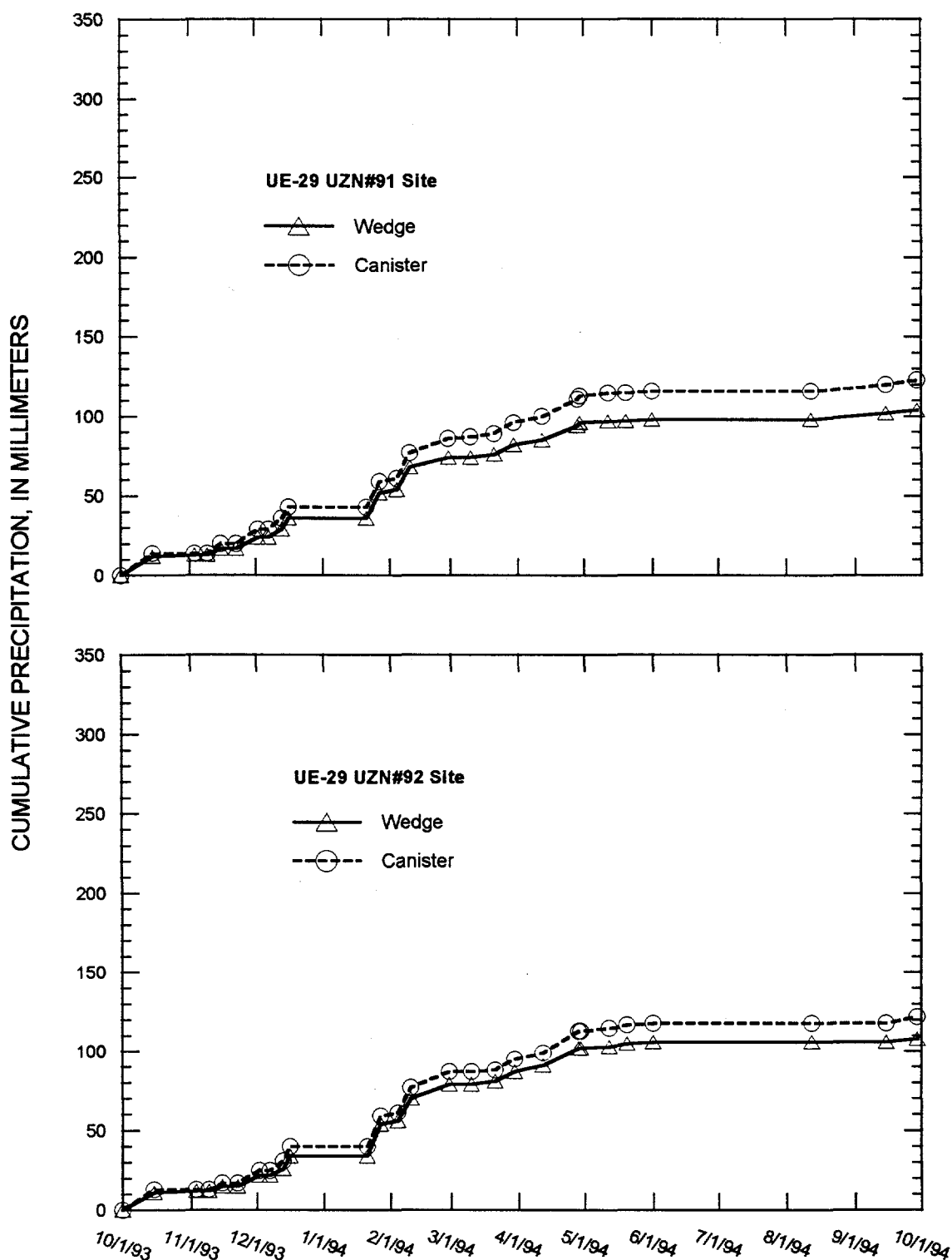
Figure 3. Cumulative precipitation at UE-29 UZN#91 and UE-29 UZN#92 sites in the Yucca Mountain area, Nevada, during water year 1994.
