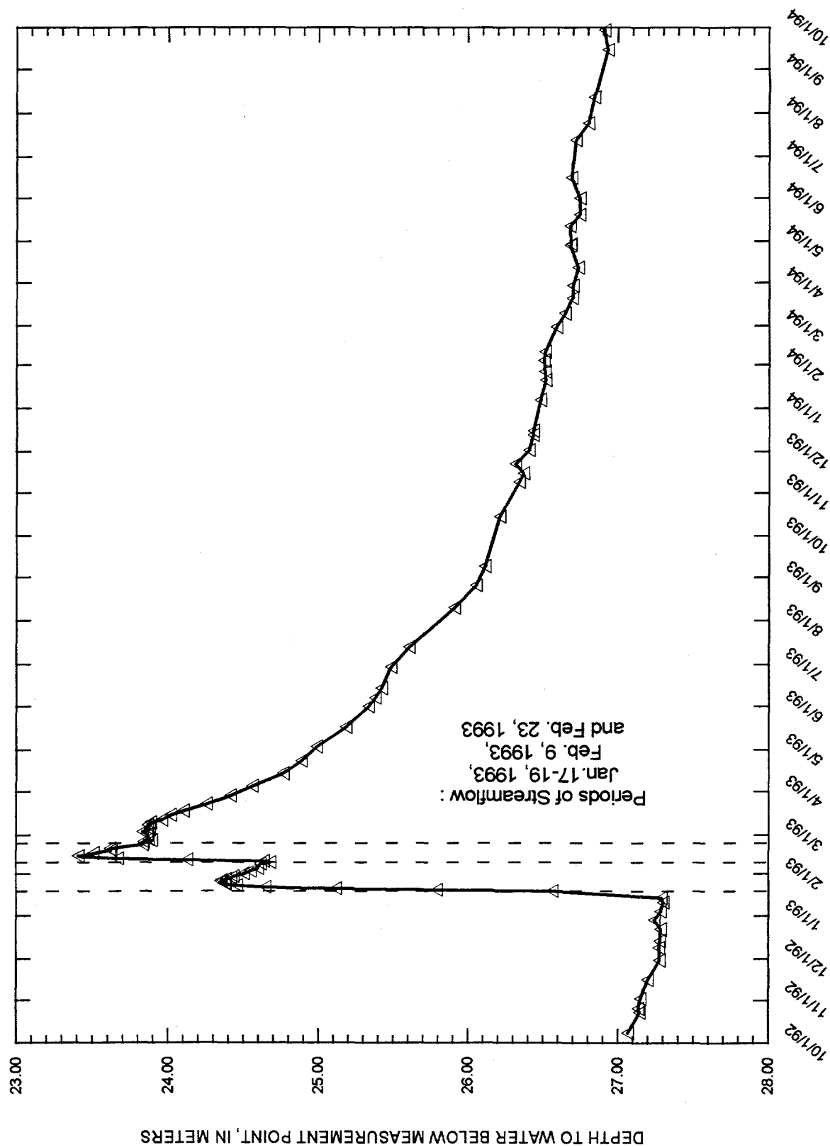
Figure 8. Depth-to-water measurements in UE-29 a#1 in the Yucca Mountain area, Nevada.
