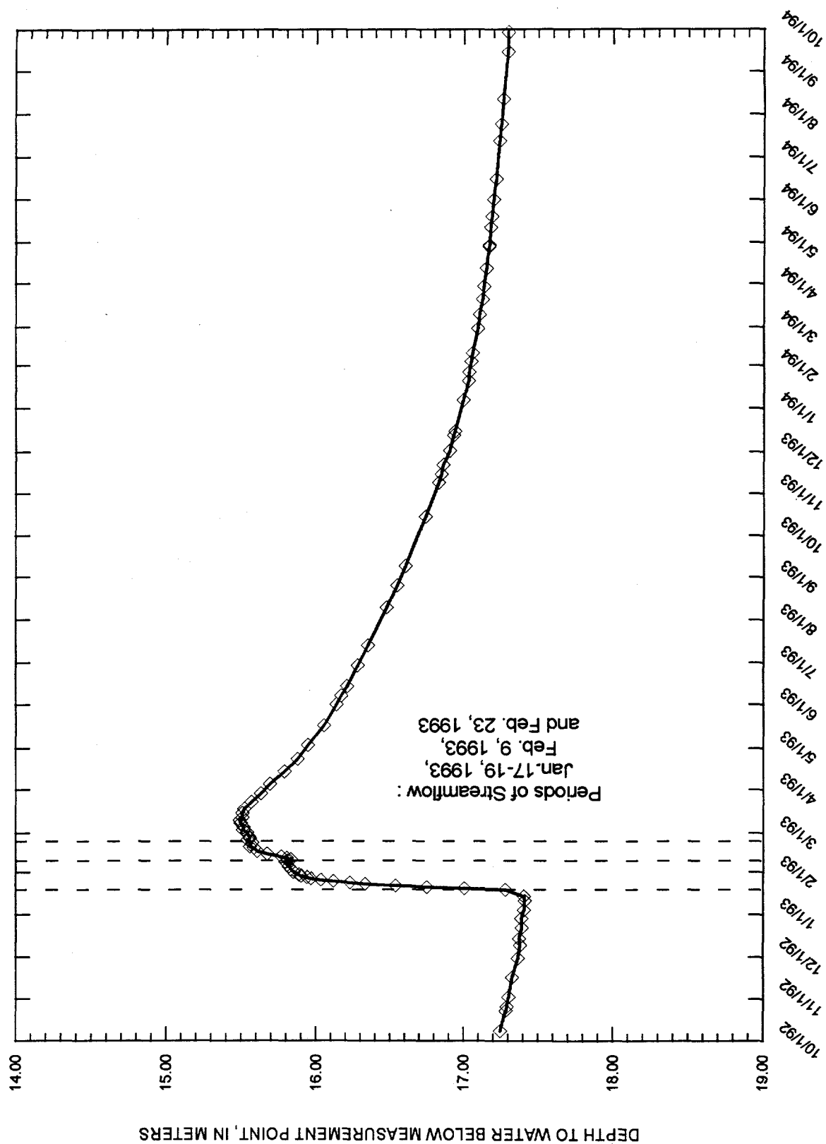
Figure 10. Depth-to-water measurements in UE-29 UZN#91 in the Yucca Mountain area, Nevada.
