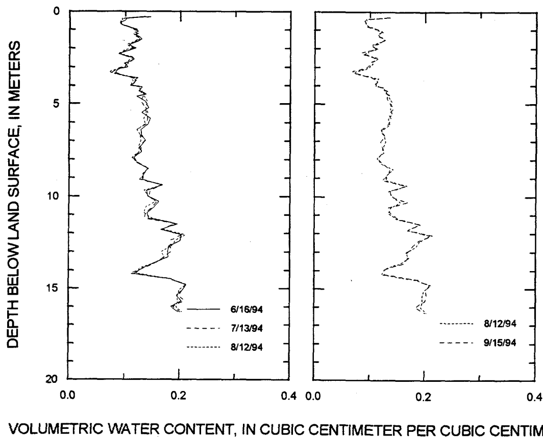
Figure 6. Volumetric water-content profiles for UE-29 UZN#91 in the Yucca Mountain area, Nevada--Continued.
