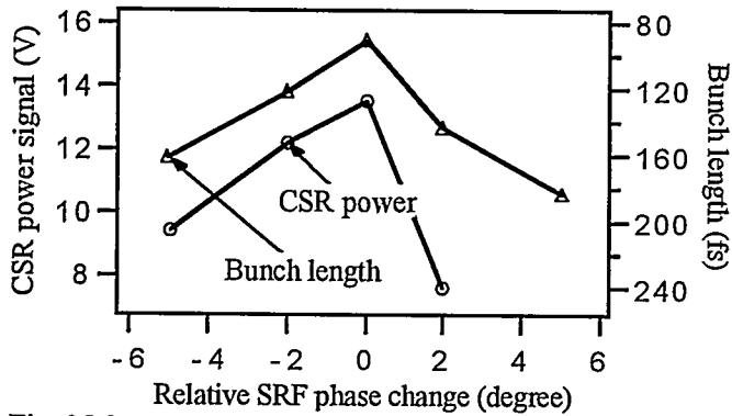
Fig. 9 Measurement results of CSR power and bunch lengths versus relative SRF phase changes. As expected, the shortest bunch length corresponds to the highest CSR power signal.
