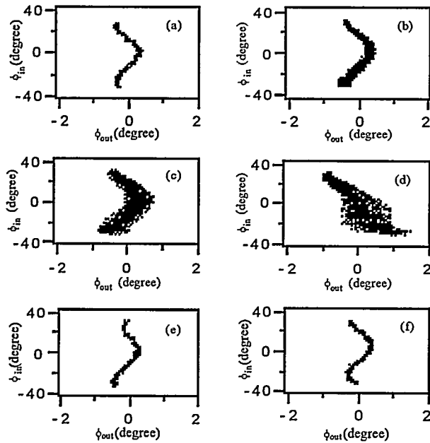
Fig. 3 Plots of phase transfer functions, a relation between modulating phase (input phase) and detected phase (output phase): (a) is measured phase pattern optimized at the first pickup cavity; (b) is simulation result with the initial energy spread and space charge off; (c) is simulation with a significant initial energy spread turned on; (d) is simulation with both energy spread and space charge turned on; (e) is measurement with 0.4 degree phase change of the capture cavity; (f) is measurement with 2 degree of chopper gang phase change.
