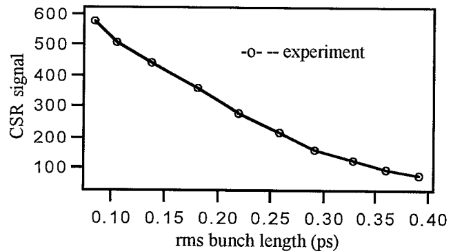
Fig. 8 Experiment result of CSR power versus rms bunch
