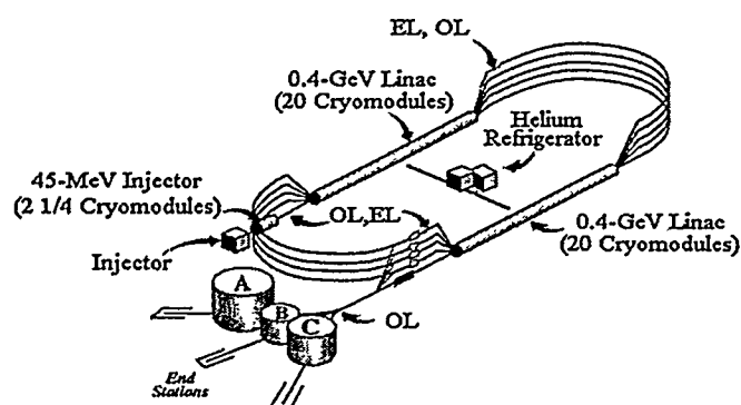
Fig. 2 Energy (EL) and Orbit (OL) locations
