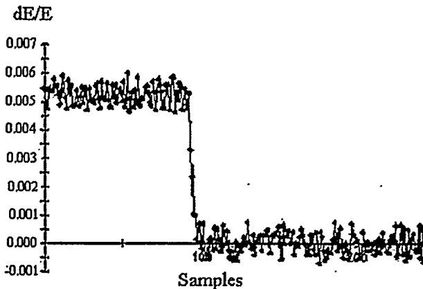
Fig. 3 Injector Energy lock- Effect of closing the loop (E = 45 MeV)
