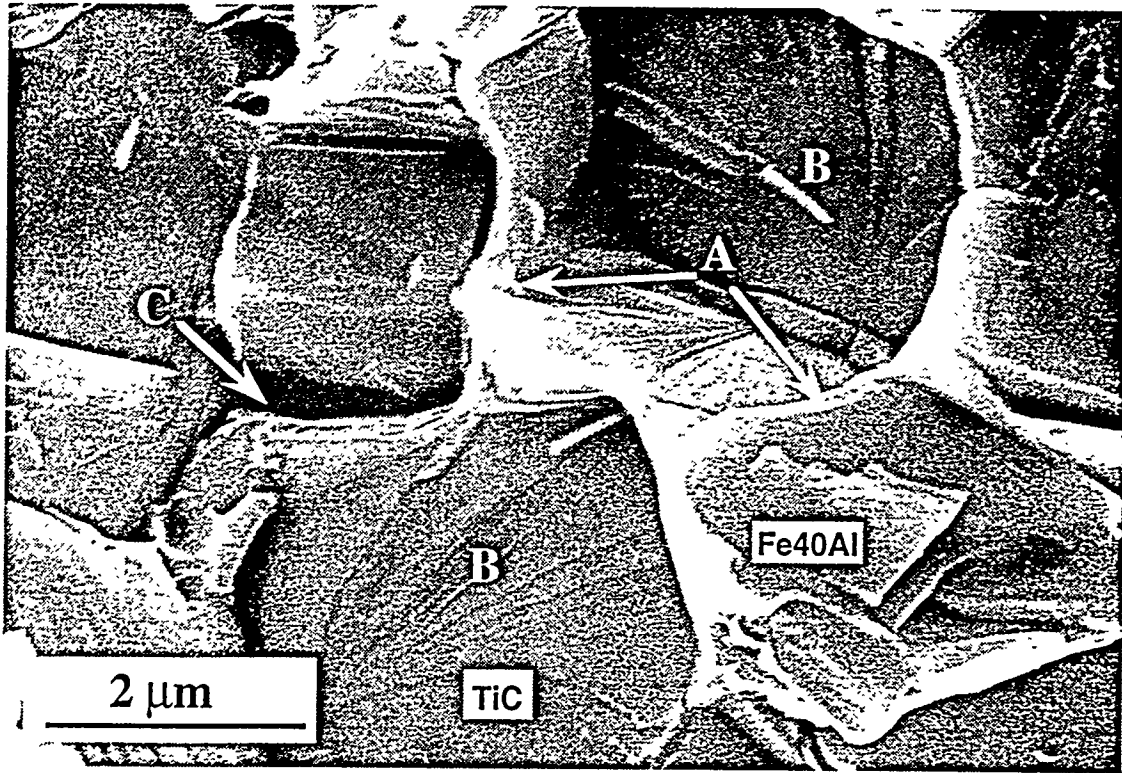
Fig. 2: Fracture surface of a Fe40Al-TiC composite with 30 vol % intermetallic phase
