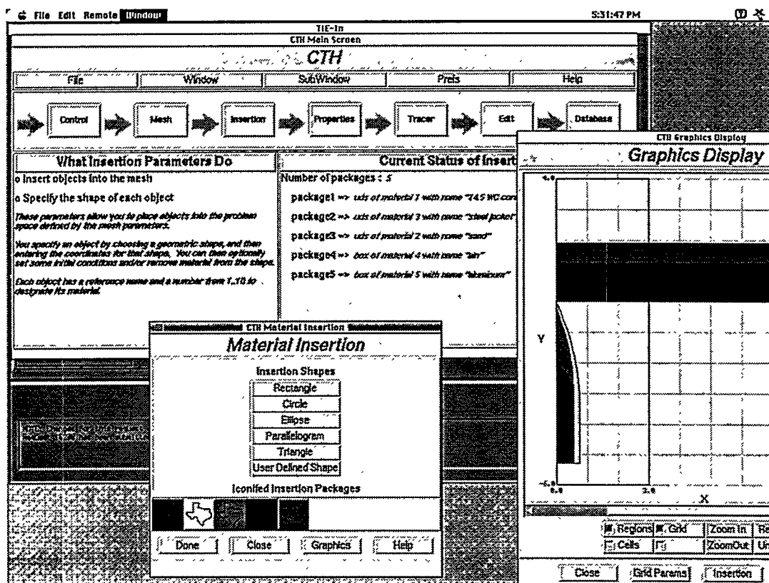
Figure 5. This example from the CTH Hydrocode application shows how the intelligent user interface can guide the user through the process of defining a ballistics penetration problem.
