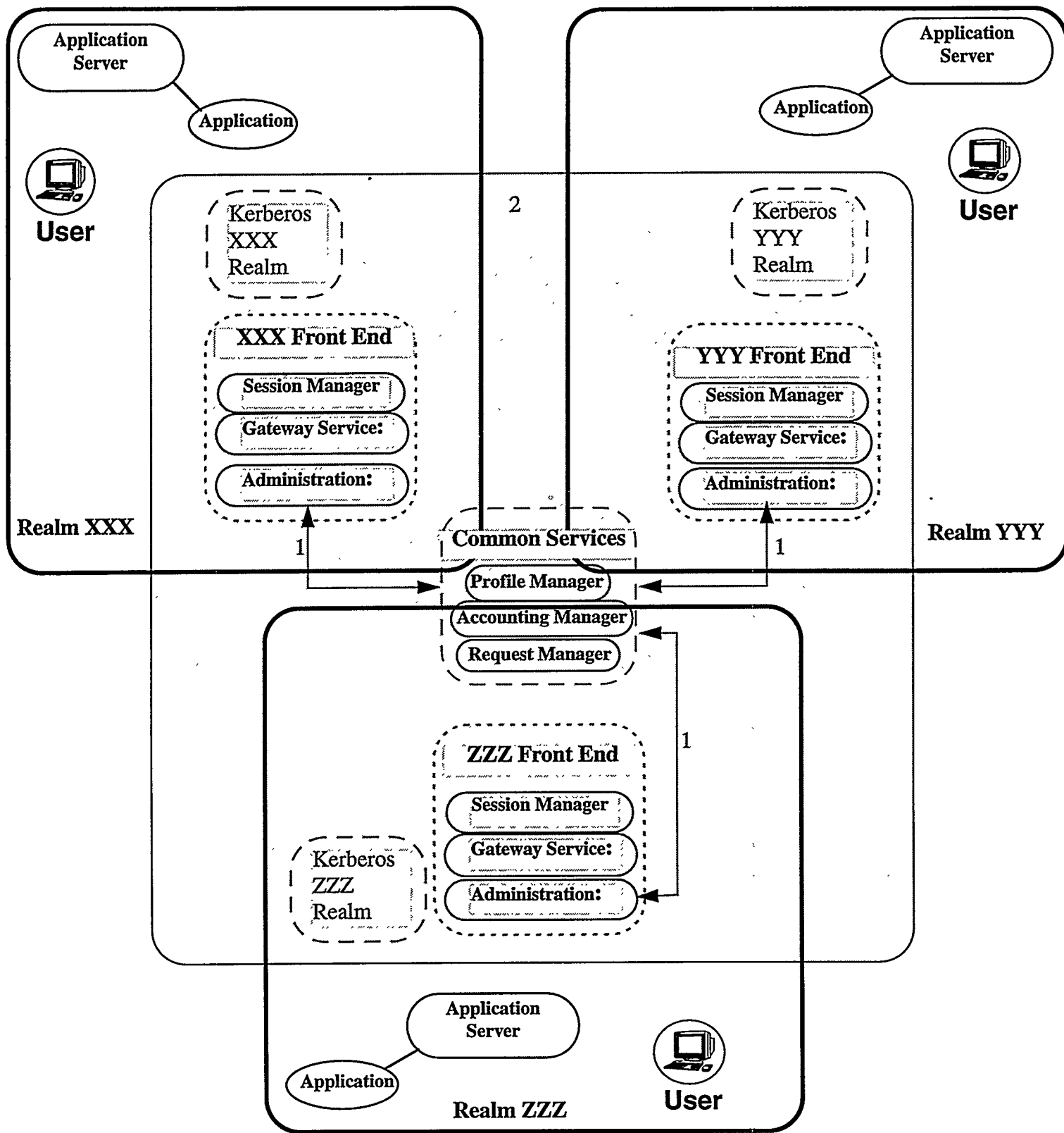
Figure 3. Schematic diagram of TIE-In Multiple Organizational Realms.
