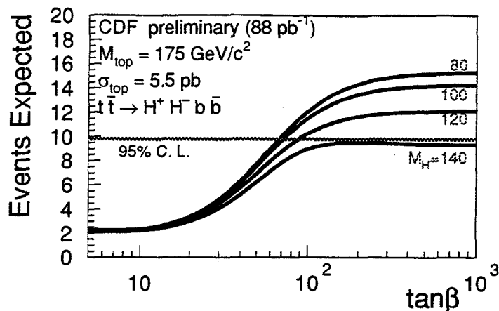
Figure 1: Expected number of charged Higgs events as a function of \tan\beta .
