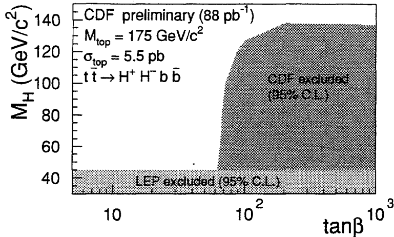
Figure 2: Excluded region in M_H vs. \tan\beta plane.
