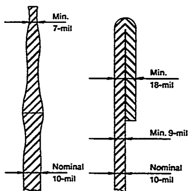
Munters DUBLfold® edges vary between 18 and 22 mil in thickness, while other processes leave edges as thin as 7 mil.
