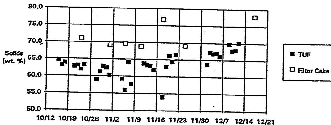
Miami Fort Pilot Plant Phase 3 Solids Settling & Filtration Data
