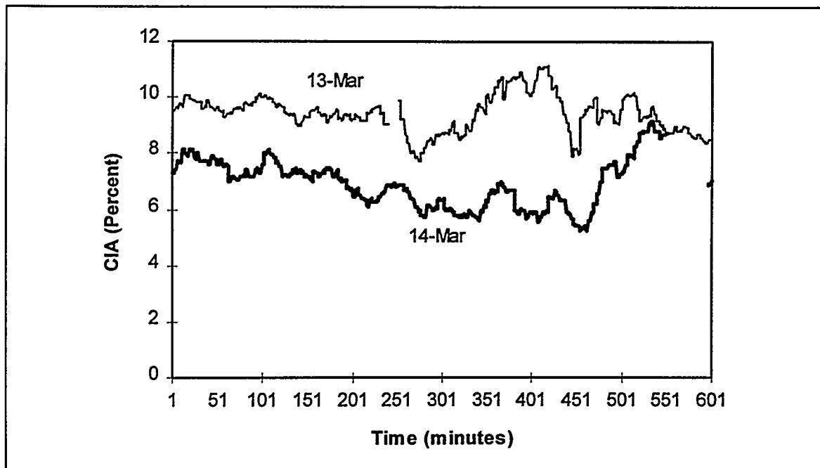
Figure 15: Kingsnorth / CIA During 10 Hour Periods on Consecutive Days
