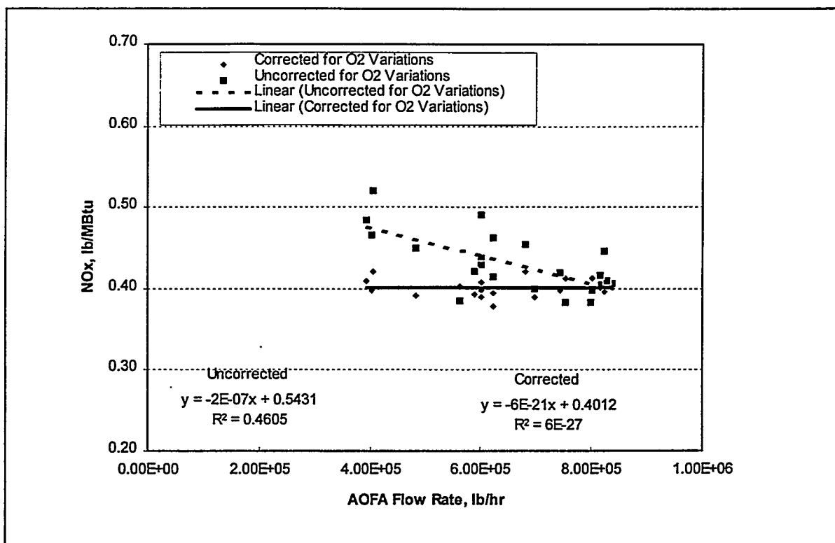
Figure 8: NO x vs AOFA Flow Rate at 450 MW
