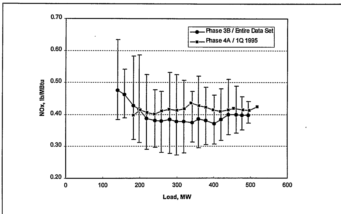
Figure 12: 1st Quarter 1995 NO x Emission Levels
