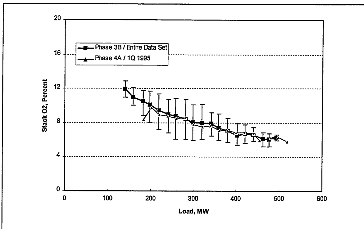
Figure 11: 1st Quarter 1995 Stack O 2 Levels
