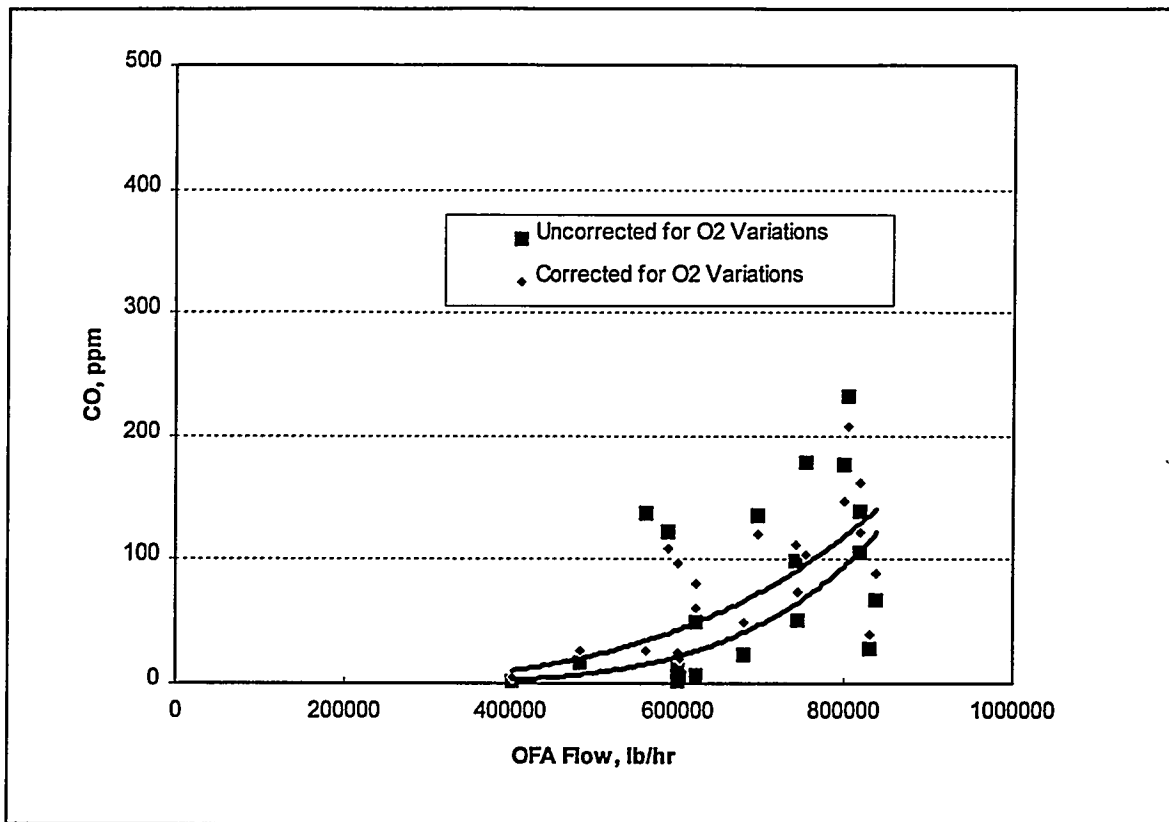
Figure 10: CO vs AOFA Flow Rate at 450 MW
