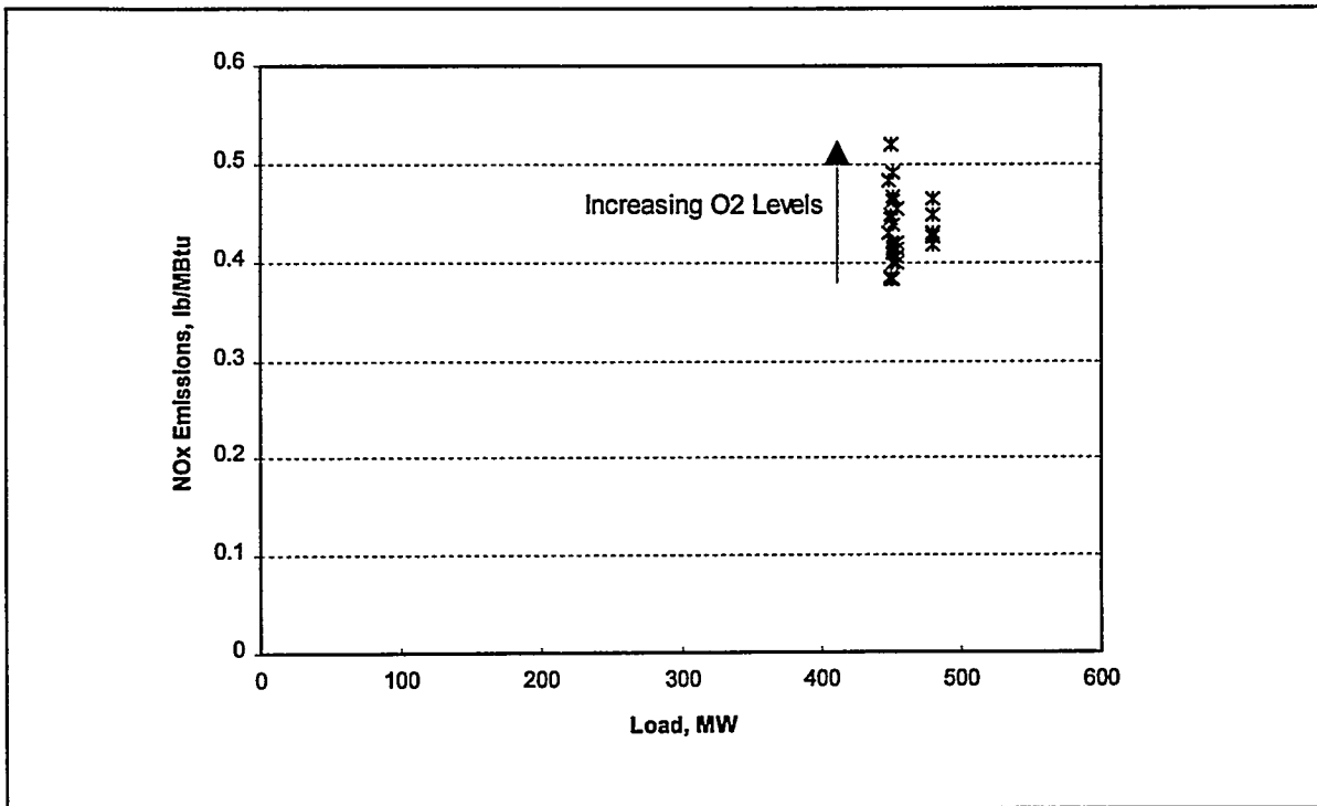
Figure 5: NO x vs. Load
