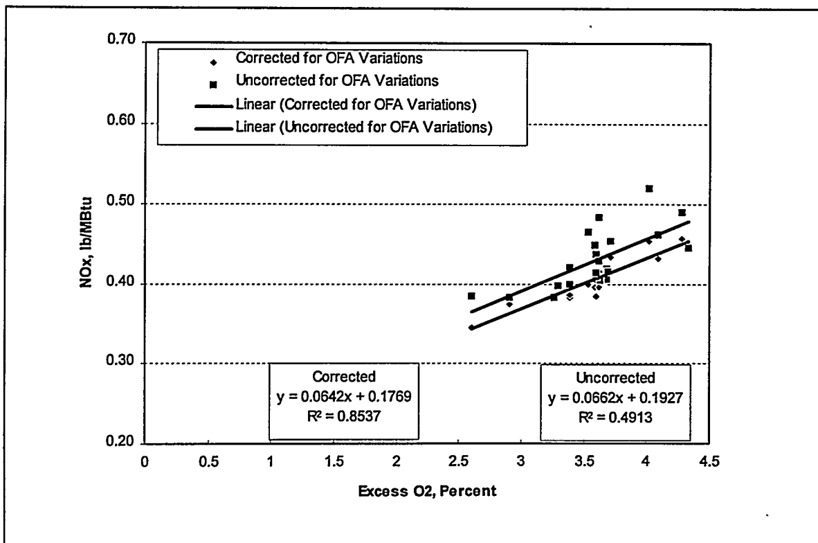
Figure 7: NO x vs Excess O 2 at 450 MW
