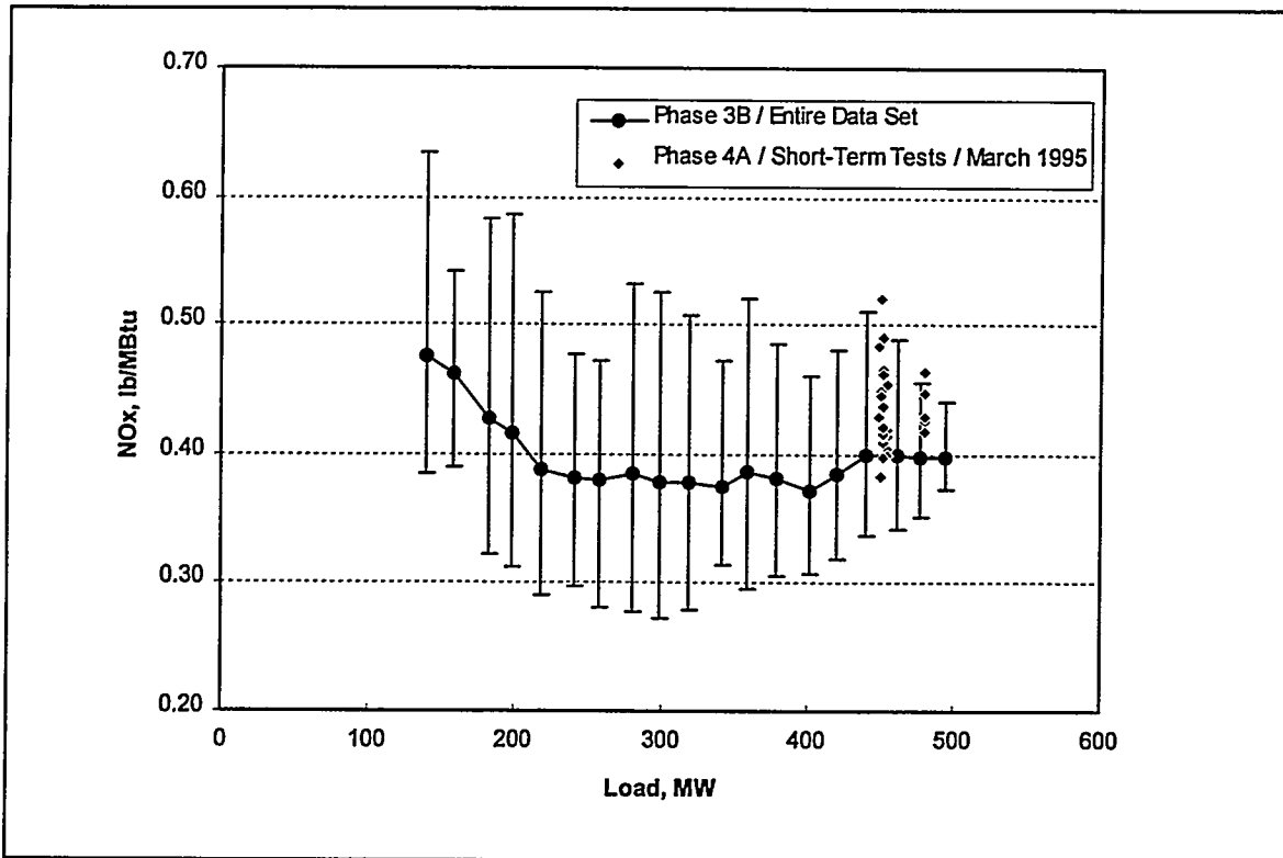
Figure 6: Comparison of 1Q 95 Test Data to Phase 3B Long-Term Data
