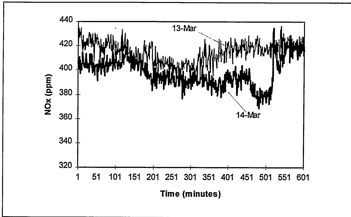
Figure 14: Kingsnorth / NO x During 10 Hour Period on Consecutive Days
