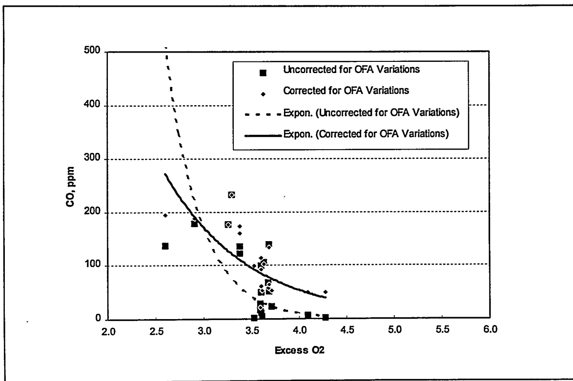
Figure 9: CO vs Excess O 2 at 450 MW
