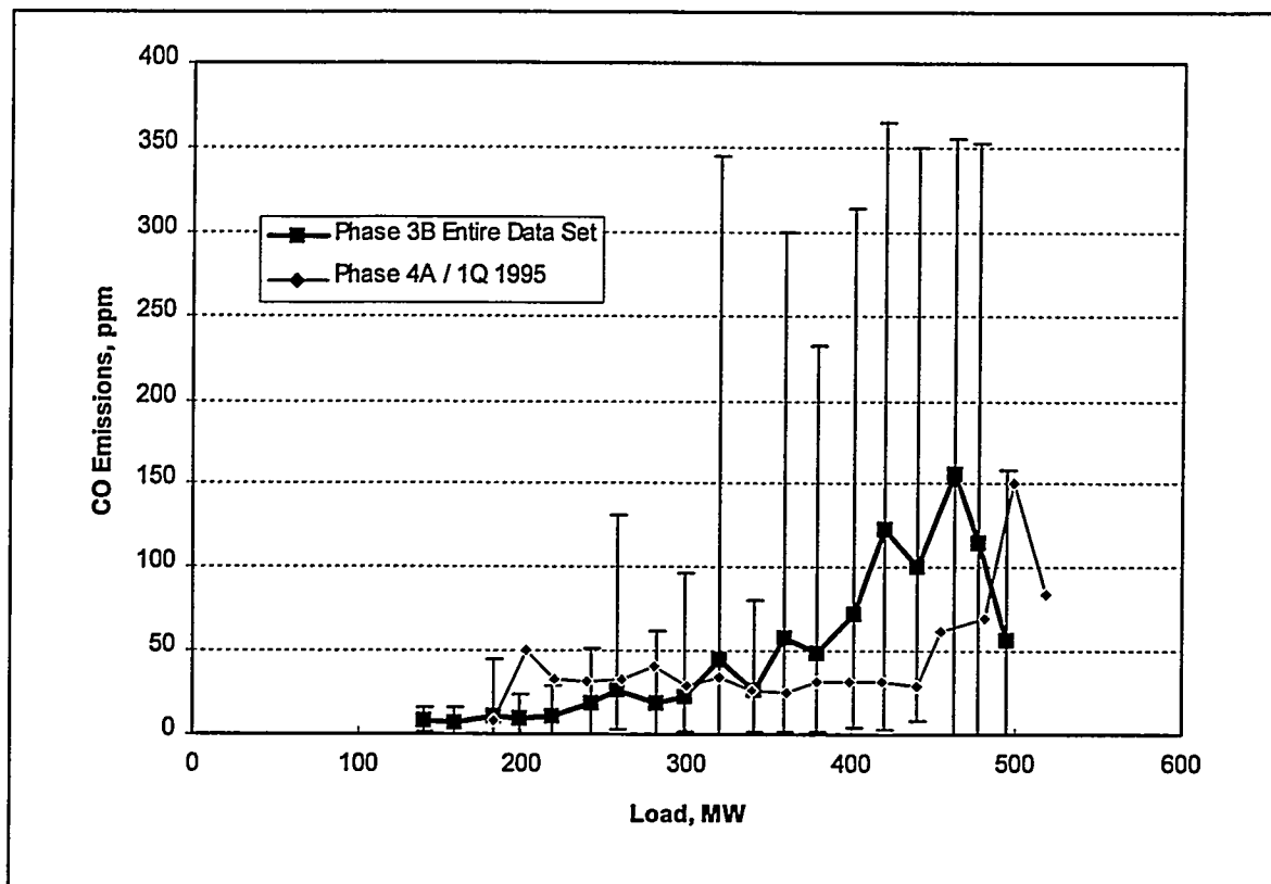
Figure 13: 1st Quarter 1995 CO Emission Levels
