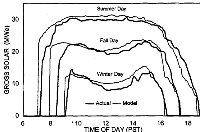
FIGURE 2. ACTUAL AND PROJECTED GROSS SOLAR ELECTRIC OUTPUT FOR SUMMER, FALL, AND WINTER DAYS
