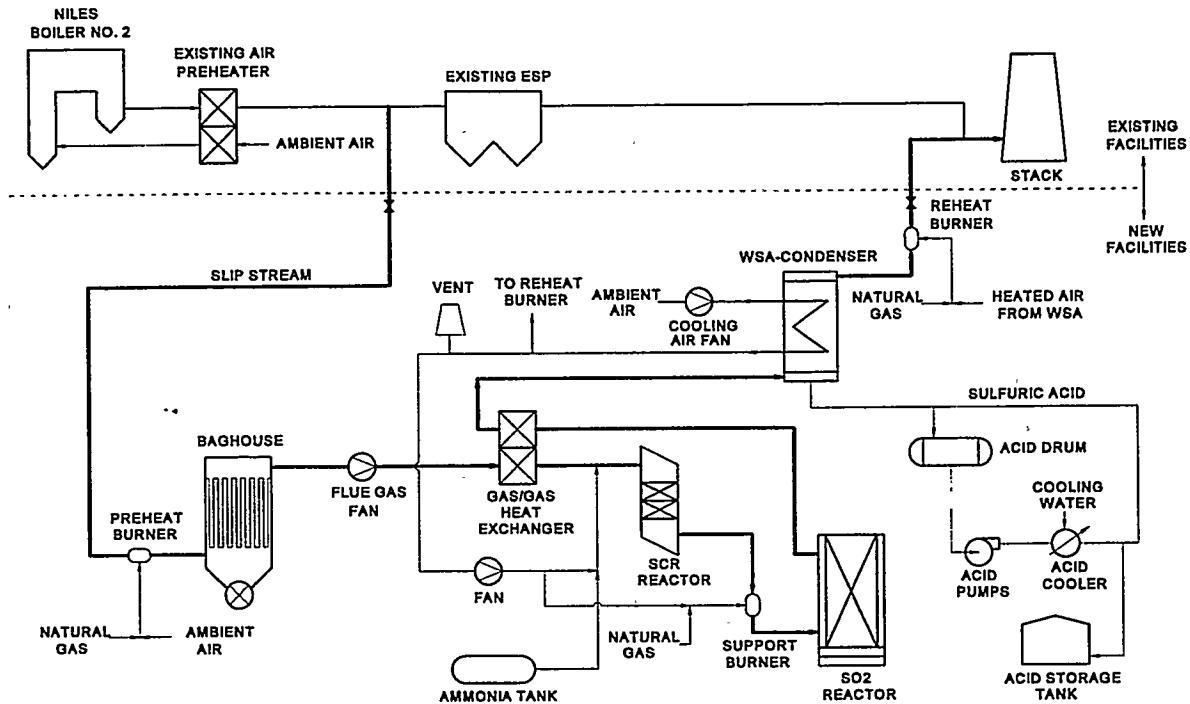
Figure 1-2 Niles SNOX Plant Process Flow Diagram
