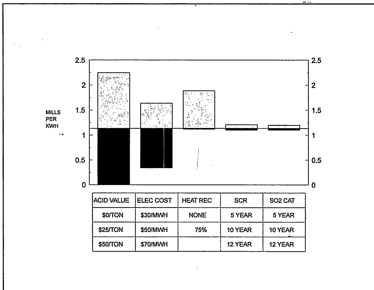
Figure 7-1 O&M Cost Sensitivity Analysis
