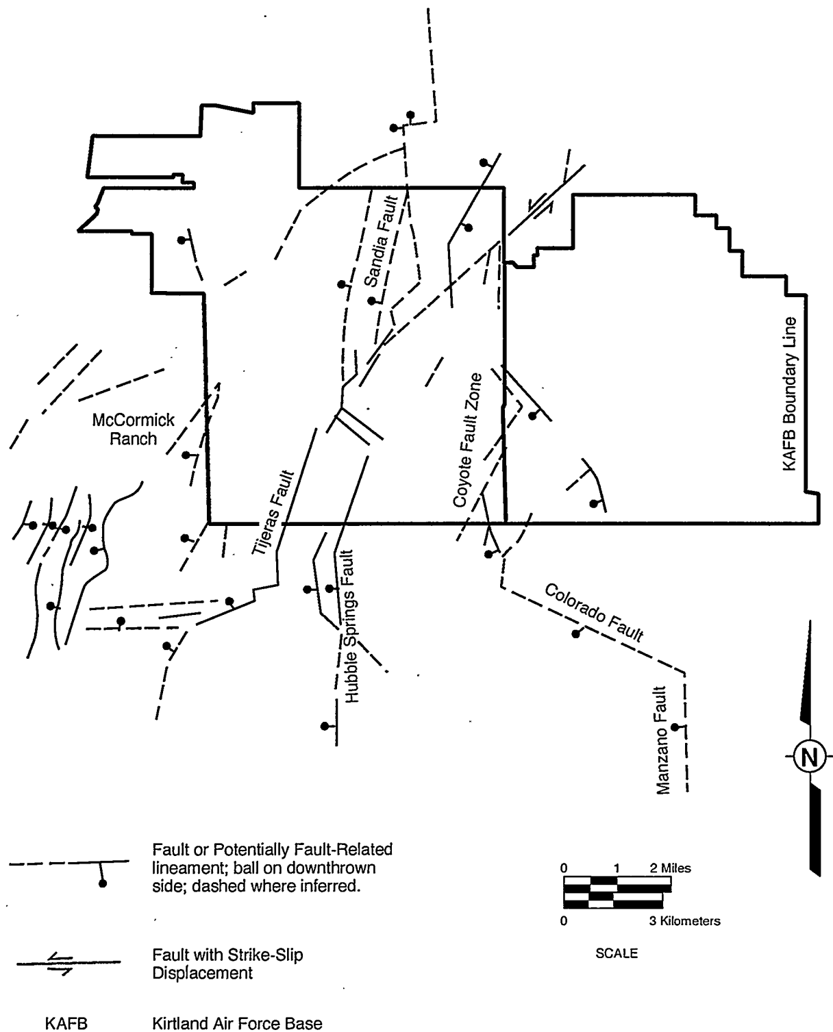
Figure 2-5 Map of Local Structural Features in the Sandia National Laboratories/New Mexico and Kirtland Air Force Base Area
