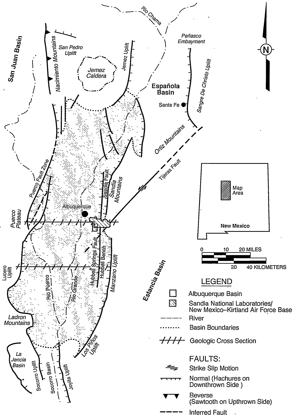
Figure 2 -1 Regional Tectonic Setting of the Albuquerque Basin, North Central New Mexico, Sandia National Laboratories/New Mexico and Kirtland Air Force Base Area
