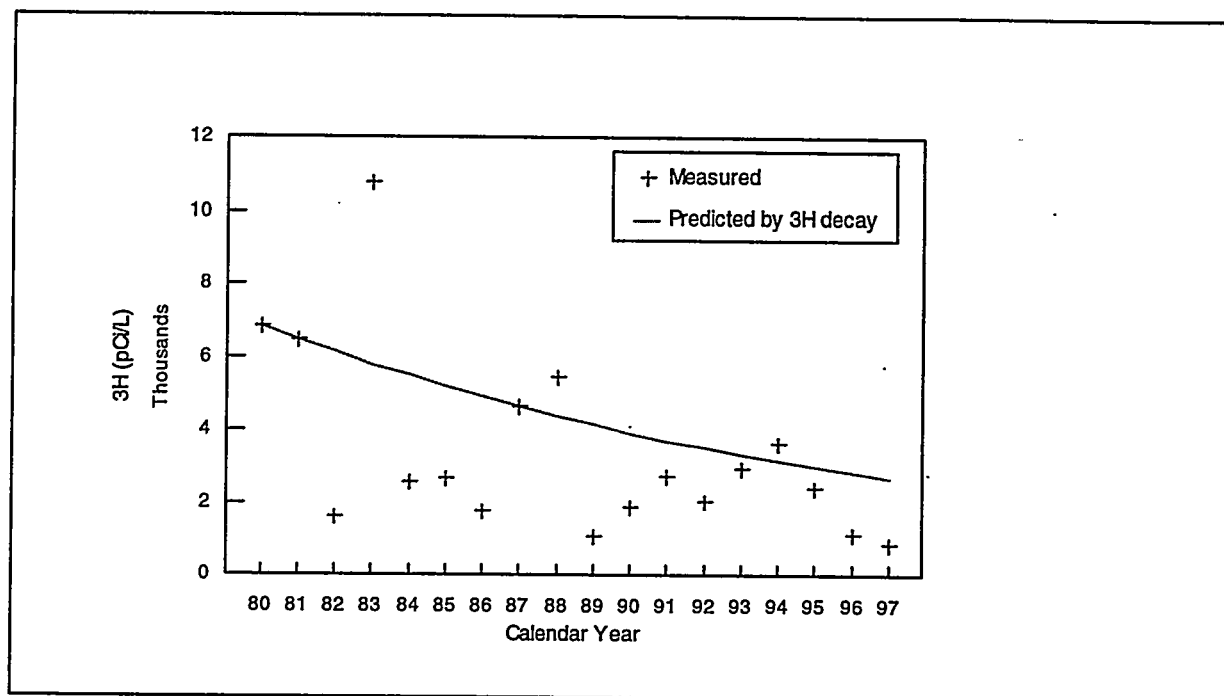
Figure 6.12 Tritium results in Well HMH-5, SALMON Site, Project DRIBBLE - 1997
