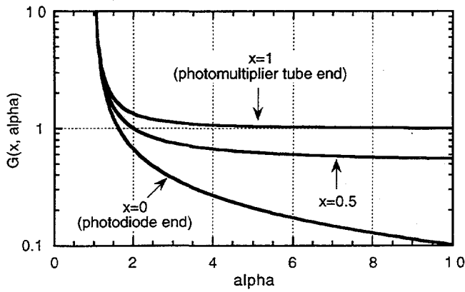
Figure 5: Dependence of the depth of interaction measurement resolution on position x ( 0 \leq x \leq 1 ) and \alpha (the light loss factor). See equation 9 for definition of G(x, \alpha) .
