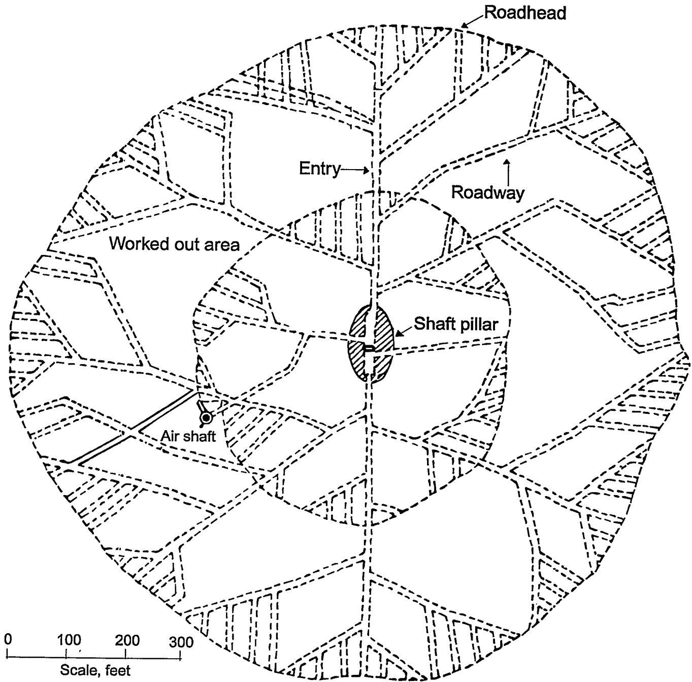
Figure 5. Early Longwall Mining
