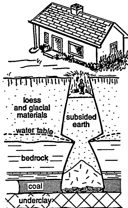
Figure 11. Cross Section of a Typical Pit Subsidence Event
