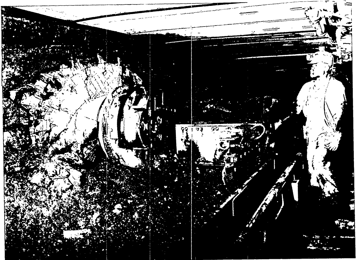
Operating at a depth of 2,140 feet, this Alabama longwall unit mines coal from the deepest vertical shaft coal mine in North America.
