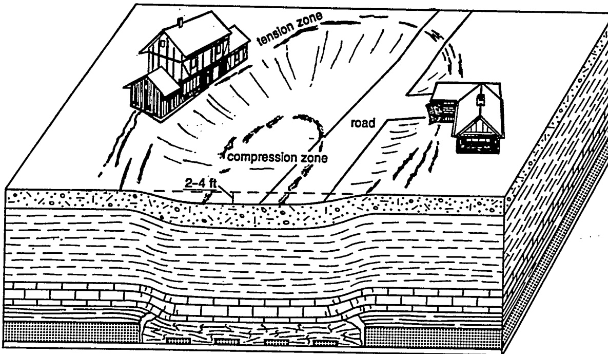
Figure 12. Diagram of a Typical Sag Subsidence Event
