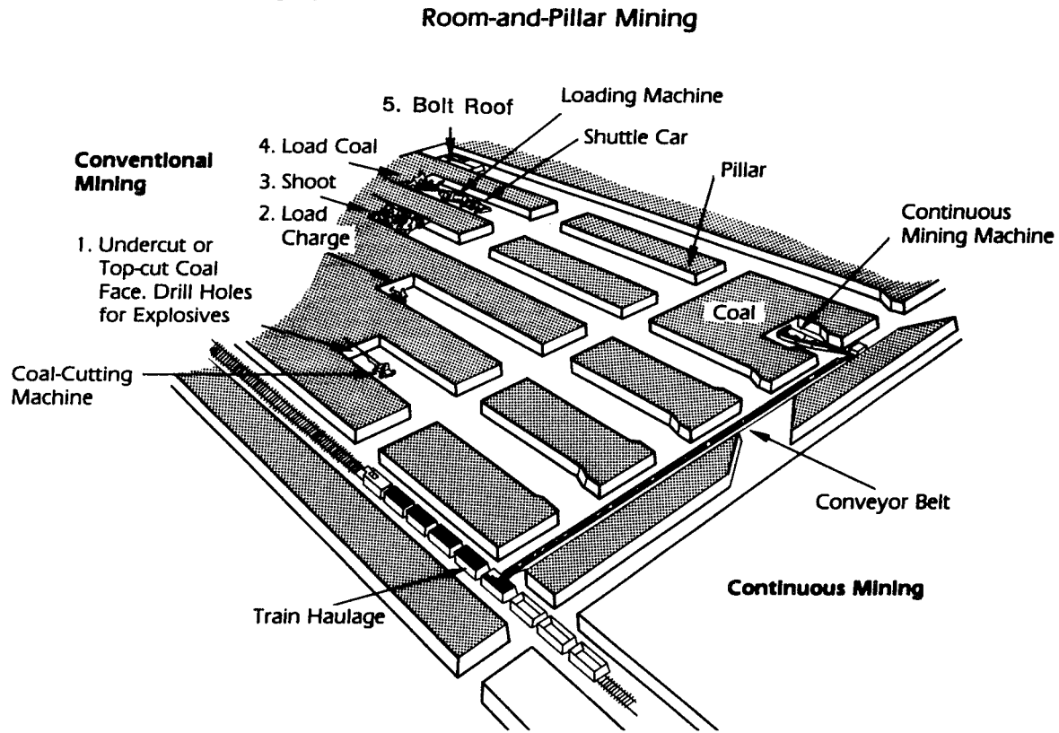
Figure 2. Underground Mining Systems
