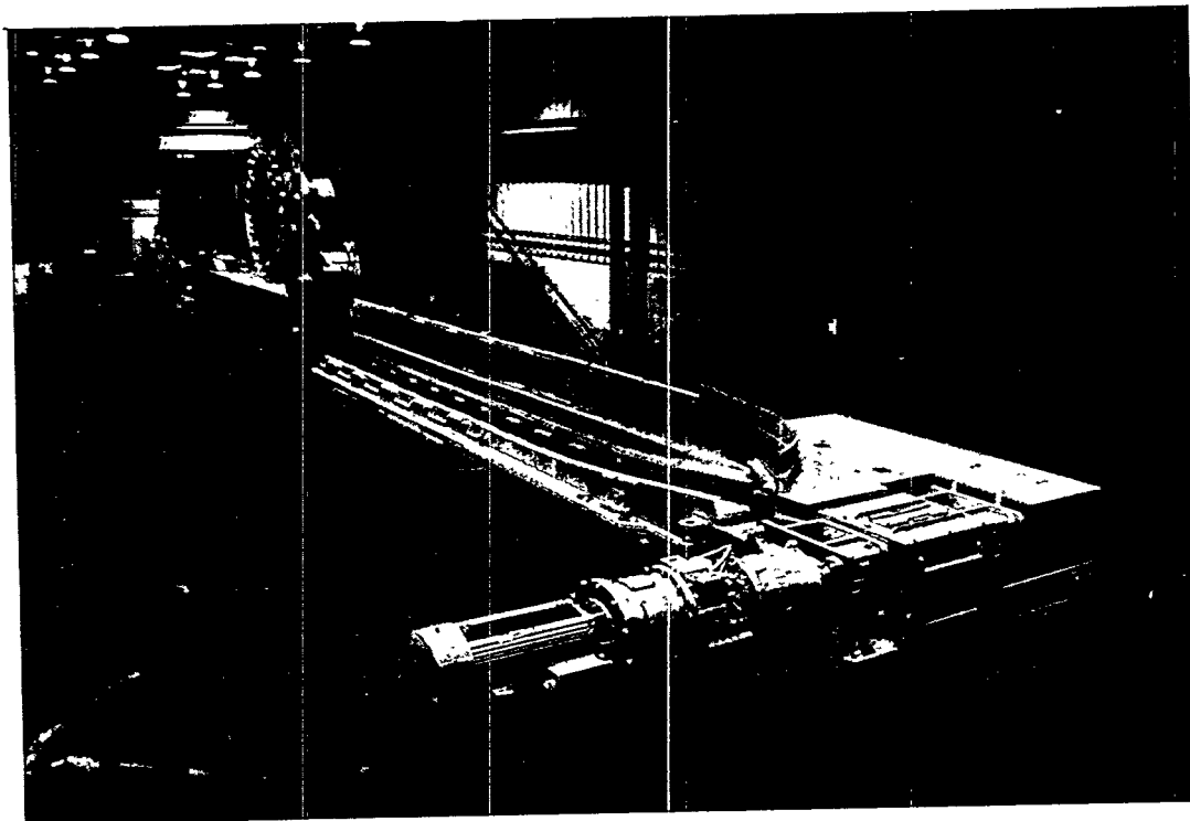
A face conveyor undergoing compatibility trials with a shearer.
