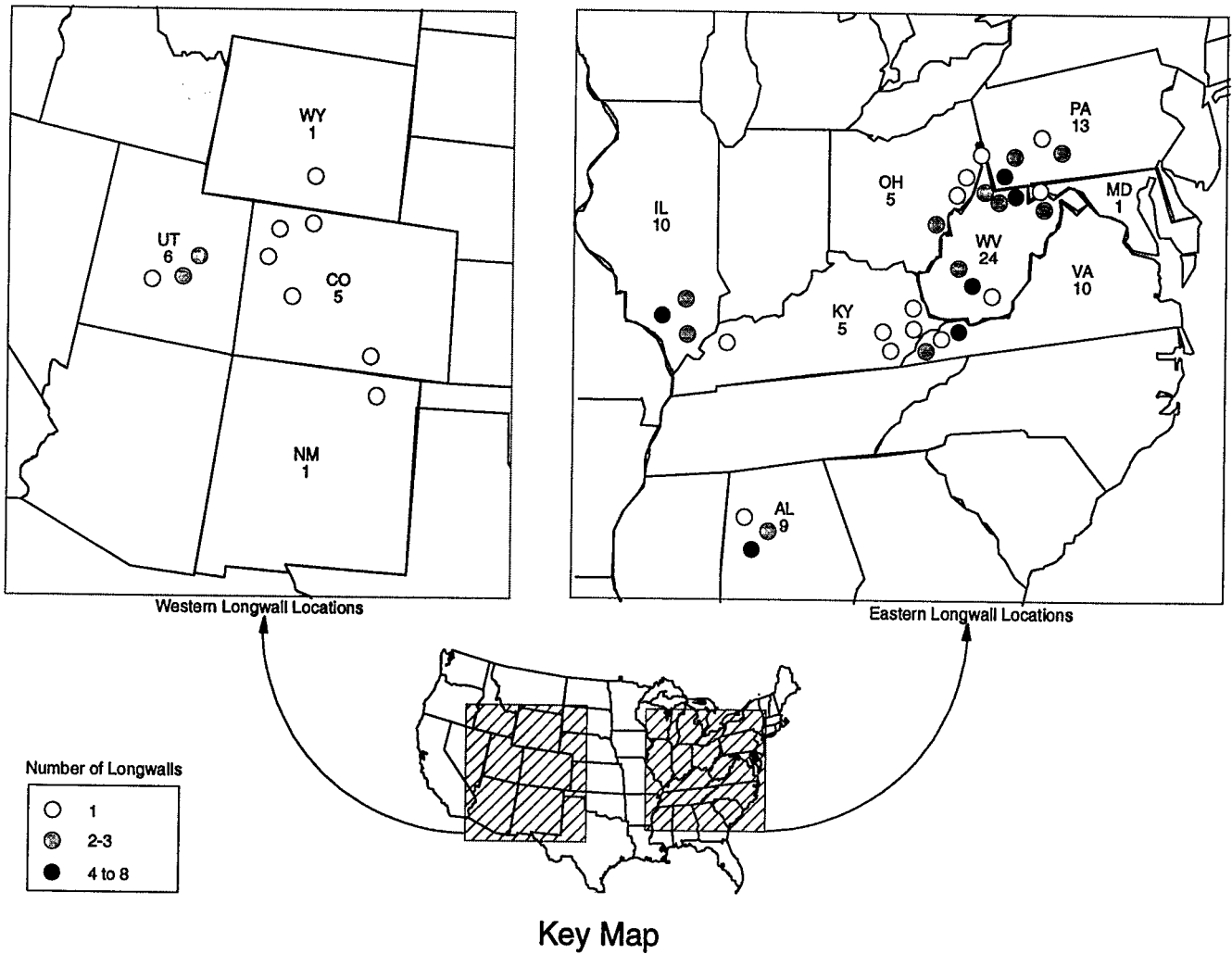
Figure 1. Location of U.S. Longwall Mining Units, 1993
