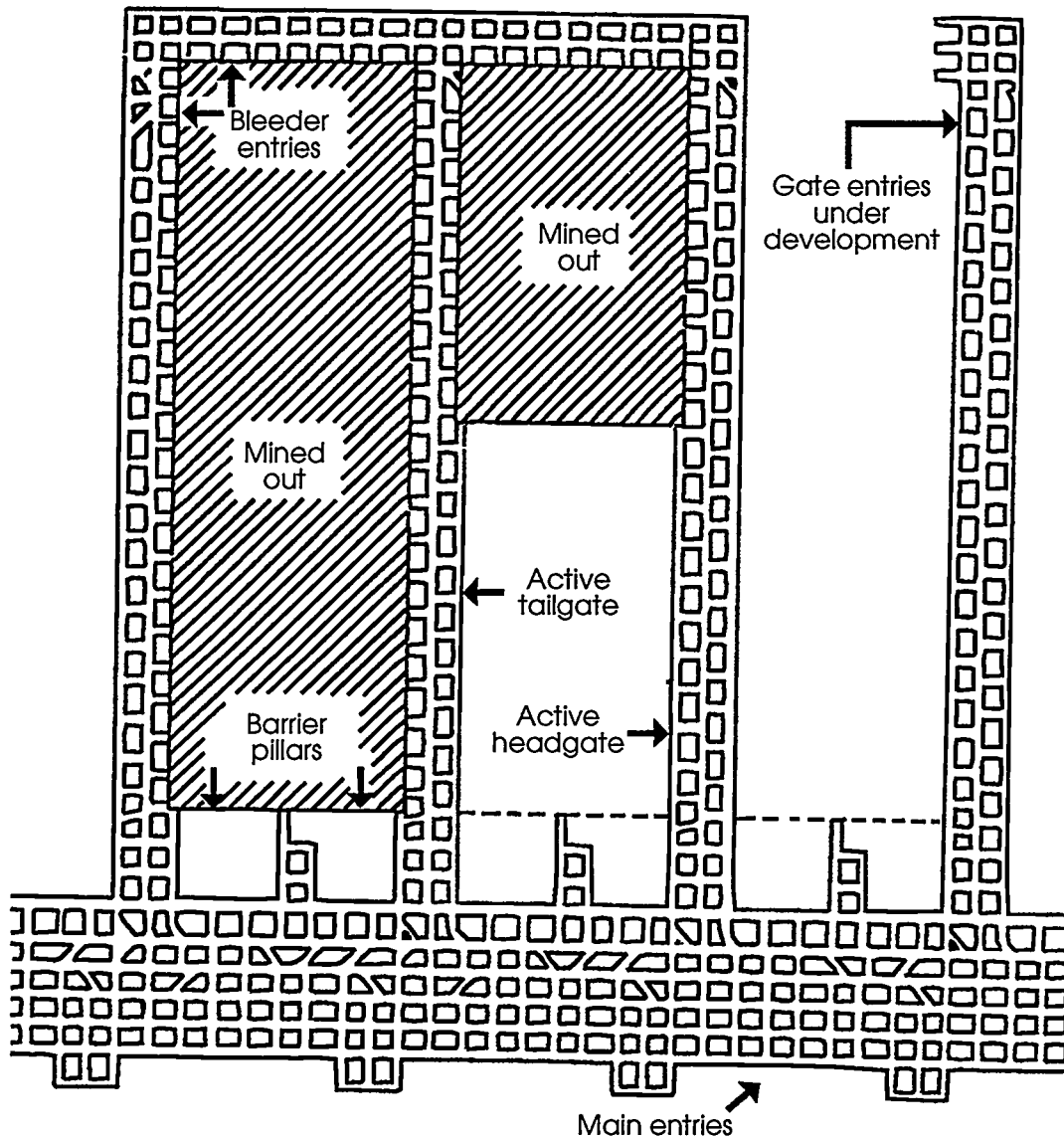
Figure 3. Plan View of U.S. Coal Mine With Longwall Operations
