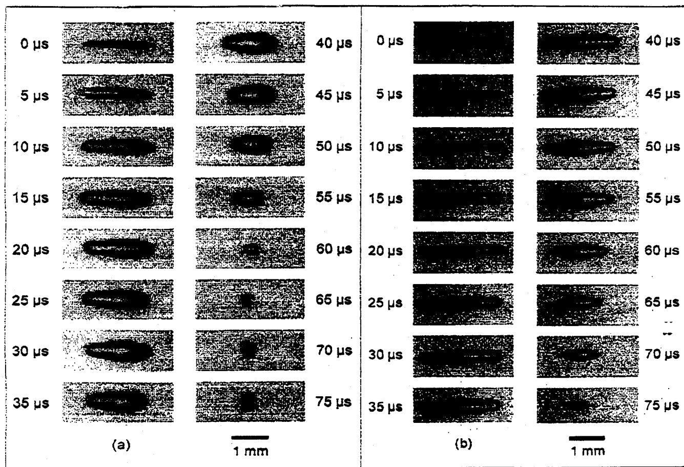
Fig. 1. Cylindrical bubble dynamics induced by 30-ps Nd:YAG laser pulses of a) 1 mJ and b) 4 mJ pulse energy which were focused into distilled water with a focusing angle of 4^\circ . The laser light was incident from the left.
