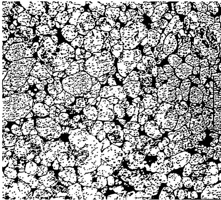
Figure 4.50. Optical micrograph of the as-polished, unetched, CIP microstructure of CAA aluminum powder.
