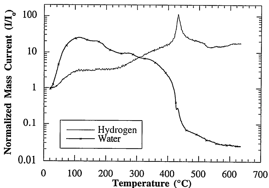
Figure 4.34. QMS water and hydrogen spectra of Al-Cu-Mg aluminum alloy powder at 5°C per minute.
