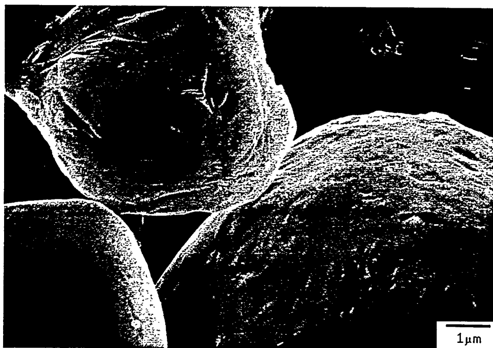
Figure 4.48. SEM micrograph of the CAA aluminum powder air sintered at 300°C for 24 hours.
