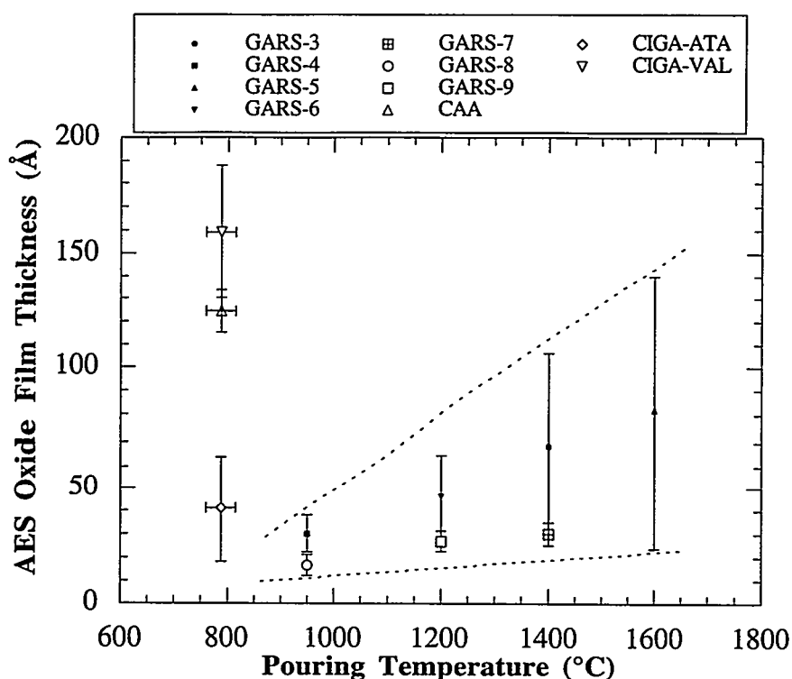
Figure 4.22. AES oxide film thickness as a function of pouring temperature.
