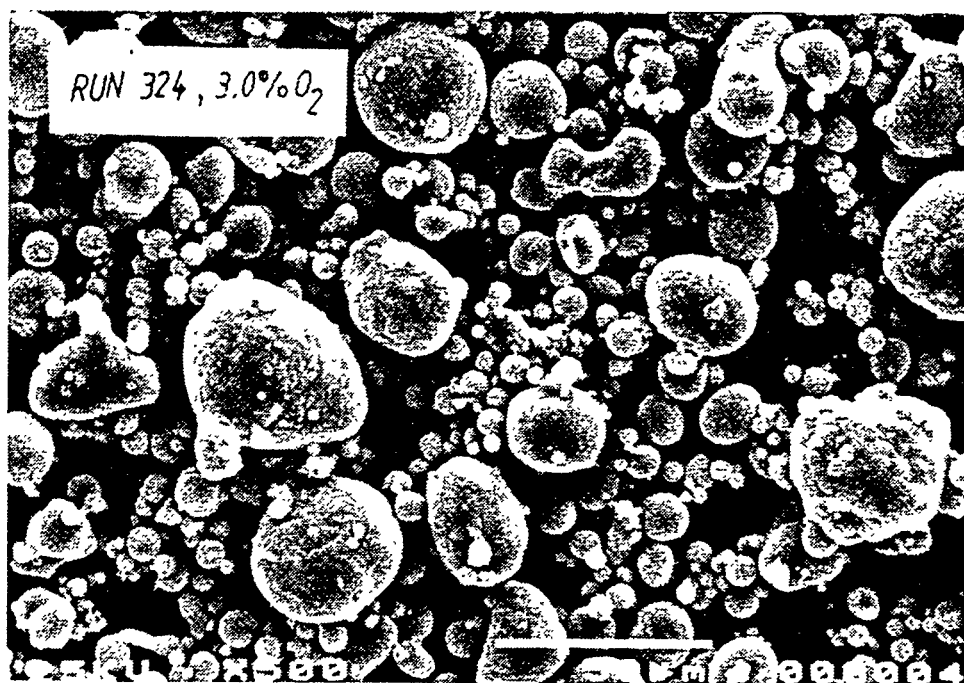
Figure 5.3. SEM micrograph of aluminum powder produced by gas atomization with a mixture of 3.0 volume percent oxygen in nitrogen gas [13].
