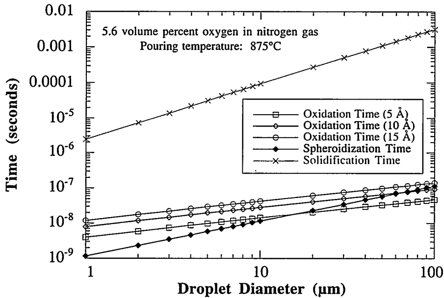
Figure 5.8. Comparison of atomization time scales for aluminum powder nitrogen gas atomized with 5.6 volume percent oxygen in the atomization gas.
