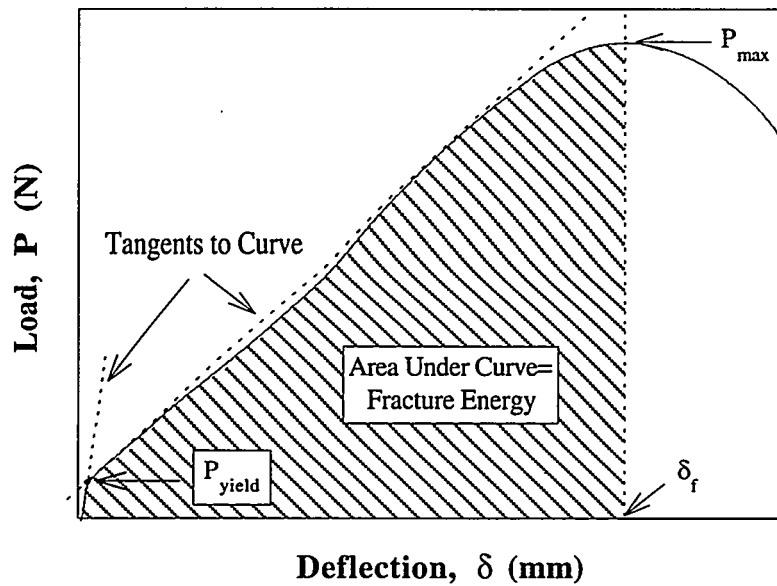
Figure 3.5. Example of the punch test raw data as recorded on a load-deflection curve.
