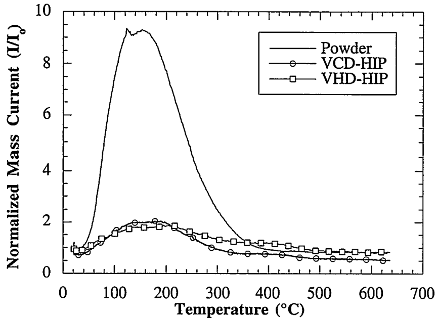
Figure 4.58. QMS results of water evolution from GARS-4 powder samples in the as-atomized powder state and consolidated states.
