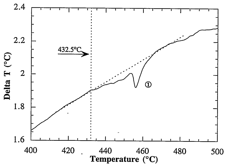
b. Expanded view of DTA trace to highlight peak one.
