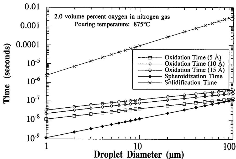
Figure 5.9. Comparison of atomization time scales for aluminum powder nitrogen gas atomized with 2.0 volume percent oxygen in the atomization gas.
