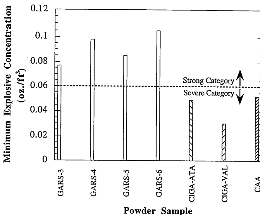
Figure 4.43. MEC data of pure aluminum powders.
