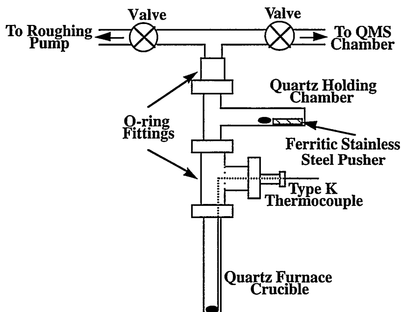
Figure 3.2. Schematic of the QMS sample chamber used for this research.
