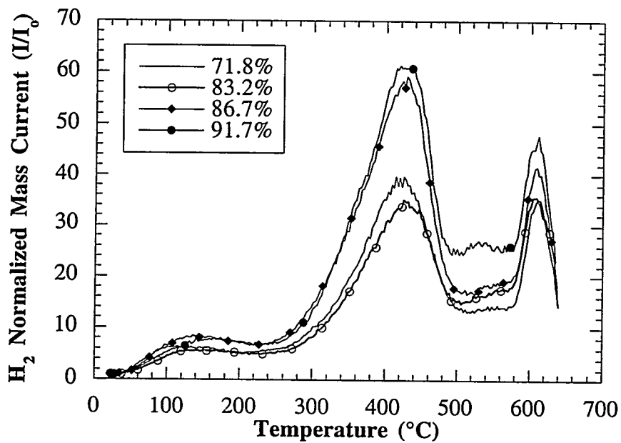
Figure 4.18. The effect of sample density variations during QMS analyses of CIGA powder at constant heating rate of 10 ^{\circ}C per minute.
