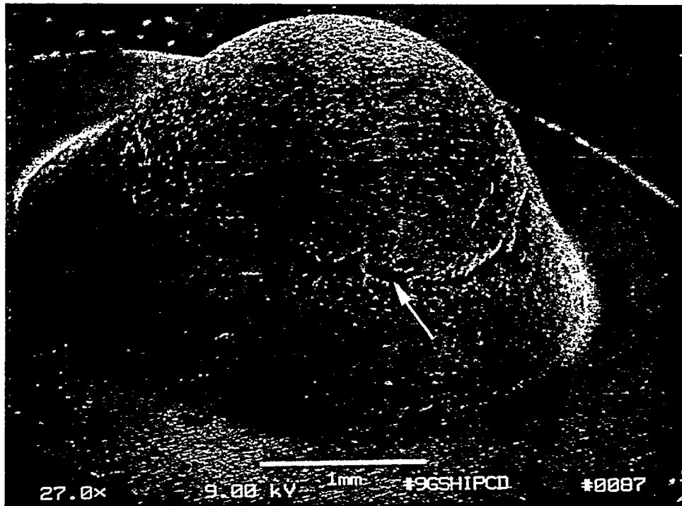
Figure 4.62. SEM micrograph of a punch test coupon after testing. The white arrow indicates the area shown in Figure 4.62, below.
