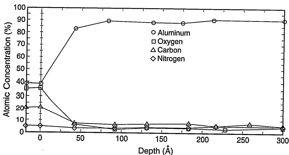
Figure 4.19. Representative AES concentration depth profile for GARS aluminum powders.
