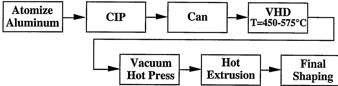
b. Conventional consolidation sequence for aluminum powders used in aerospace applications as described in [1].
