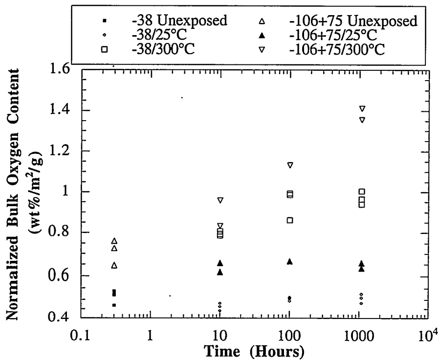
Figure 4.45. Normalized oxygen content of GARS-9 aluminum powders used for MEC experiment.
