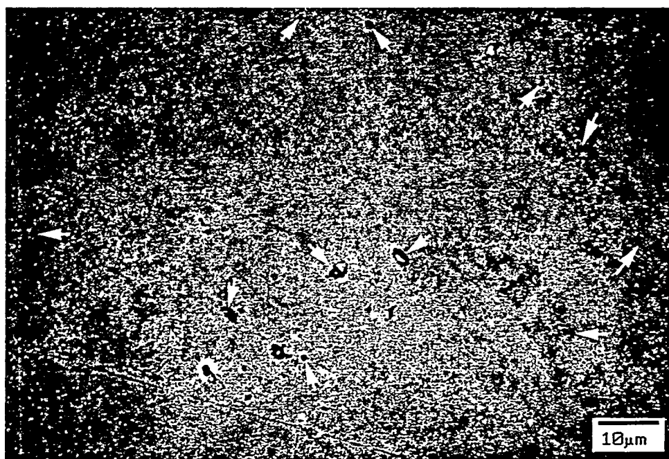
Figure 4.53. SEM micrograph showing the CIP-VHD-HIP microstructure of the CAA aluminum powder. The white arrows indicate the residual porosity in the sample.
