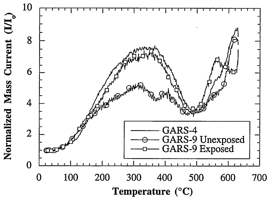
Figure 4.39. QMS hydrogen spectra of GARS-9 aluminum in the unexposed state and exposed for greater than 3000 hours.
