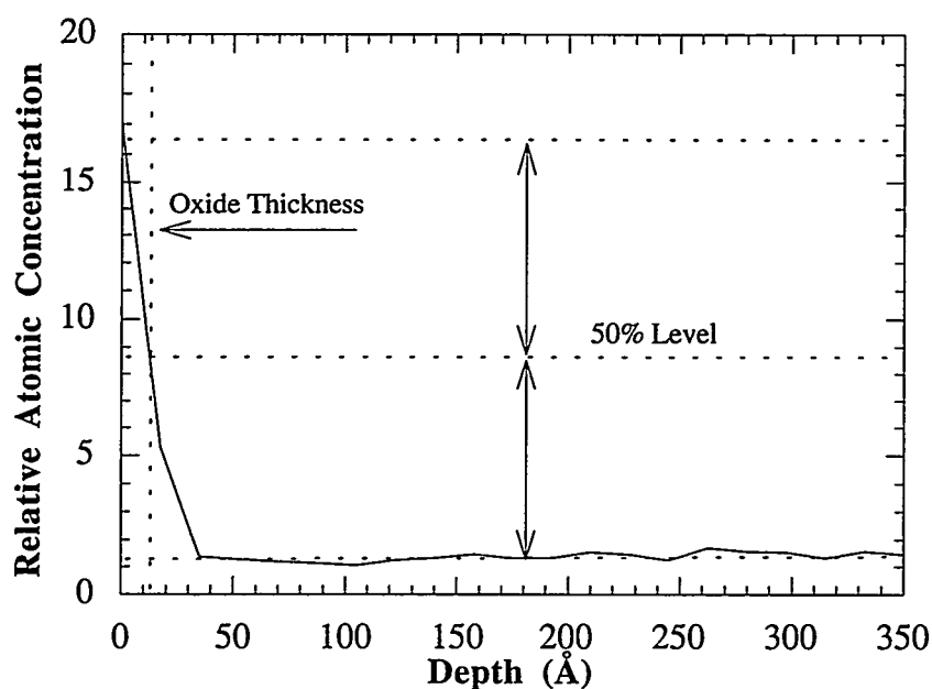
Figure 4.21 Example AES oxygen depth profile for the measurement method used to determine the oxide thickness of aluminum powders.
