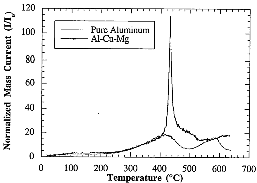
Figure 4.36. QMS hydrogen spectra of SSA pure aluminum powder and a Al-Cu-Mg aluminum alloy powder heated at 5°C per minute.
