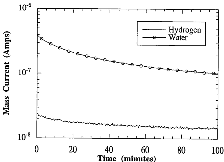
Figure 4.7. QMS plot illustrating the signal decrease of the water and hydrogen during the two hour UHV ambient temperature degassing procedure.
