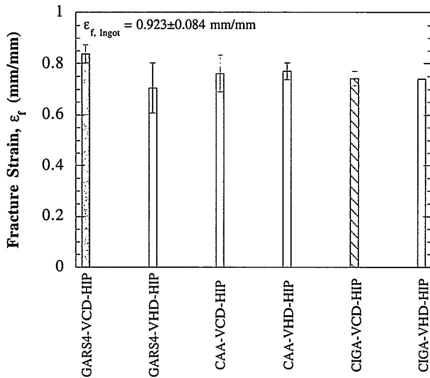
Figure 4.66. Fracture strain results from punch testing the GARS-4, CAA, and CIGA-ATA aluminum powders consolidated by CIP-VCD-HIP and CIP-VHD-HIP routes.
