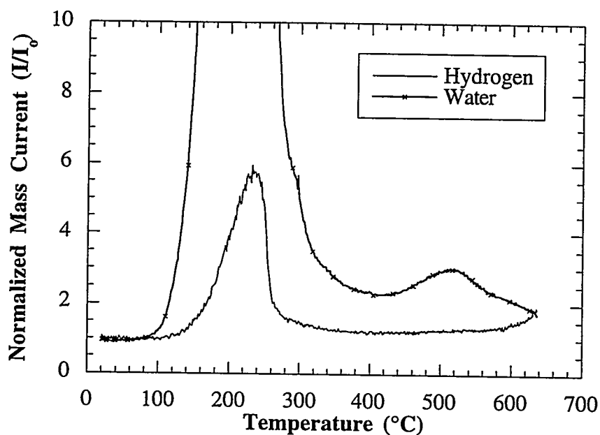
b. Expanded view of QMS scan to highlight the water peak at about 520°C.
