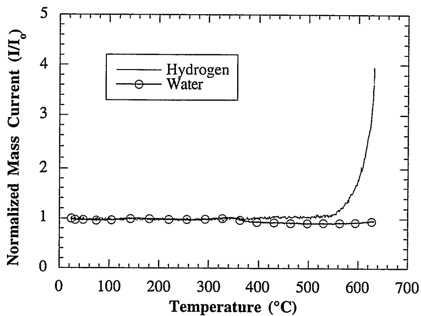
Figure 4.8. QMS water and hydrogen spectra for the empty furnace crucible heated at 5^{\circ}\text{C}/\text{min} .
