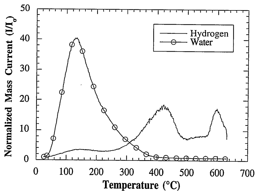
Figure 4.12. Representative QMS plot of CIGA-ATA aluminum powder heated at 5^{\circ}\text{C}/\text{min} .
