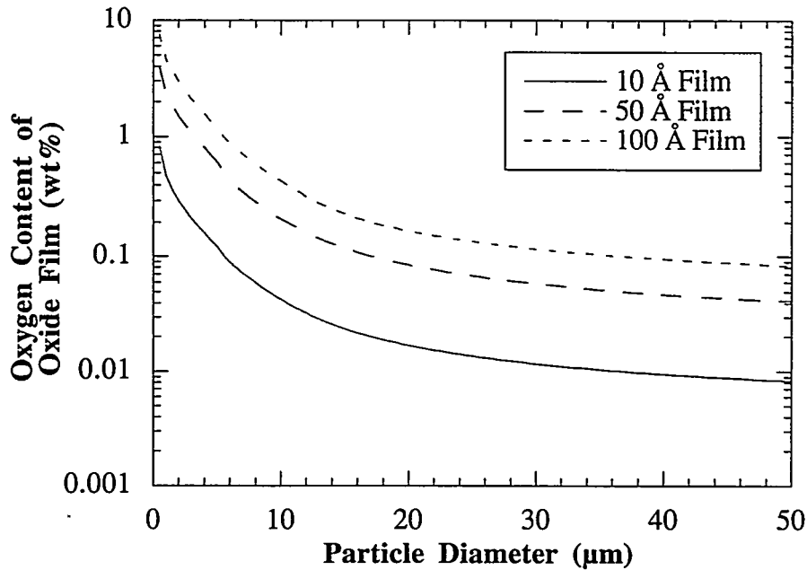
Figure 5.12. Plot of oxygen content of the oxide film on aluminum powder particle as a function of particle diameter and oxide film thickness.
