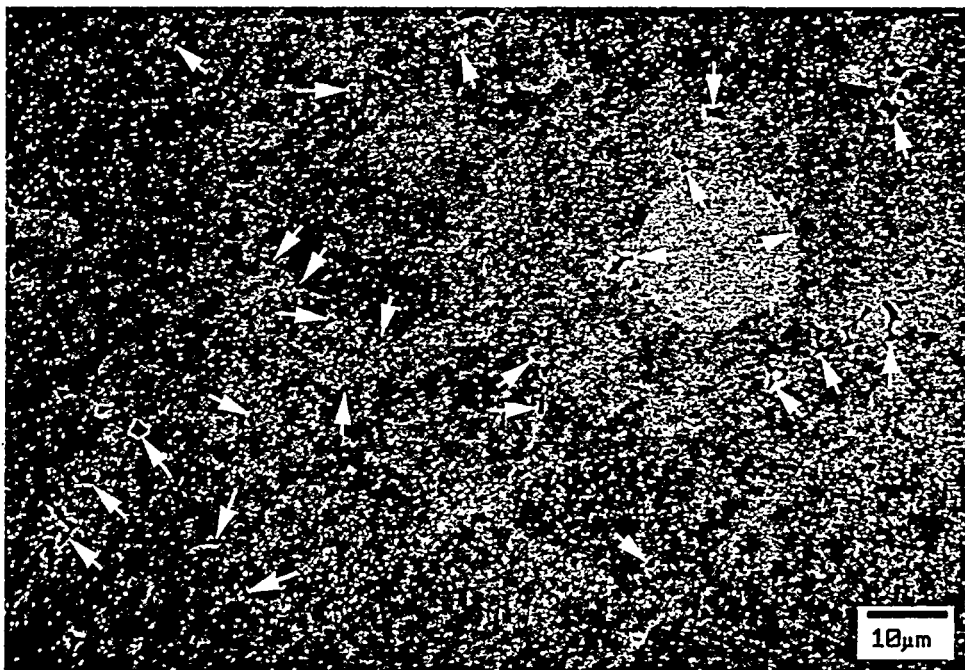
Figure 4.55. SEM micrograph showing the CIP-VHD-HIP microstructure of GARS aluminum powder. The white arrows indicate the residual porosity in the sample.
