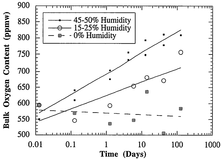
Figure 4.38. Oxidation behavior of GARS pure aluminum powders exposed to air atmosphere with various levels of humidity. The lines are drawn only to guide the eye.
