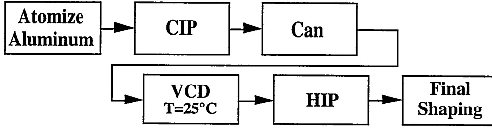
a. Modified consolidation sequence for aluminum powders used for this research.
