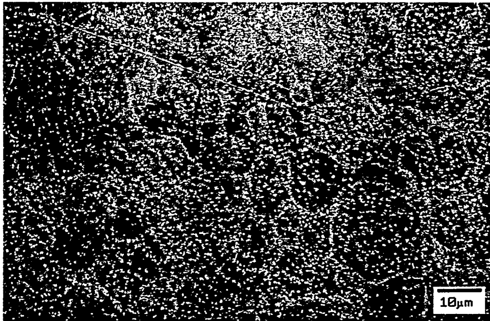
Figure 4.54. SEM micrograph showing the CIP-VCD-HIP microstructure of the GARS aluminum powder. No residual porosity is observed in the sample.
