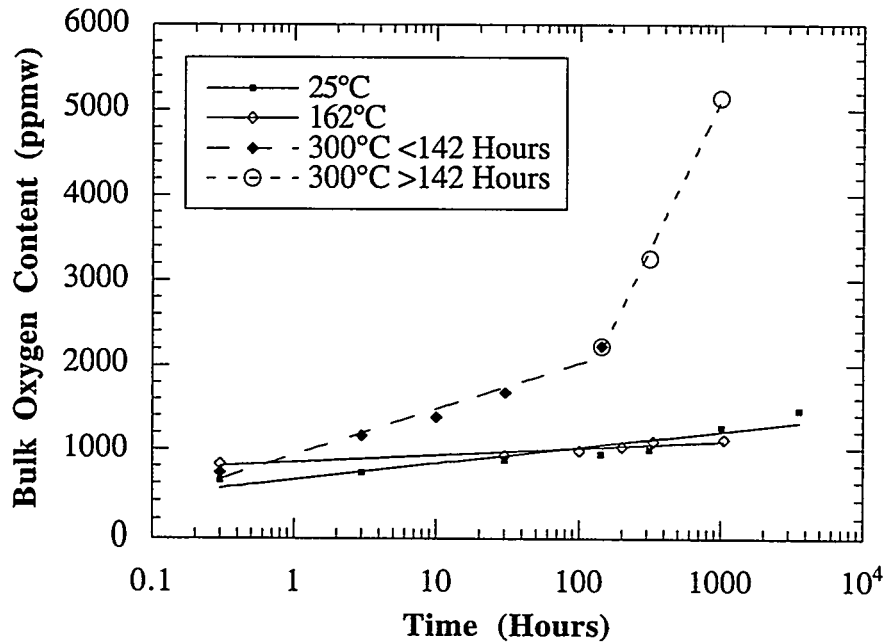
Figure 4.41. Oxidation behavior of Al-Ti-Y alloy powder as exposed to ambient air and different thermal conditions.
