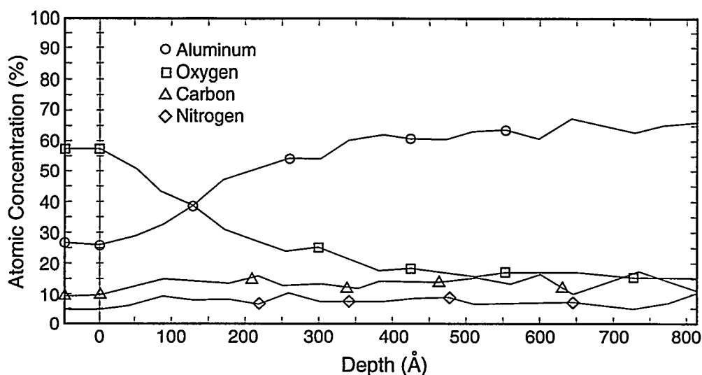
Figure 4.20. Representative AES concentration depth profile for CAA aluminum powders.
