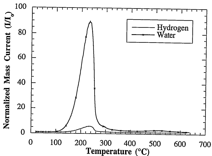
a. Overall QMS water and hydrogen scan of the trihydrate alumina.
