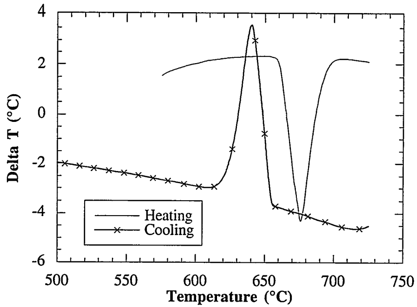
Figure 4.5. DTA trace of Alcoa pure aluminum ingot.
