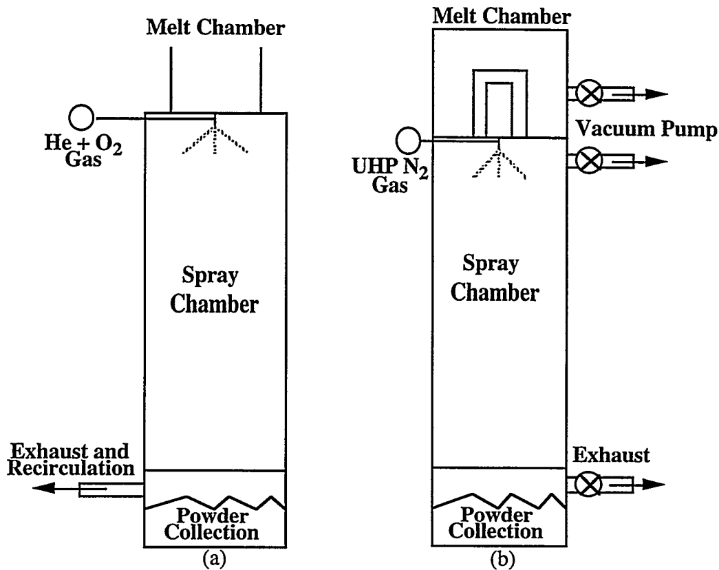
Figure 2.2. a) Schematic of vertically downward atomization system used by Valimet for CIGA-VAL aluminum powders [9]. b) Schematic of vertically downward atomization system used for GARS aluminum powder processing.
