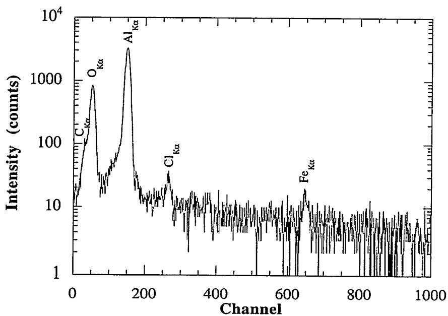
Figure 4.27. EDS spectra of the oxide film on GARS-8 aluminum powder.
