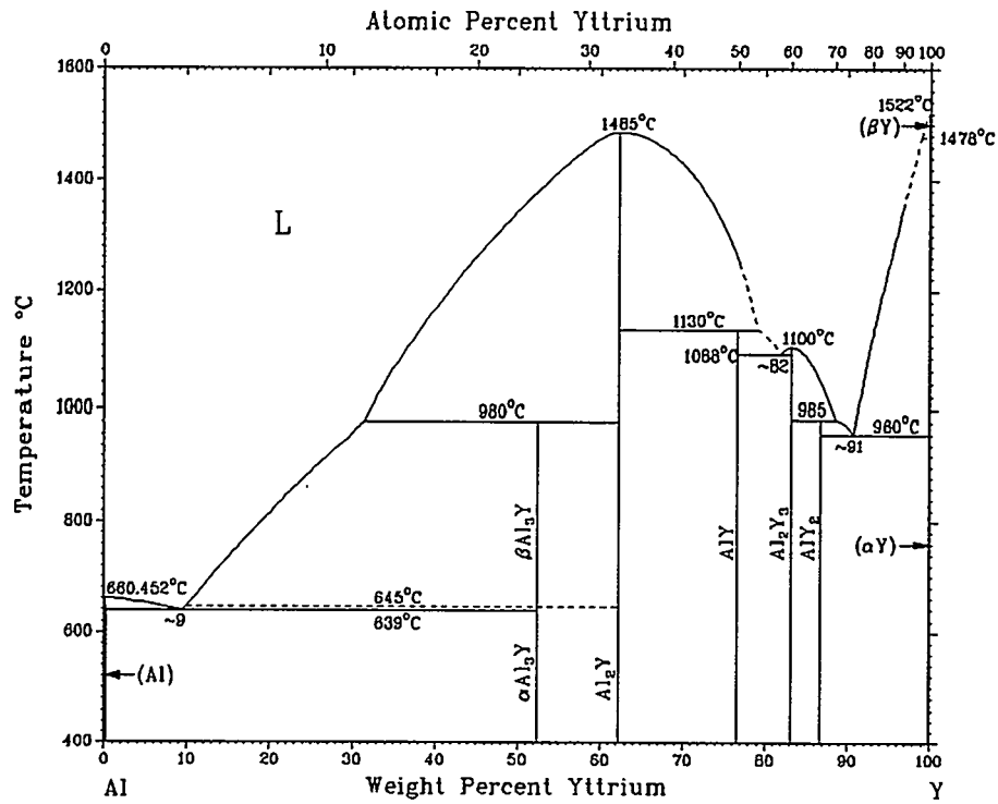
Figure 4.32. Aluminum-yttrium phase diagram [82].
