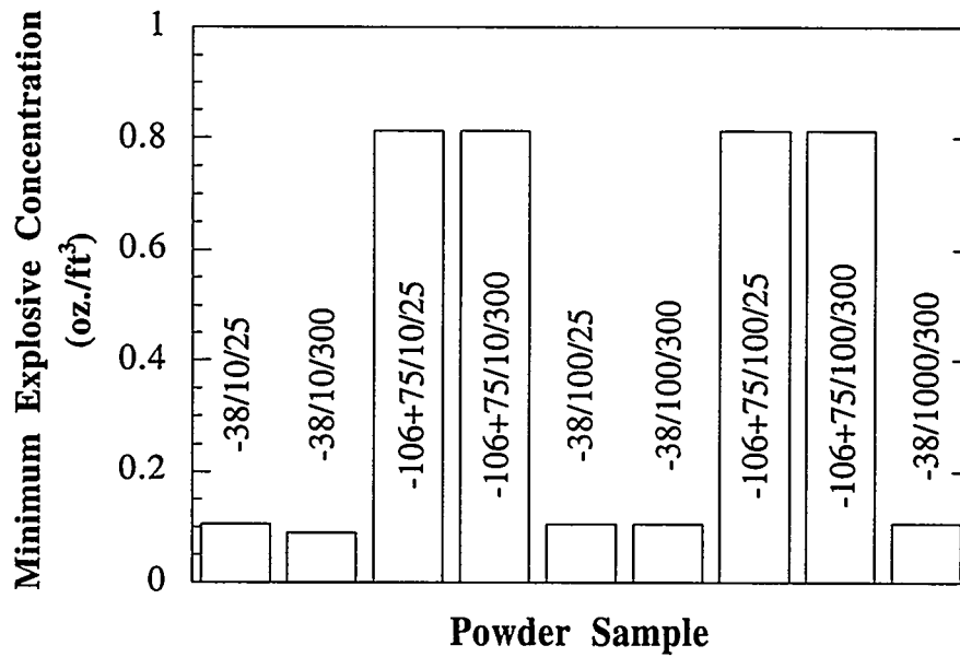
Figure 4.44. MEC data of GARS-9 aluminum powder.
