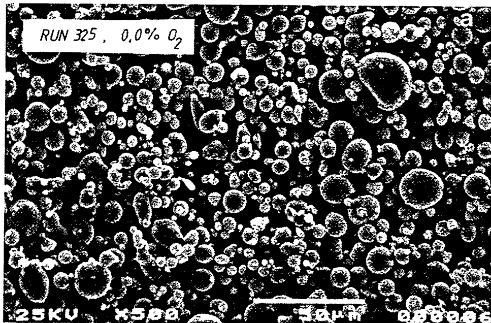
Figure 5.2. SEM micrograph of aluminum powder produced by gas atomization with a mixture of 0.0 volume percent oxygen in nitrogen gas [13].
