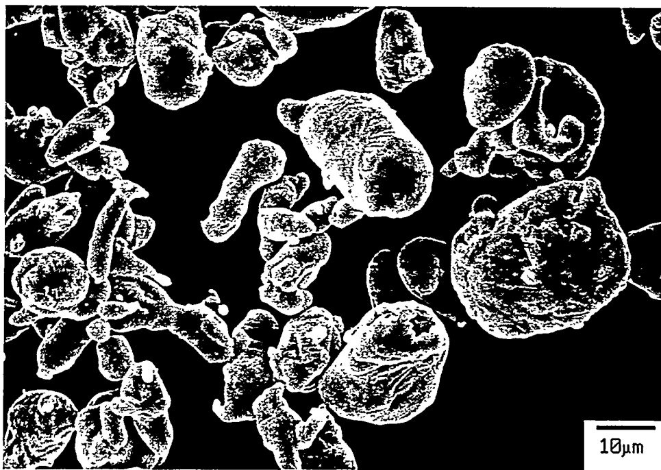
Figure 4.3. SEM micrograph of the as-atomized CAA aluminum powder.
