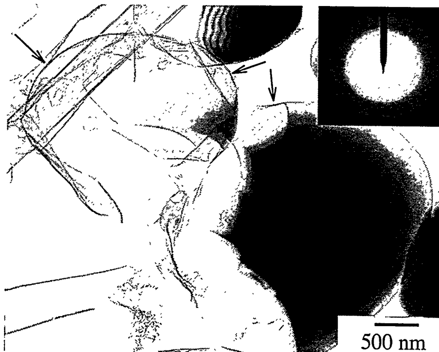
Figure 4.24. TEM micrograph and SAD pattern of the oxide film on GARS aluminum powder. The arrows indicate oxide thickness measurements.
