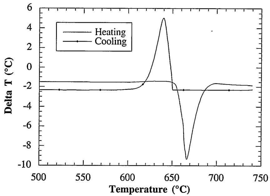
Figure 4.6. DTA scan of the GARS-6 pure aluminum powder in the as-atomized state.
