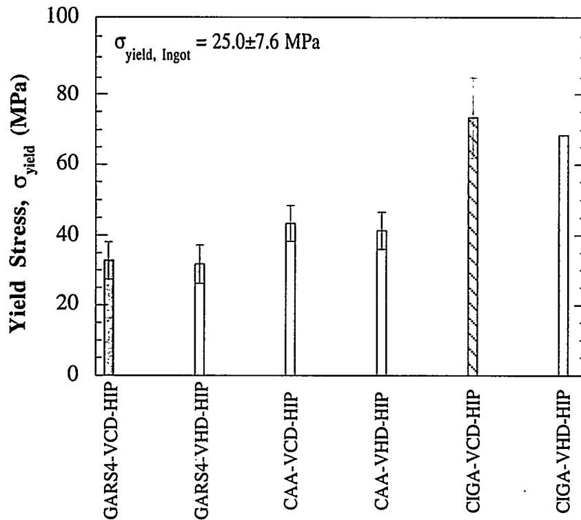
Figure 4.64. Yield stress results from punch testing the GARS-4, CAA, and CIGA-ATA aluminum powders consolidated by CIP-VCD-HIP and CIP-VHD-HIP routes.
