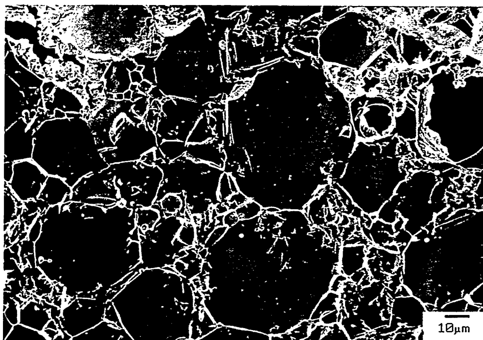
Figure 4.29. SEM micrograph of GARS-8 aluminum powder TEM sample in Figure 4.24.
