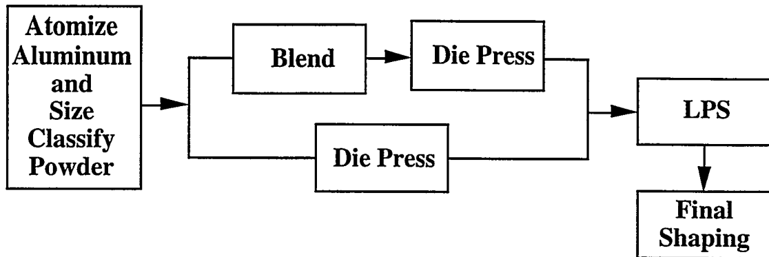
Figure 2.4. Press and liquid phase sintering (LPS) route for aluminum P/M components.
