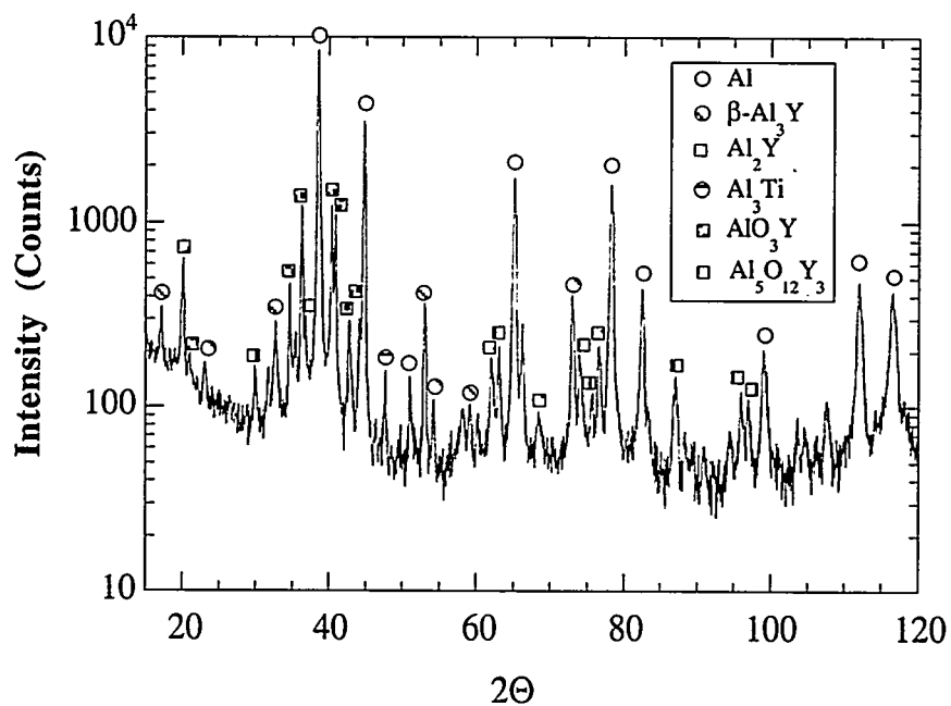
Figure 4.30. XRD scan of Al-Ti-Y powder in the as-atomized state.
