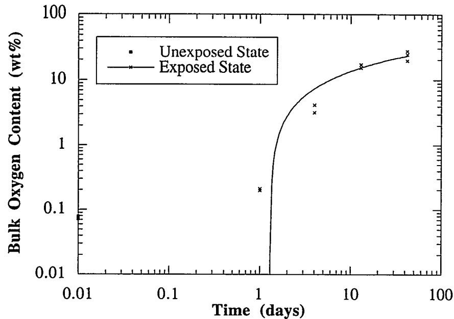
Figure 4.40. Controlled air exposure of aluminum powder in 85% relative humidity at 29.4°C. The line is drawn only to guide the eye.
