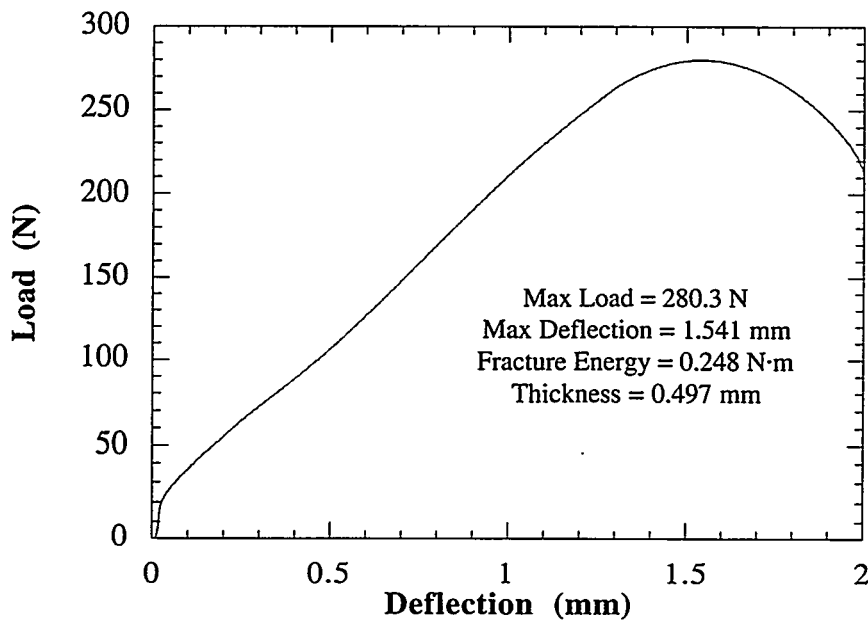
Figure 4.61. An example punch test plot of a consolidated CAA aluminum powder, illustrating the nearly ideal behavior of the consolidated powders samples during the punch test.
