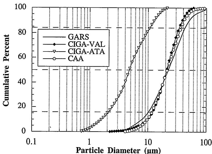
Figure 4.4. Cumulative size distributions of the GARS-4, CIGA-ATA, CIGA-VAL, and CAA aluminum powders.
