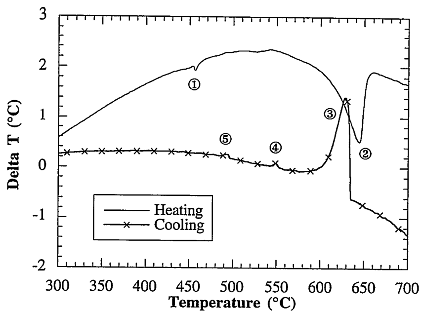
a. Overall DTA trace of Al-Cu-Mg aluminum alloy powder.
