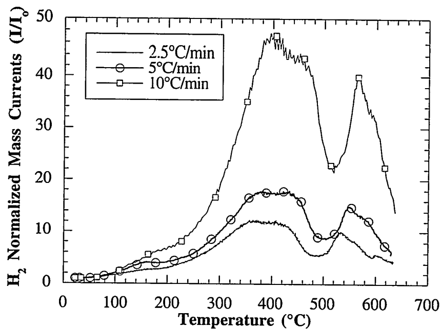
Figure 4.17. The effect of different heating rates during a QMS examination of CAA aluminum powder at a constant sample density of 92.3%.
