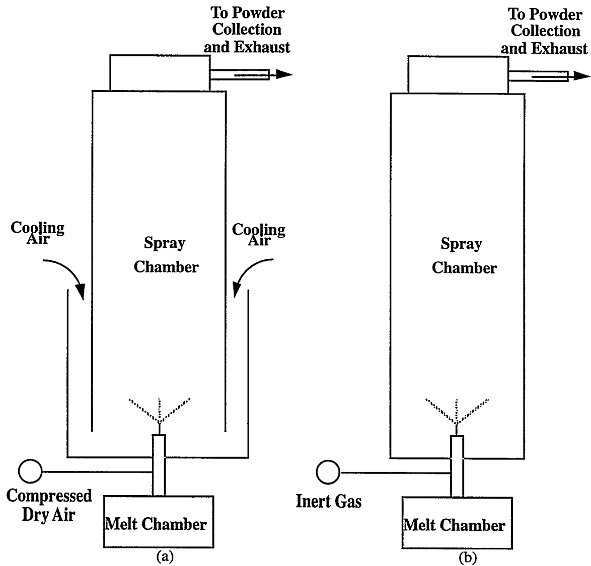
Figure 2.1. a) Schematic of vertically upward atomization system used by Alcoa for CAA of aluminum powders [2]. b) Schematic of vertically upward atomization system used by Alcan-Toyo America for CIGA-ATA of aluminum powders [2, 6].
