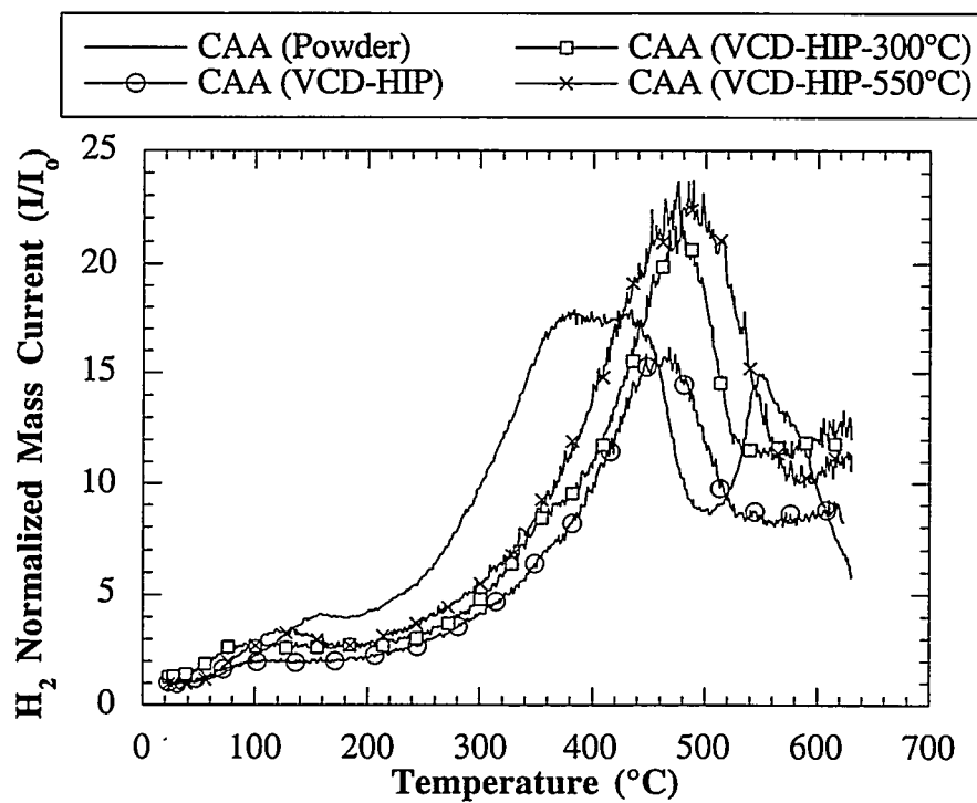
Figure 4.60. Effect of heat treating temperature on CIP-VCD-HIP CAA powder samples.
