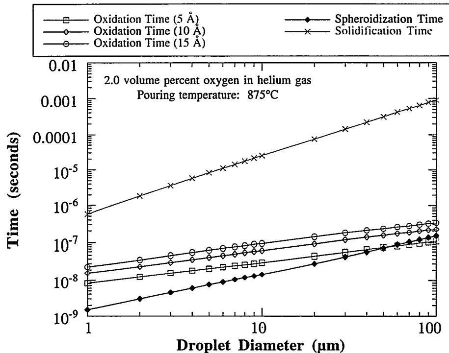
Figure 5.10. Comparison of atomization time scales for aluminum powder helium gas atomized with 2.0 volume percent oxygen in the atomization gas.
