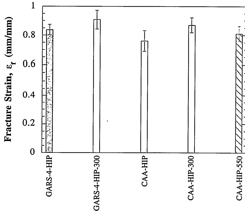
Figure 4.69. The effect of heat treatment on the fracture strain properties of the GARS-4 and CAA aluminum powders consolidated by the CIP-VCD-HIP route.
