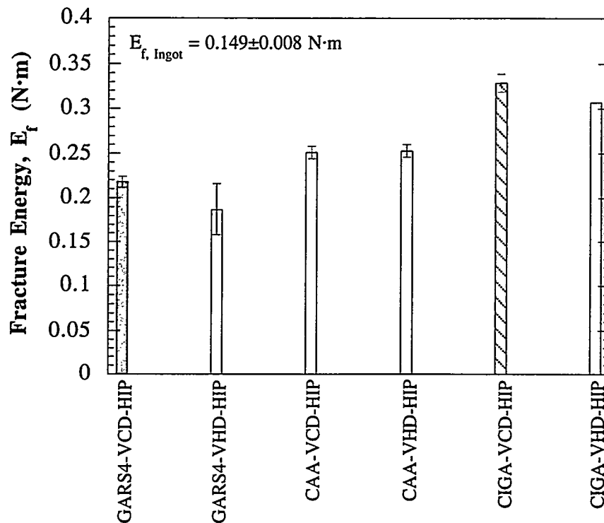
Figure 4.65. Fracture energy results from punch testing the GARS-4, CAA, and CIGA-ATA aluminum powders consolidated by CIP-VCD-HIP and CIP-VHD-HIP routes.
