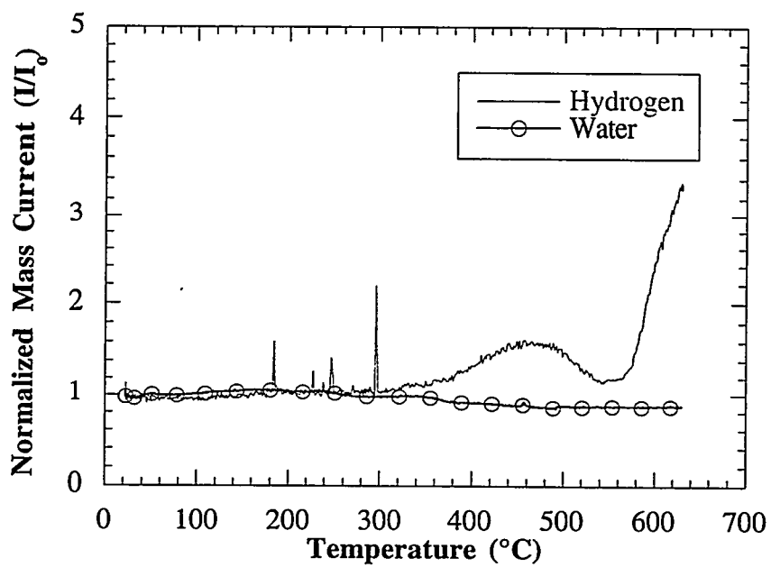
Figure 4.9. QMS results of 99.999% Alcoa aluminum ingot heated at 5^{\circ}\text{C}/\text{min} .
