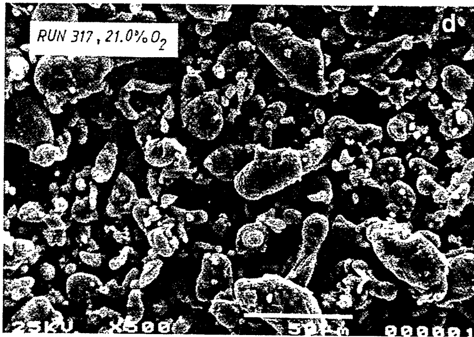
Figure 5.1. SEM micrograph of aluminum powder produced by gas atomization with a mixture of 21.0 volume percent oxygen in nitrogen gas [13].
