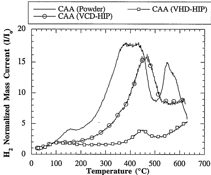
Figure 4.56. QMS results of the CAA powder samples comparing the as-atomized powder to the CIP-VHD-HIP and CIP-VCD-HIP consolidated samples.
