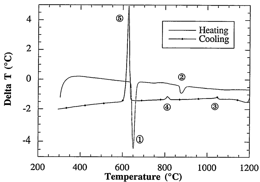
Figure 4.31. DTA of Al-Ti-Y alloy powder in the as-atomized condition.
