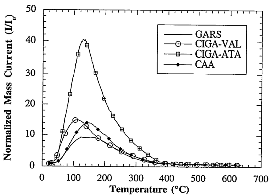
Figure 4.15. Comparison of the water evolution from the GARS, CIGA-VAL, CIGA-ATA and CAA pure aluminum powders during the QMS experiments.
