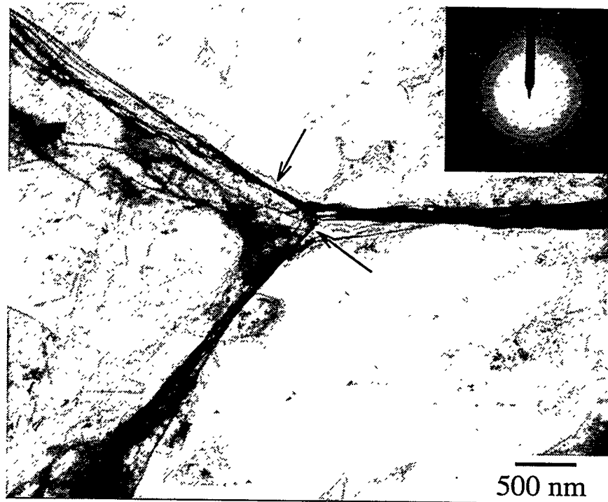
Figure 4.23. TEM micrograph and SAD pattern of the oxide film on CAA aluminum powder. The arrows indicate the oxide thickness measurements.
