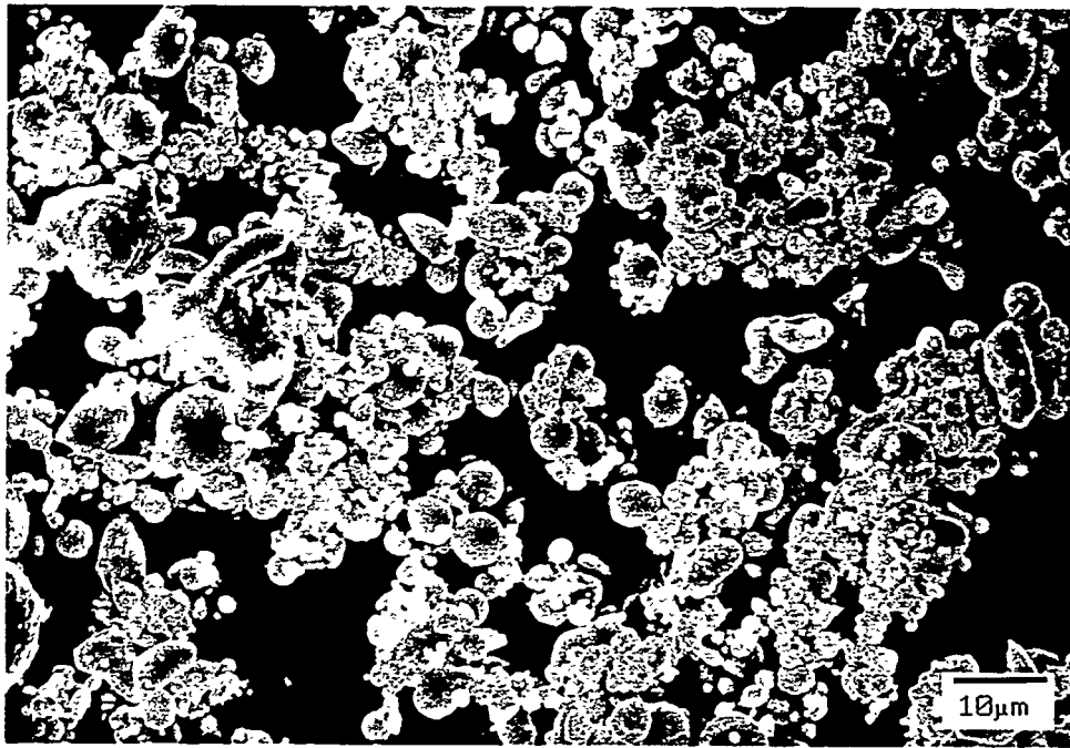
Figure 4.2. SEM micrograph of the as-atomized CIGA-ATA pure aluminum powder.
