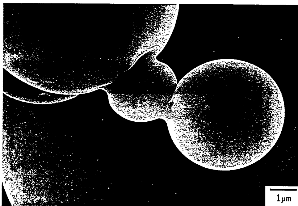
Figure 4.49. SEM micrograph of the GARS aluminum powder air sintered at 300°C for 24 hours.
