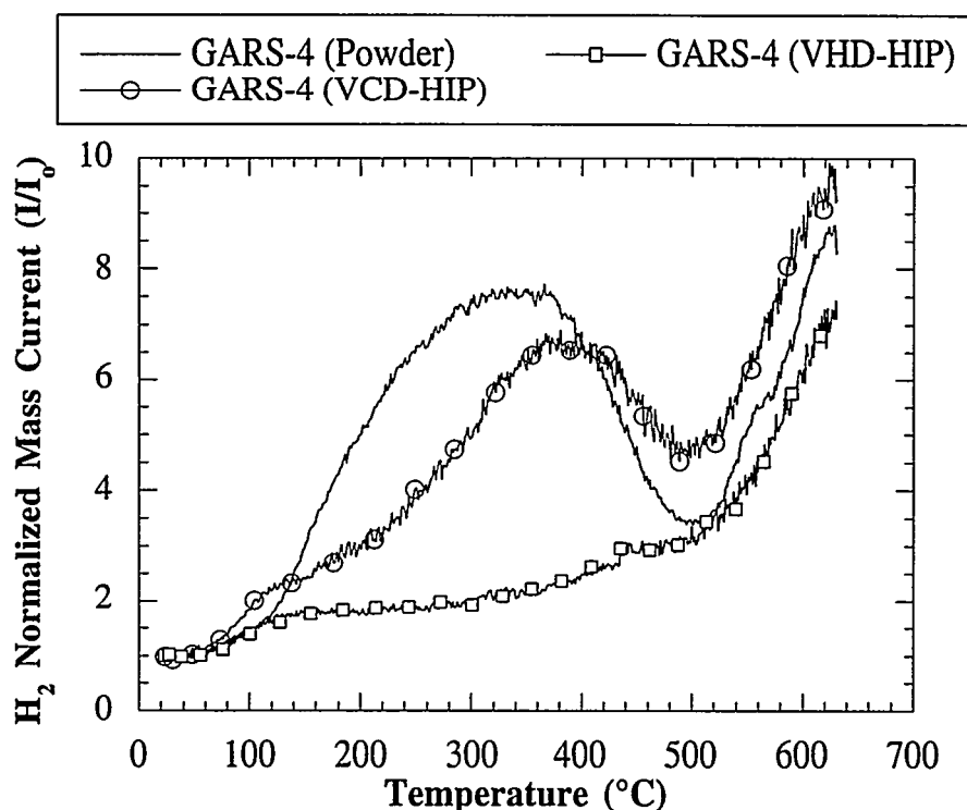
Figure 4.57. QMS results of the GARS-4 powder samples comparing the as-atomized powder to the CIP-VHD-HIP and CIP-VCD-HIP consolidated samples.
