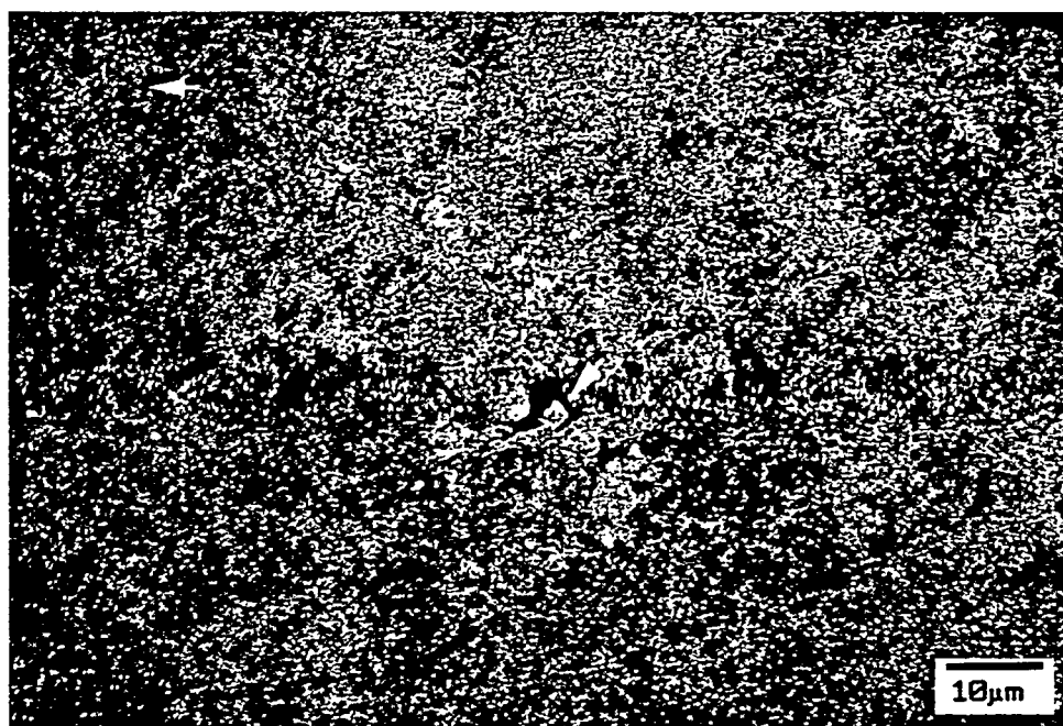
Figure 4.52. SEM micrograph showing the CIP-VCD-HIP microstructure of the CAA aluminum powder. The white arrows indicate the residual porosity in the sample.
