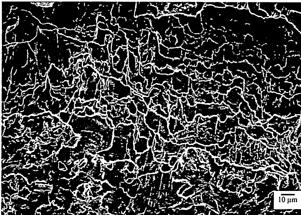
Figure 4.63. SEM micrograph showing the typical fracture surface formed during punch testing of the aluminum powder punch test coupons.
