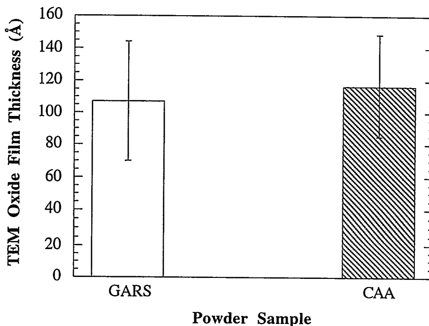
Figure 4.25. TEM measurements of the oxide film thickness on the GARS-8 and CAA pure aluminum powders
