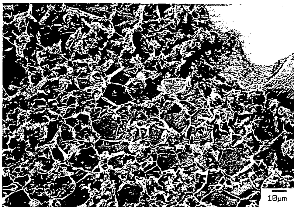
Figure 4.28. SEM micrograph of CAA aluminum powder TEM sample in Figure 4.23.
