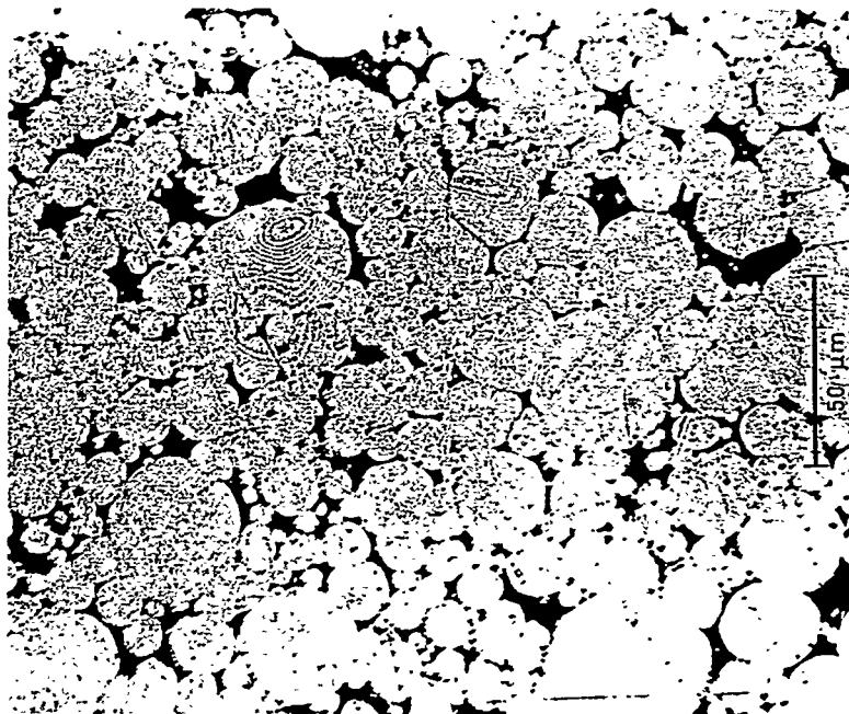
Figure 4.51. Optical micrograph of the as-polished, unetched, CIP microstructure of the GARS aluminum powder.
