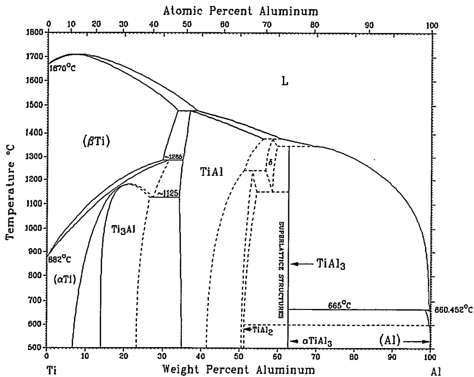
Figure 4.33. Aluminum-titanium phase diagram [83].
