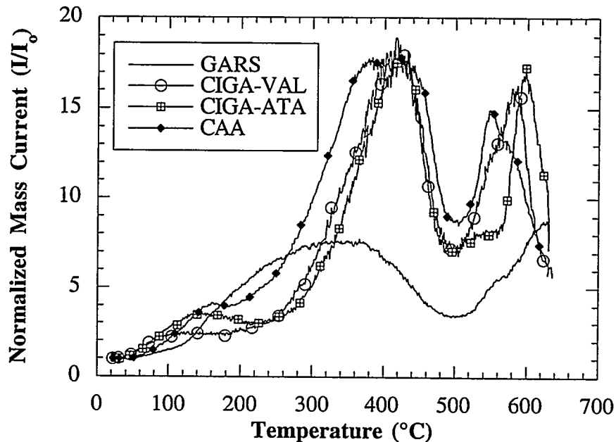
Figure 4.16. Comparison of the hydrogen evolution from the GARS, CIGA-VAL, CIGA-ATA, and CAA pure aluminum powders during the QMS experiments.
