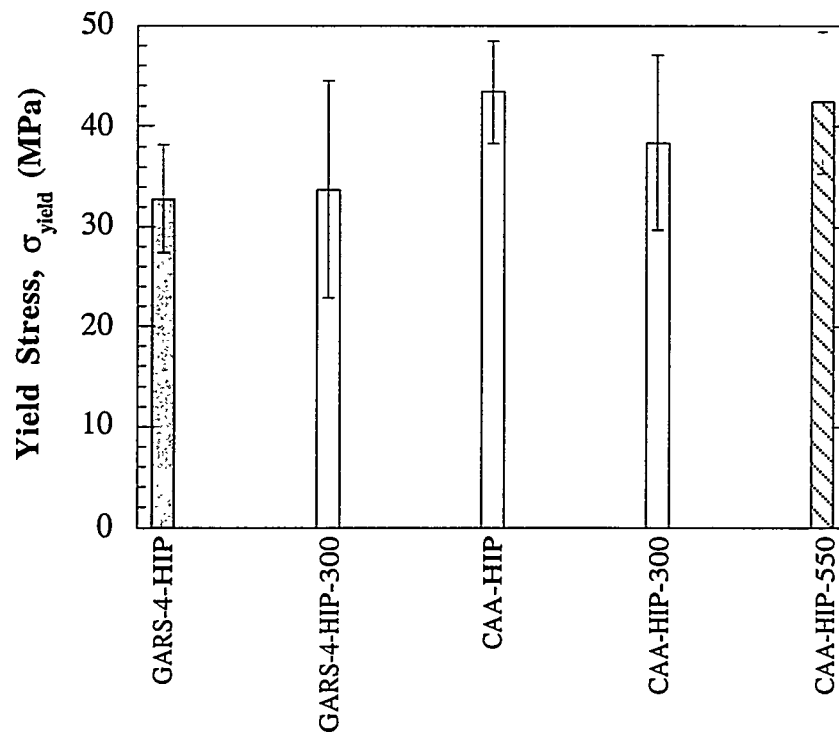
Figure 4.67. The effect of heat treatment on the yield stress properties of the GARS-4 and CAA aluminum powders consolidated by the CIP-VCD-HIP route.
