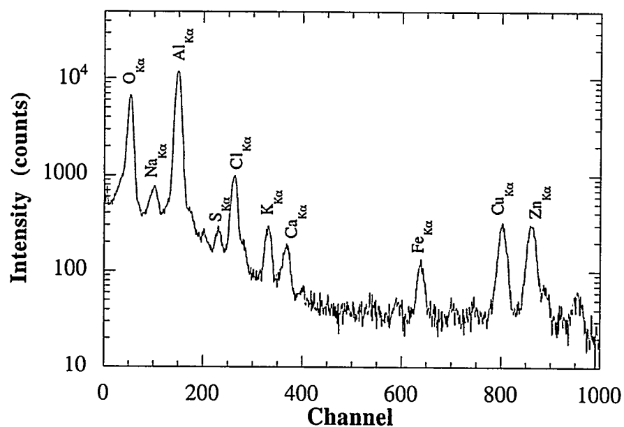
Figure 4.26. EDS spectra of the oxide film on CAA aluminum powder.
