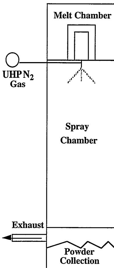
Figure 3.1. Schematic of the gas atomization system used at the Ames Laboratory.
