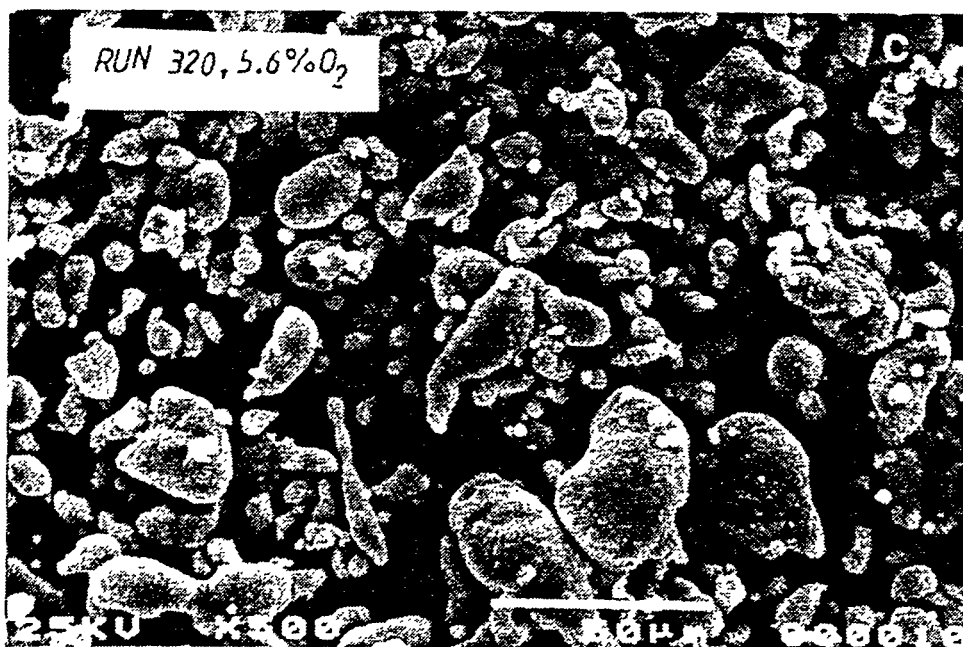
Figure 5.4. SEM micrograph of aluminum powder produced by gas atomization with a mixture of 5.6 volume percent oxygen in nitrogen gas [13].
