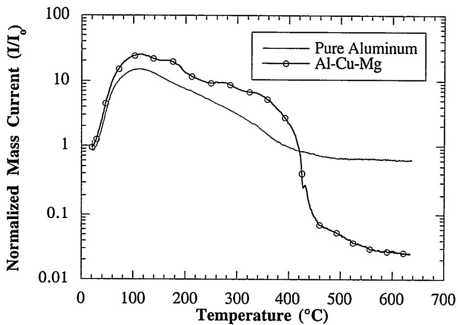
Figure 4.35. Comparison of the QMS water spectra of a SSA pure aluminum powder and a SSA Al-Cu-Mg aluminum alloy powder heated at 5°C per minute.
