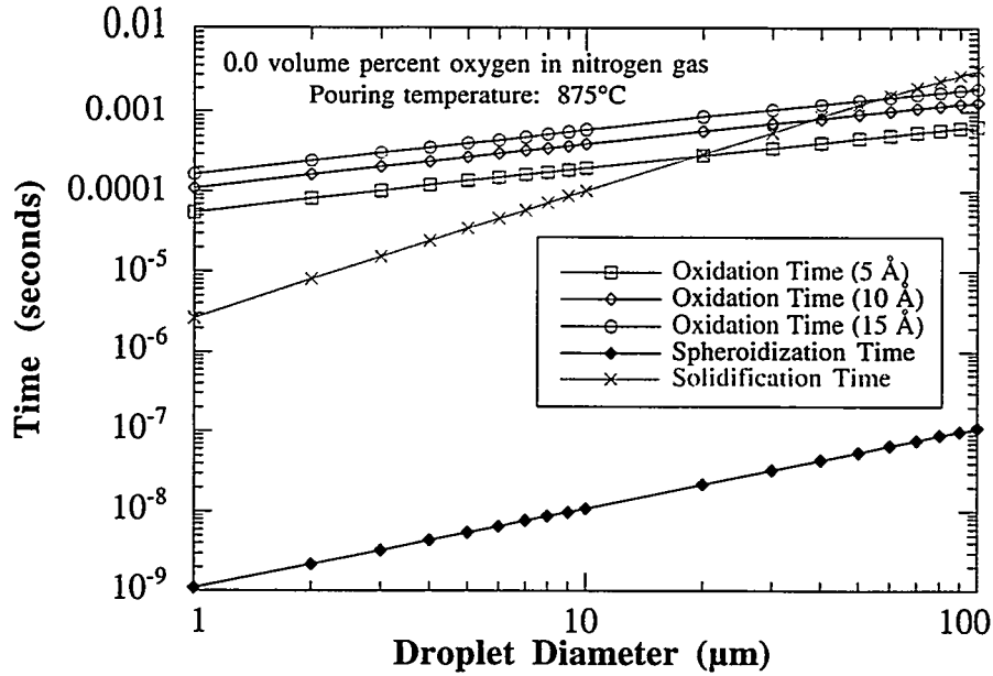
Figure 5.6. Atomization time scale comparison for molten aluminum gas atomized with a gas mixture of 0.0 volume percent oxygen in nitrogen gas.
