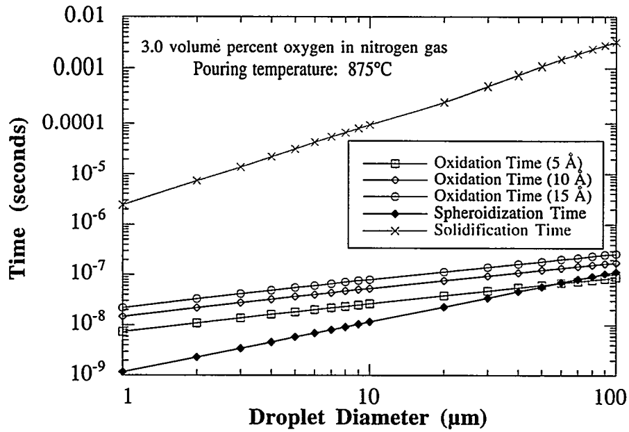
Figure 5.7. Comparison of atomization time scales for aluminum powder nitrogen gas atomized with 3.0 volume percent oxygen in the atomization gas.
