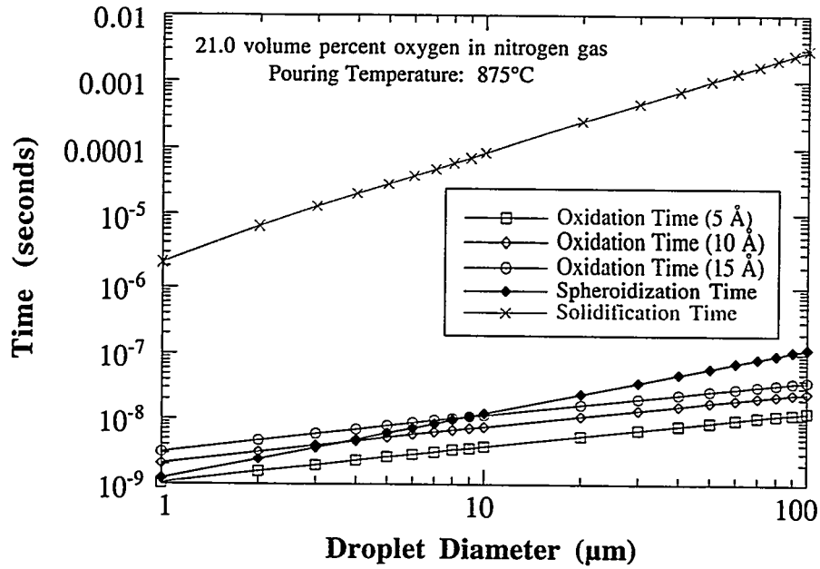
Figure 5.5. Atomization time scale comparison for molten aluminum gas atomized with a gas mixture of 21.0 volume percent oxygen in nitrogen gas.
