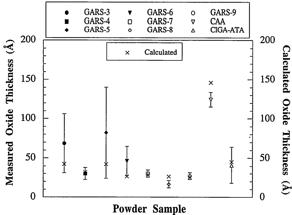
Figure 5.13. Comparison of oxide film thicknesses predicted from the model presented in the text and as measured by AES.
