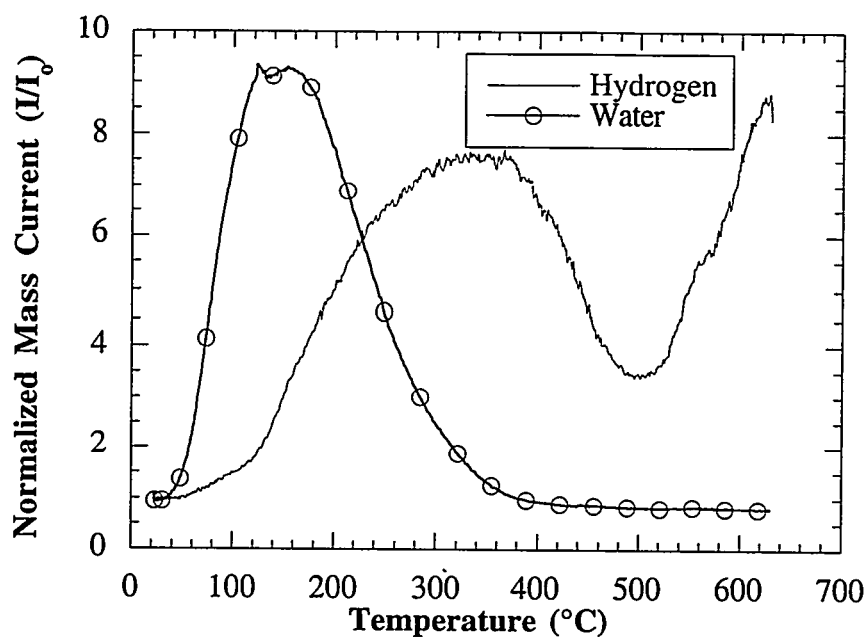
Figure 4.14. Representative QMS plot of GARS-4 aluminum powder heated at 5°C/min.
