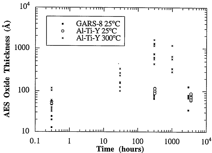
Figure 4.42. AES oxide thickness measurements for aluminum based powders exposed to ambient air at room temperature, nominally 25°C, and 300°C.
