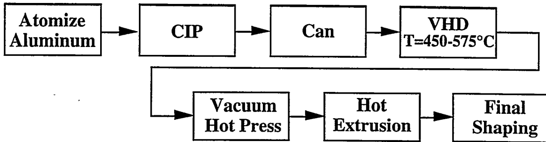
Figure 2.3. Conventional consolidation sequence for aluminum powders used in aerospace applications [1].
