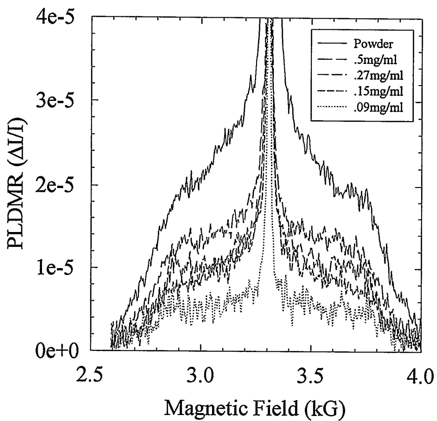
Figure 4.10 The full-field PLDMR of films and frozen toluene solutions of selected concentrations of DBO-PPE at T=15\text{K} .
