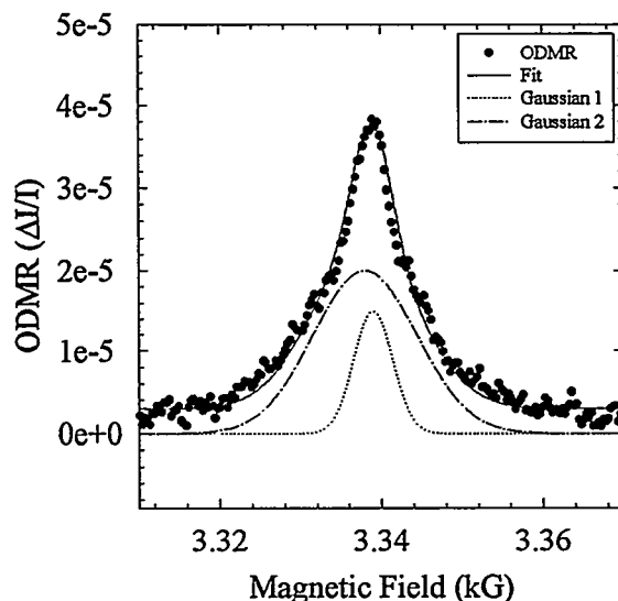
Figure 1.3 Typical spin- \frac{1}{2} enhancing PLDMR spectra. This particular spectrum comes from poly( p -phenylene)-type ladder (LPPP) polymers (described below).
