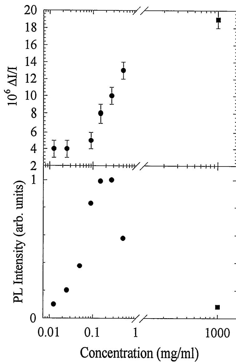
Figure 4.11 The amplitude \Delta I/I of the half-field resonance and the PL intensity I vs. concentration of DBO-PPE in toluene at 15K. The values for DBO-PPE powder are shown at the equivalent concentration of 1000mg/ml.
