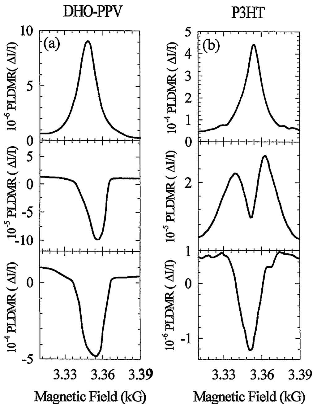
Figure 2.7 (a) DHO-PPV at (top to bottom) \lambda_{\text{ex}} =458, 430, and 406nm. (b) P3HT at (top to bottom) \lambda_{\text{ex}} =458, 353, and 308nm. Microwave power for all spectra was 1400mW except for the spectra taken at 458nm, at which it was 40mW. Temperature was set at 10K for all spectra.
