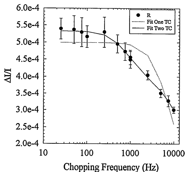
Figure 4.7 Modulus of the g=2 PLDMR signal of DBO-PPE powder at 15K.
