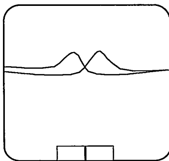
Figure A.3 Properly adjusted fluxmeter.
