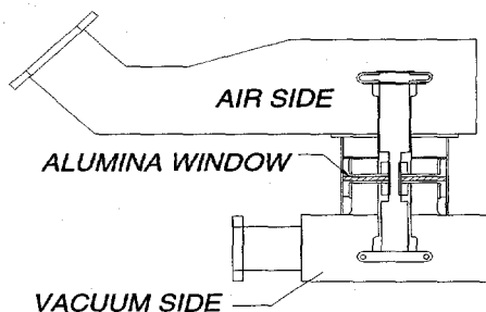
Figure 4: RFQ coaxial window.
