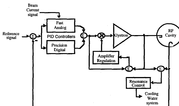
Figure 6: LLRF control system.
