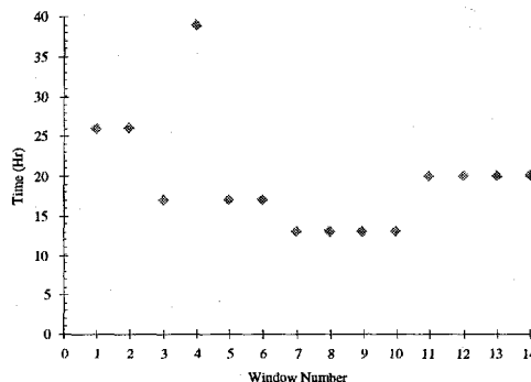
Figure 5: RFQ vacuum window conditioning time.
