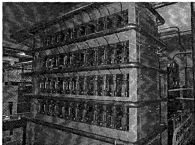
Figure 3: Power Column For IGBT Power Supply
