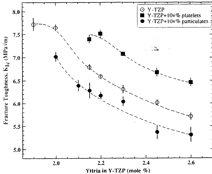
Figure 6. Effect of \text{Y}_2\text{O}_3 content on the fracture toughness of Y-TZP monoliths, Y-TZP+10v% \text{Al}_2\text{O}_3 (platelet) composites and Y-TZP+10v% \text{Al}_2\text{O}_3 (particulate) composites.
