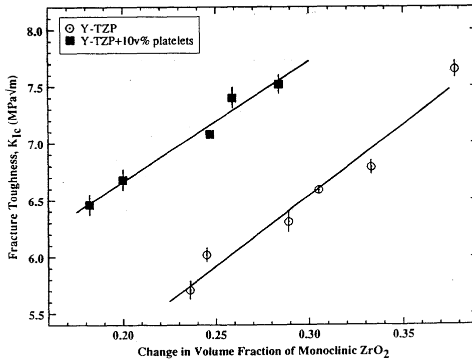
Figure 7. Correlations of fracture toughness and change in monoclinic content on the fracture surface for Y-TZP monoliths and Y-TZP+10v% \text{Al}_2\text{O}_3 (platelet) composites.
