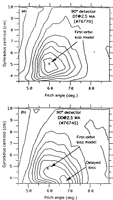
Fig. 2: Pitch angle vs. gyroradius distributions of alpha loss at I_p = 2.5 MA for similar DT and DD discharges at R = 2.52 m. In DT the pattern is consistent with first-orbit loss when the instrumental broadening effects are included. The delayed loss in DD which is not seen in DT is most likely due to collisional losses of 1 MeV tritons in DD.
