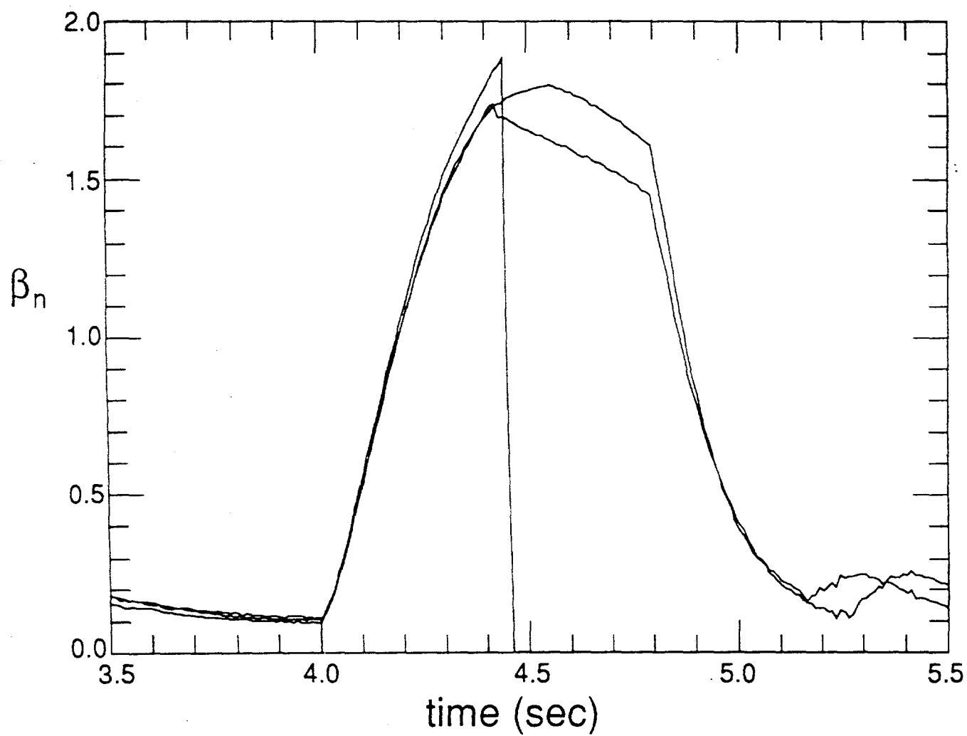
Figure 1 Time evolution of \beta_n for three of the highest fusion power D-T shots.
