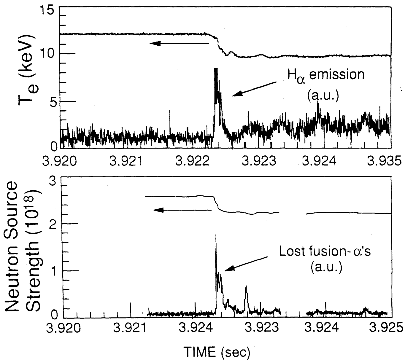
Figure 4 Central electron temperature, edge H_\alpha , global neutron rate and alpha loss rate through a minor disruption.
