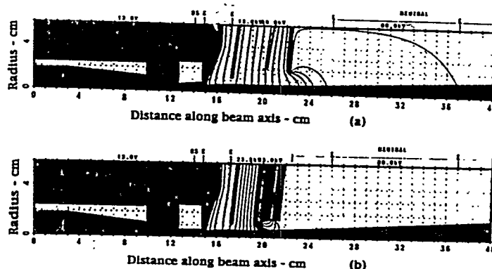
Fig. 5 Trajectories and equipotentials for the 16-mA production beam with the present accelerating column (a) and for a 40-mA beam with a high gradient tetrode column (b).
