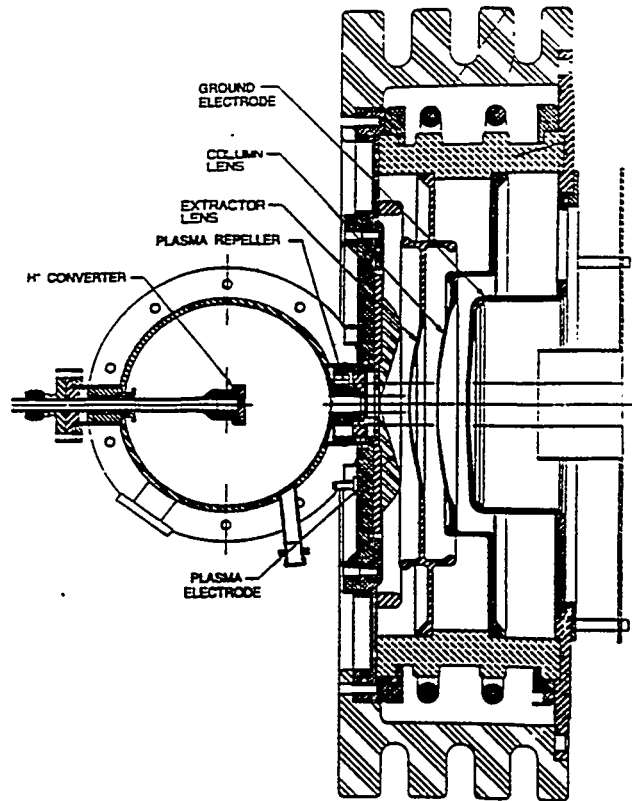
Fig. 1. Layout of the LANL converter ion source with the present accelerating column.
