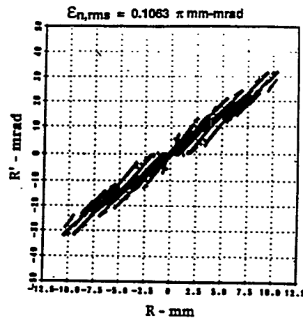
Fig. 3. Calculated emittance distribution of a 16-mA H^- beam at the column exit for 12-kV extraction voltage.
