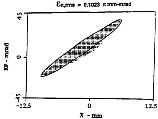
Fig. 2. Horizontal emittance scan of a 16-mA H^- beam at the column exit with 12-kV extraction voltage.
