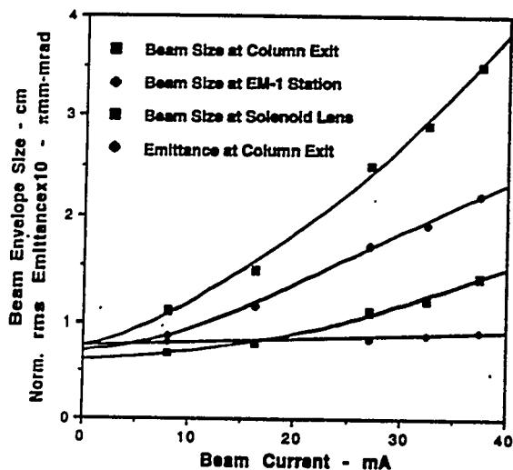
Fig. 4. Beam emittance at the column exit and beam sizes in the LEBT as a function of extracted current.
