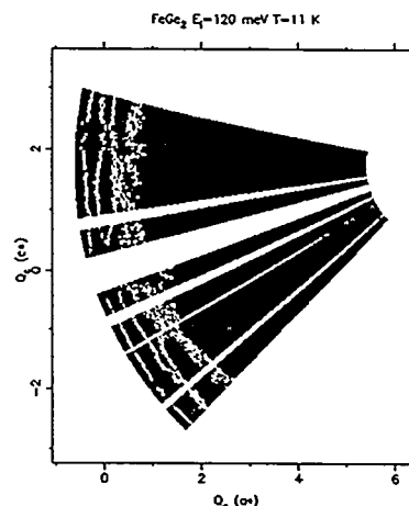
Figure 3: Spin wave and phonon scattering from FeGe 2 at 11 K for energy transfers from -10 to 120 meV (left to right) projected onto the ( Q_a, Q_c ) plane.
