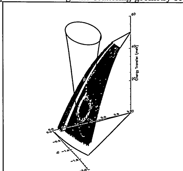
Figure 2: Time of flight spectra obtained on HET from the CMR compound \text{La}_{0.7}\text{Pb}_{0.3}\text{MnO}_3 in the ferromagnetic phase at T=10 K. The intersection of the dispersion surface extracted from fits to the data with the neutron trajectories in (\mathbf{Q}, \omega) space is shown schematically.
