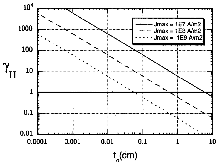
Fig. 1 Equation [1] plotted for various values of J_{\max} with B_r=1.2 T, \mu_m=1.05 , \alpha=0.75 , and \mu_0=4\pi(10)^{-7} Hy/m. This plot is intended only as a rough gauge of the trade-off involved between a permanent magnet and a coil in generating a static magnetic field.
