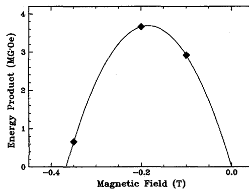
Fig. 6 Data from the smallest permanent magnet which was measured
