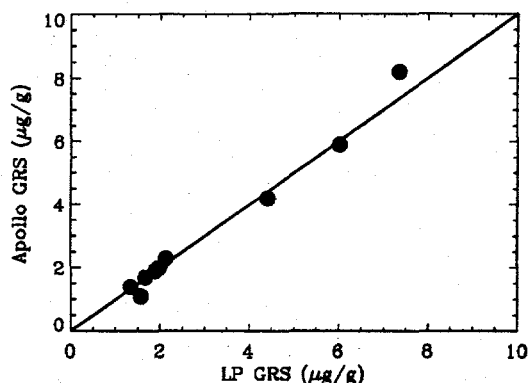
Figure 2: Comparison of the absolute thorium abundance measured by the LP GRS to the absolute thorium abundance measured by the Apollo 15 and 16 GRS for various Apollo and Luna landing sites.
