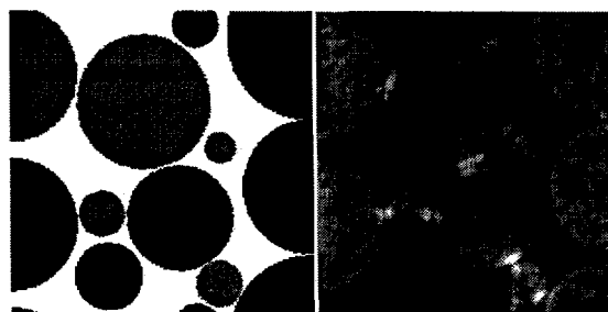
FIGURE 7. "LOCKED" STATE IN THE SMALL GRANULAR SHEAR PROBLEM.
