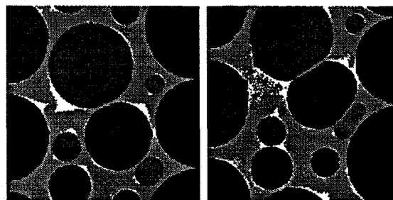
FIGURE 8. INTERMEDIATE AND FINAL STATES IN THE SHEARING OF GRAINS WITH BINDER.
