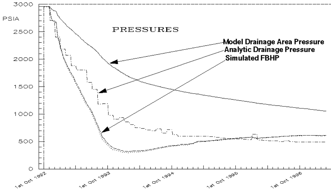
Fig. 19. Analytical vs. simulated pressure response for initial k_{rg} , NDP Well #1.
