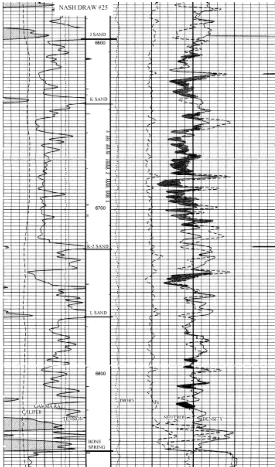
Fig. 3. Log from Well 25 showing poor pay quality.
