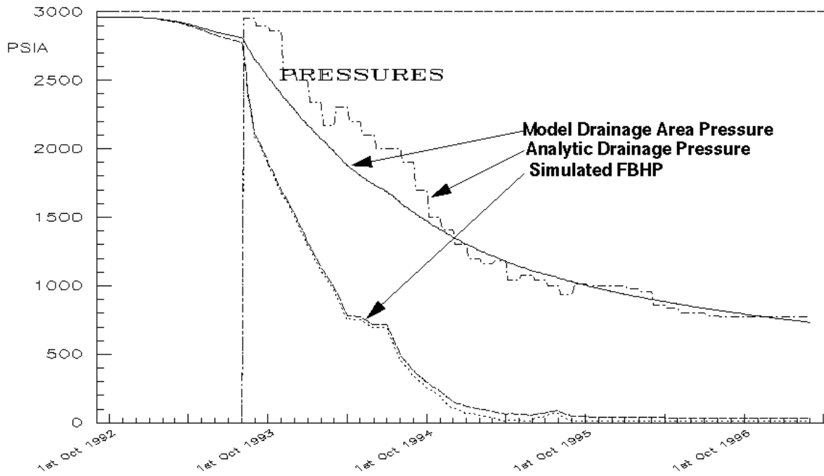
Fig. 14. Pressure response for trans_{fracture} = 2.0 darcy-ft per cp, NDP Well #14.
