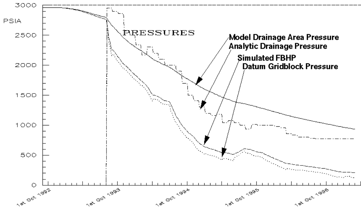
Fig. 24. Pressure response with enhanced matrix transmissibility, NDP Well #14.
