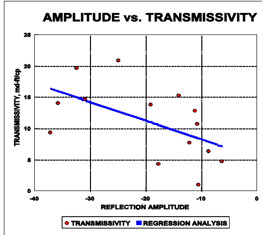
Fig. 6. "L" Zone seismic amplitude vs. transmissivity.
