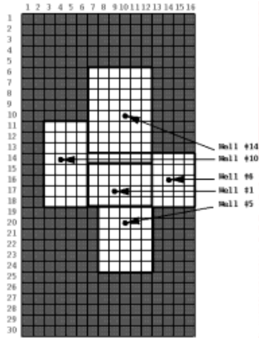
Fig. 13. Well drainage areas in the simulation model. (Each cell occupies an area of approximately one acre).
