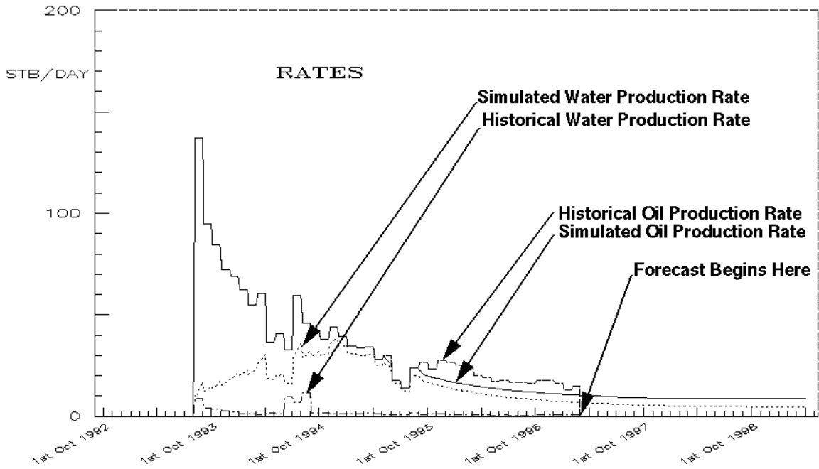
Fig. 30. Rate response for case 1, NDP Well #14.
