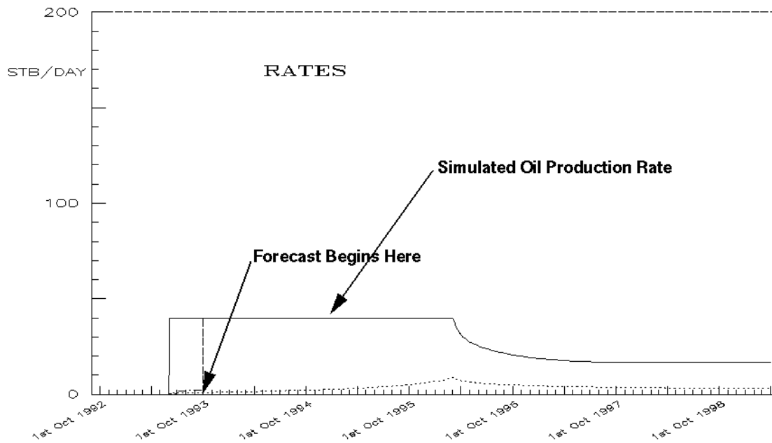
Fig. 33. Oil production for case 2, NDP Well #6.
