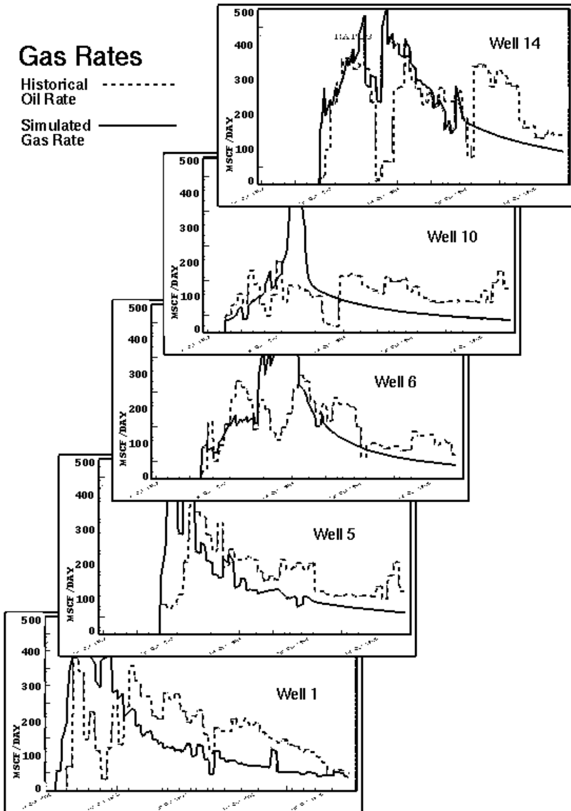
Fig. 27. Gas production rate match for Nash Draw pilot area wells.
