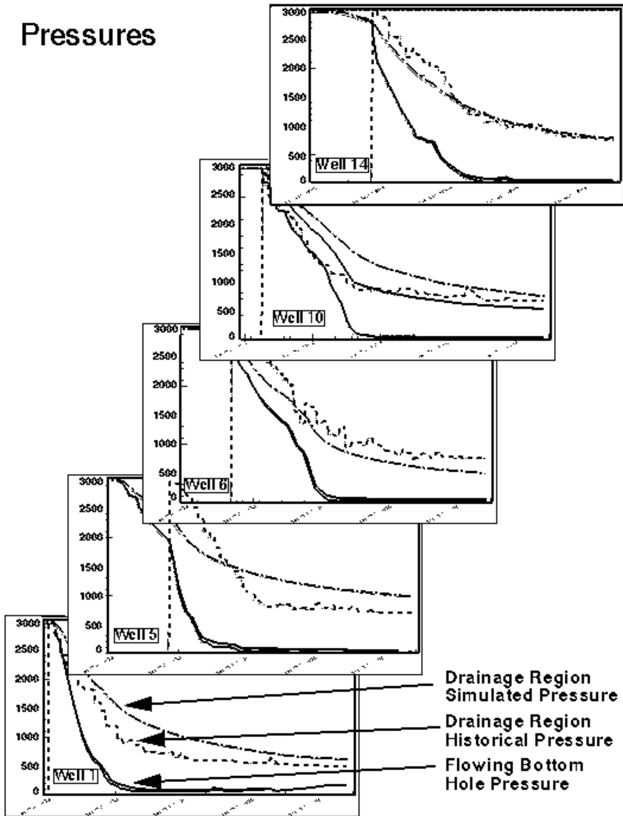
Fig. 25. Pressure match for Nash Draw pilot area wells.
