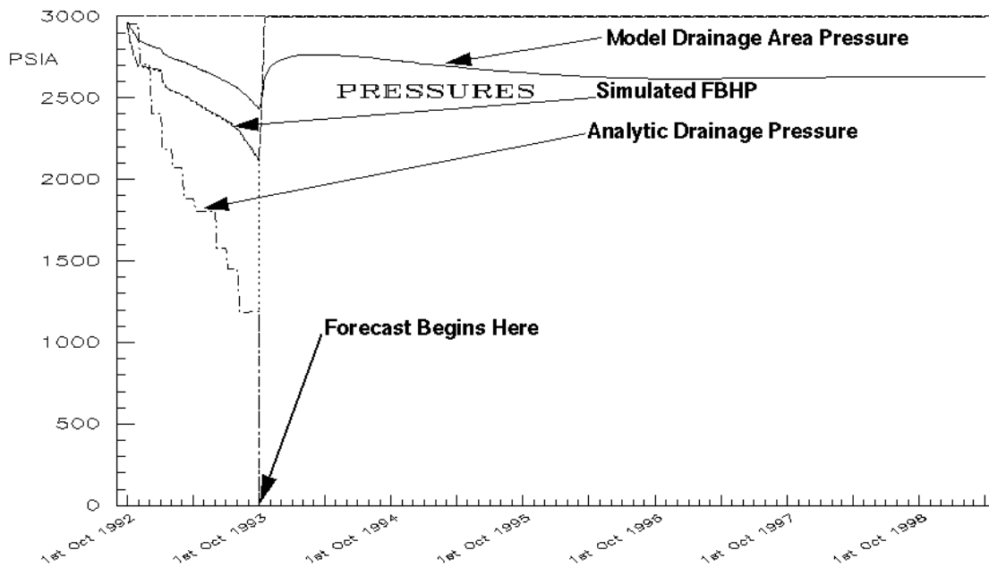
Fig. 31. Pressure response for case 2, NDP Well #1.
