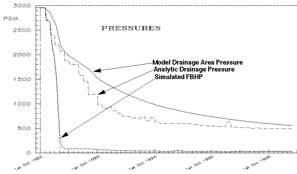
Fig. 18. Simulated pressure response with original data, NDP Well #1.
