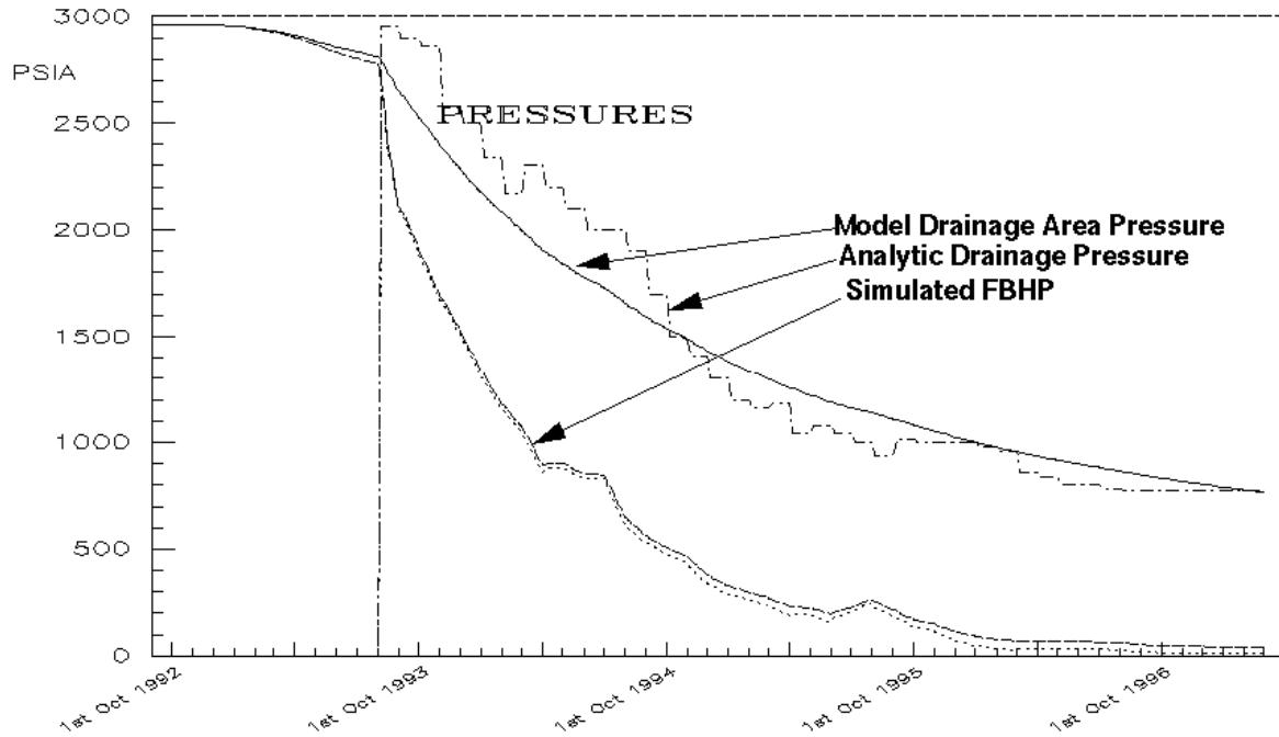
Fig. 15. Pressure response for \text{trans}_{\text{fracture}} = 0.5 darcy-ft per cp, NDP Well #1.
