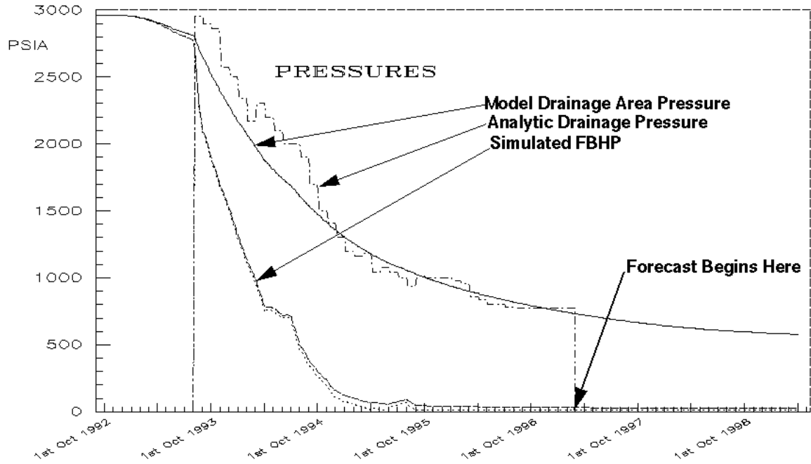
Fig. 28. Pressure response for case 1, NDP Well #1.
