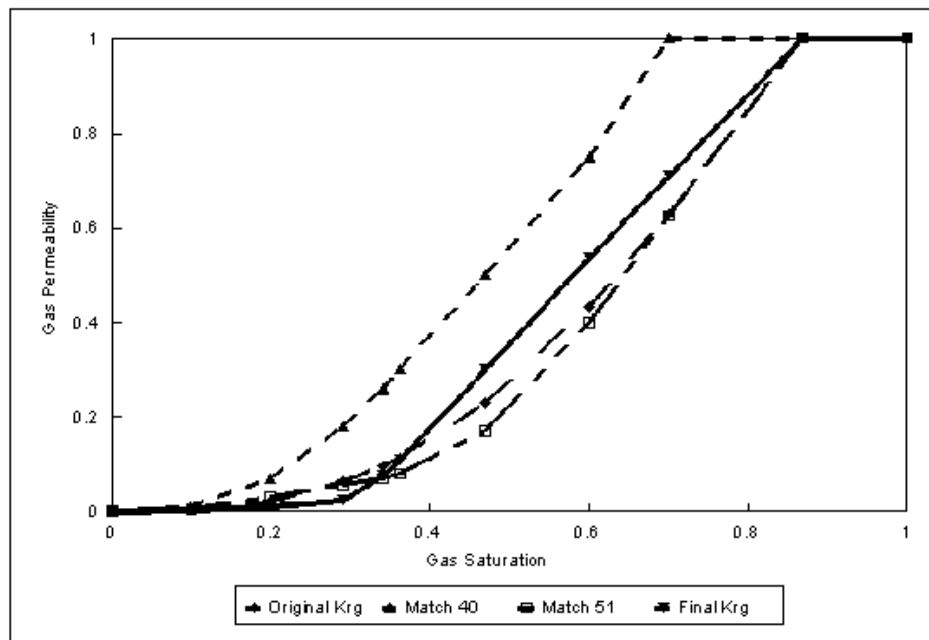
Fig. 22. The envelope of k_{rg} curves investigated during model validation.
