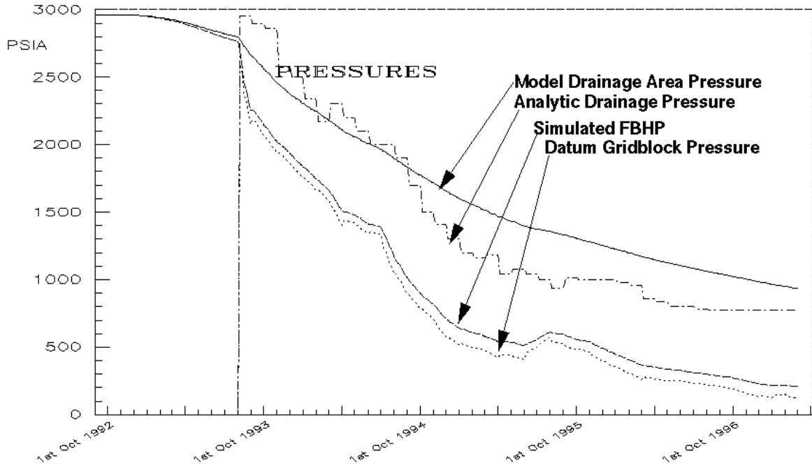
Fig. 23. Pressure response with original reservoir description, NDP Well #14.
