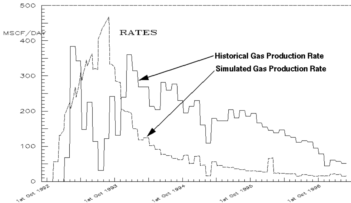
Fig. 20. Gas production for initial k_{rg} , NDP Well #1.
