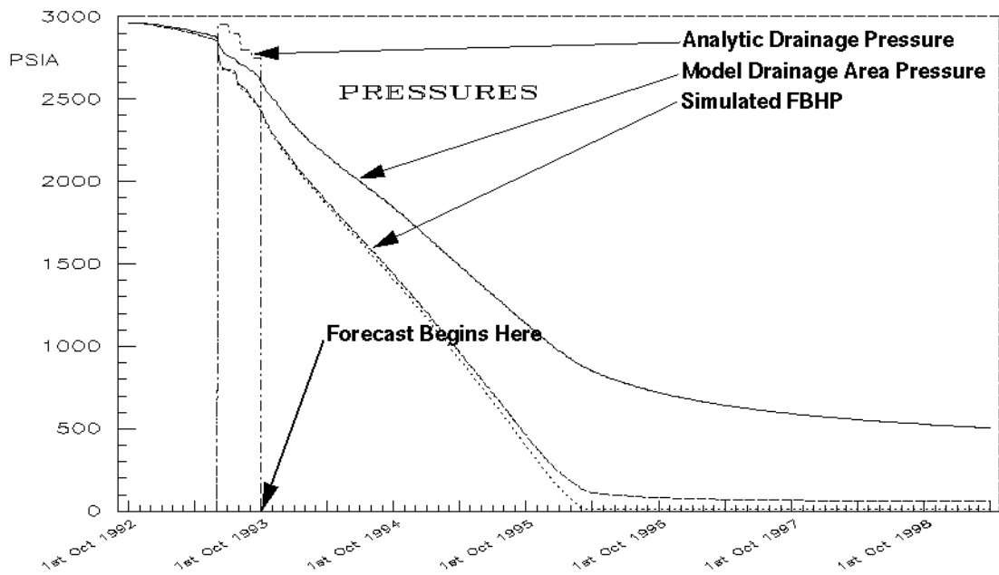
Fig. 32. Pressure response for case 2, NDP Well #6.
