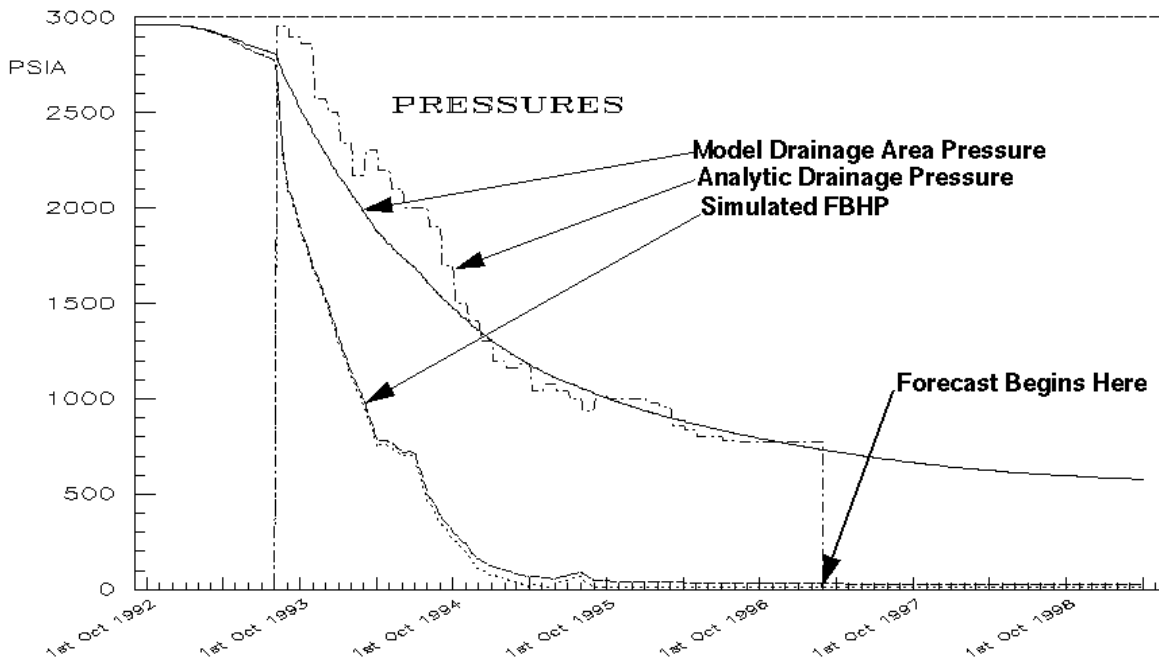
Fig. 29. Pressure response for case 1, NDP Well #14.
