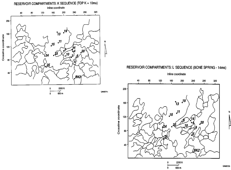
Fig. 7. Reservoir compartmentalization.
