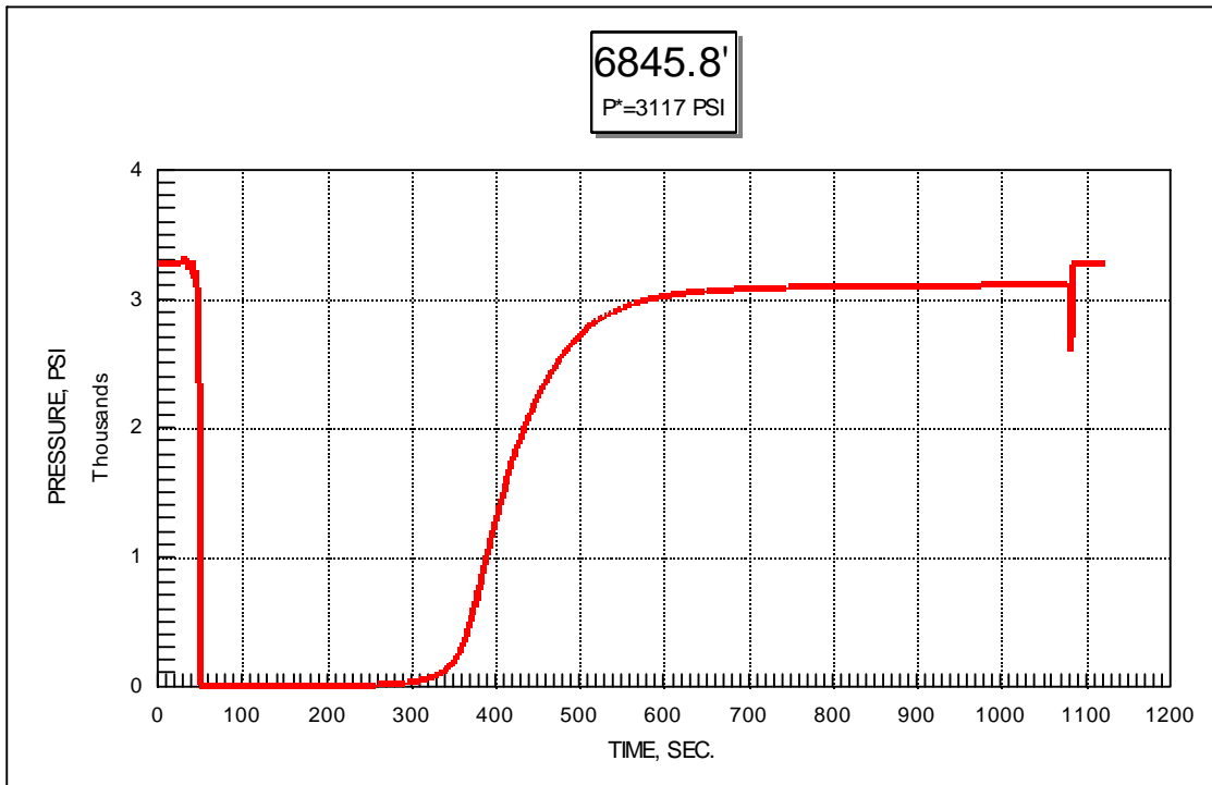
Fig. 9. Continuity test with RFT tool.
