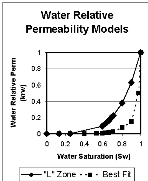
Fig. 16. Initial and "best fit" values of k_{rw} .
