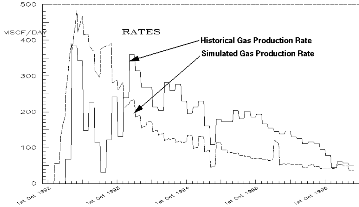
Fig. 21. Gas production after history matching adjustments, NDP Well #1.
