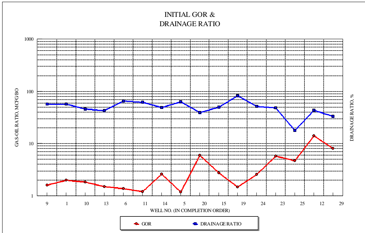
Fig. 10. Initial gas-oil ratio and drainage ratio.
