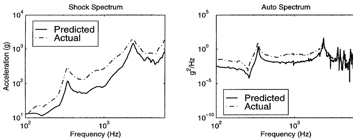
Figure 8 Base of component response (location B)
