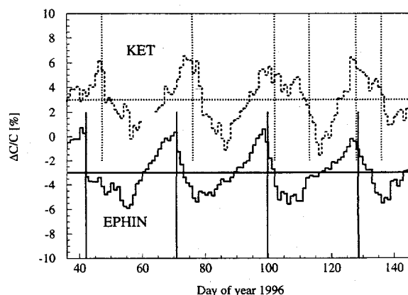
Figure 3. Daily averaged detrended >100 MeV proton count rates. EPHIN and KET data are the solid and dashed lines, respectively. The vertical lines mark the onset of individual RCRDs seen by SOHO at Earth and Ulysses.
