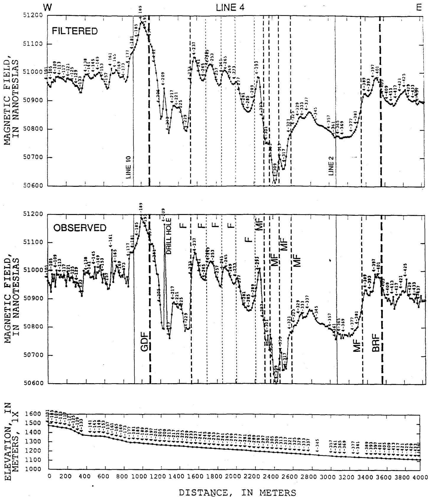
FIGURE 5.—Observed and filtered magnetic profile of line 4. See figure 4 for explanation.
