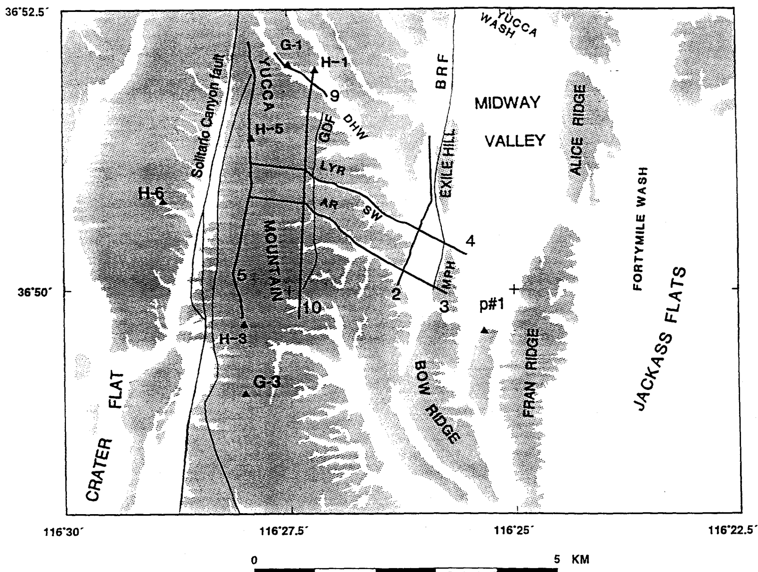
FIGURE 1.—Index map of the study area showing locations of magnetic profiles across the central block of Yucca Mountain. White area, Quaternary alluvium and colluvium; Shaded area, Tertiary volcanic rocks; Triangle, drill hole; AR, Antler Ridge; BRF, Bow Ridge fault; DHW, Drill Hole Wash; GDF, Ghost Dance fault; LYR, Live Yucca Ridge; MPH, Muck Pile Hill; SW, Split Wash. Geology modified from Frizzell and Shulters (1990).
