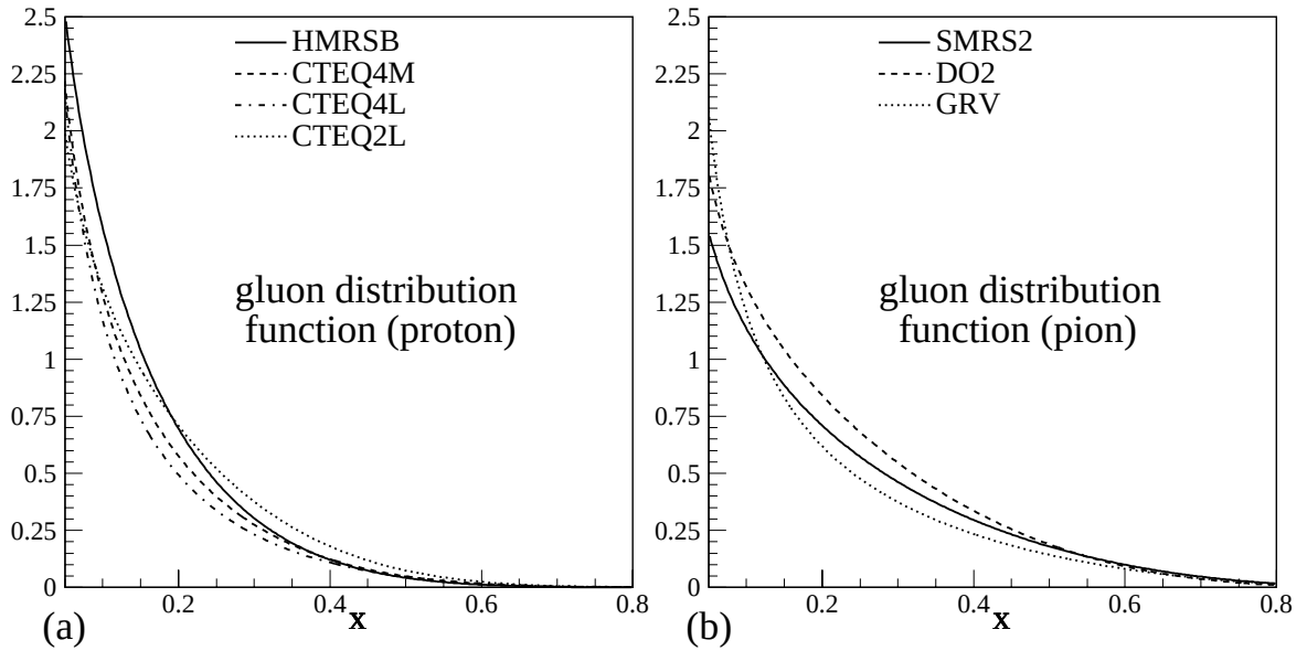
Fig. 6.9.— Plots of gluon distribution functions at Q^2=5 \text{ (GeV/c)}^2 in the range 0.05 < x < 0.8 for protons (a) and pions (b) from several PDF sets. The PDF data are obtained from the CERN program PDFLIB [3].
