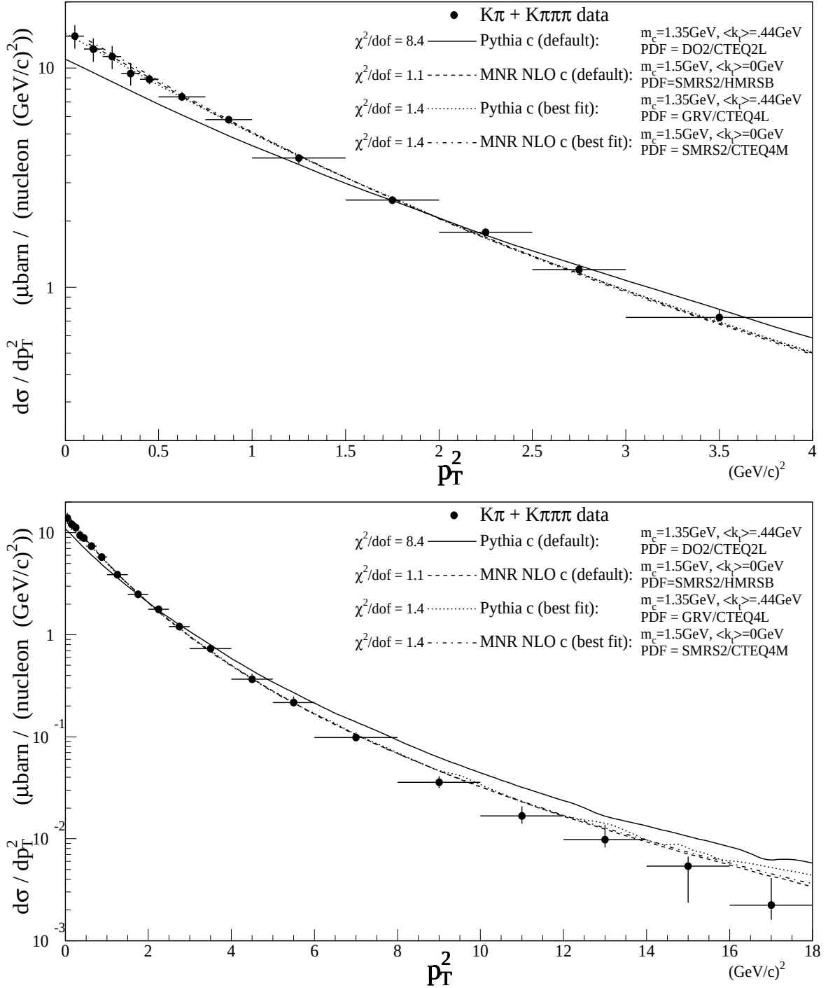
Fig. 6.11.— Comparison of the D^0 p_T^2 distribution to theory predictions. The theory predictions are obtained for charm quarks using two different parameters, the default parameters and the set which best fits the x_F and p_T^2 data. The distributions are normalized to obtain the best fit to the data.
