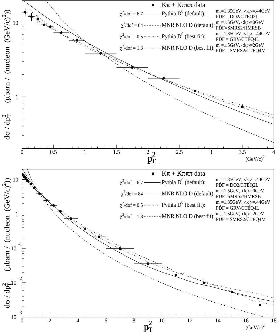
Fig. 6.13.— Comparison of the D^0 p_T^2 distribution to theory predictions. The MNR NLO (PYTHIA/JETSET) predictions are obtained for D ( D^0 ) mesons using two different parameters, the default parameters and the set which best fits the x_F and p_T^2 data. The distributions are normalized to obtain the best fit to the data.
