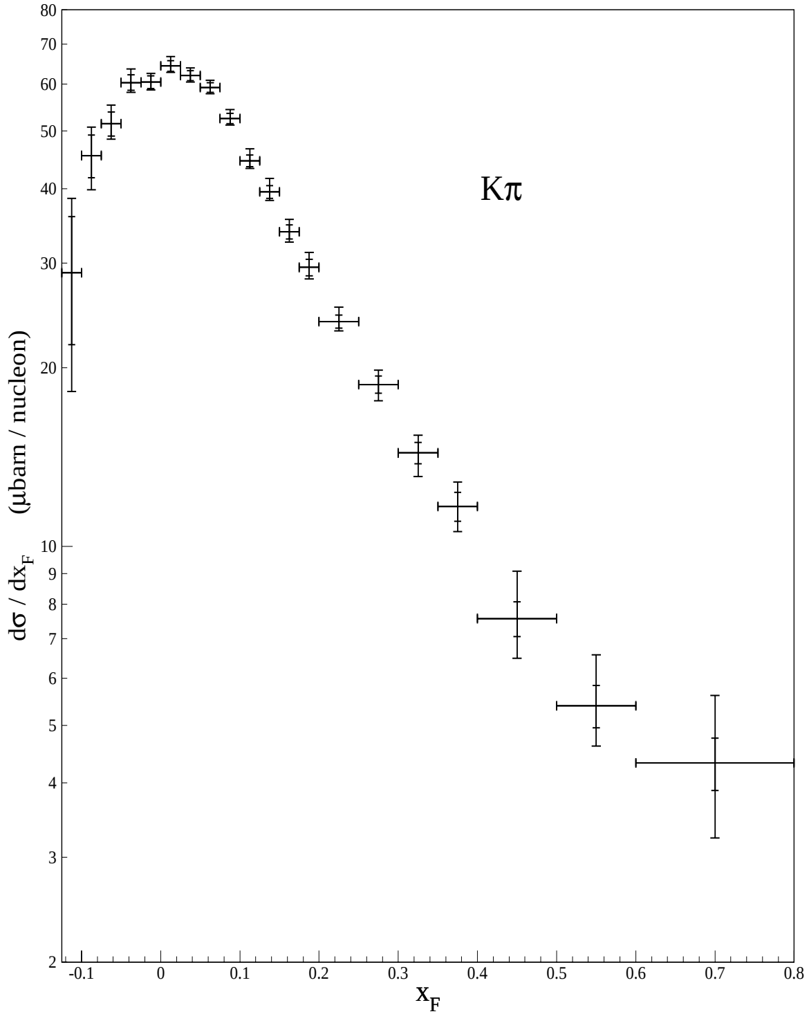
Fig. 6.3.— K\pi fully corrected x_F differential cross section. The inner error bars show the statistical errors only. The outer error bars show the quadratic sum of the statistical errors and the K\pi -only systematic errors.
