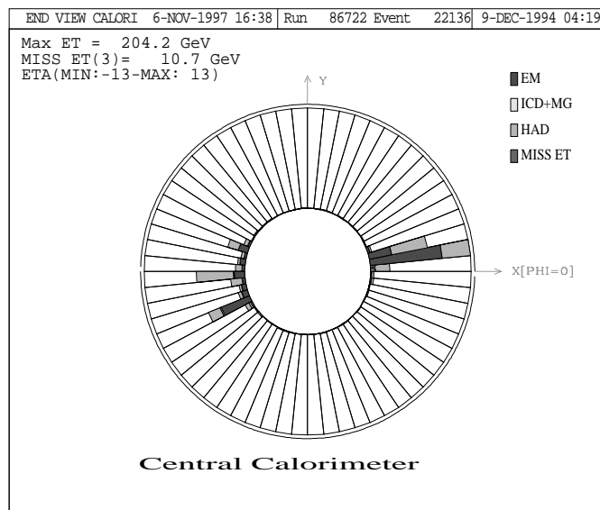
Figure 3.2: Calorimeter end view for the same D\bar{D} event.
