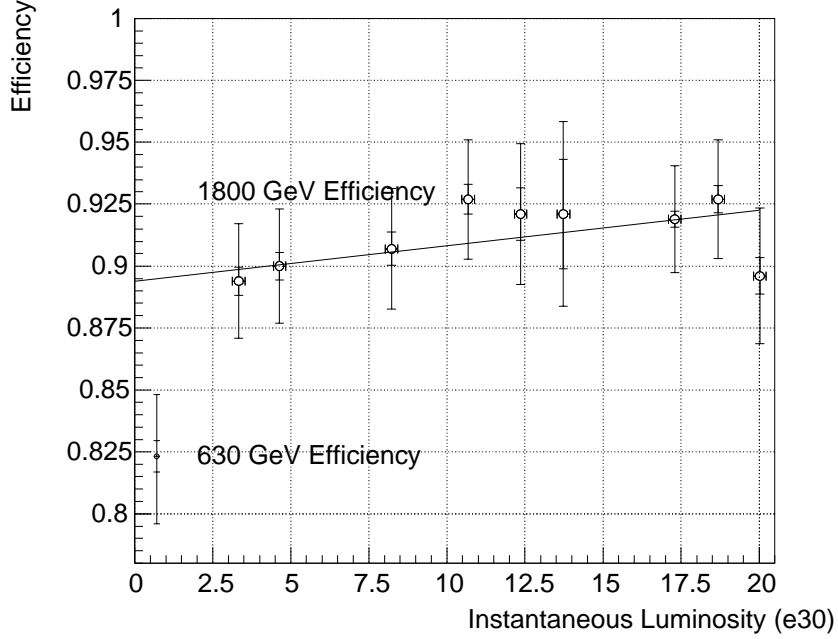
Figure 5.3: The Level Ø hardware efficiency at \sqrt{s} = 1800 and 630 GeV. The residual luminosity dependence is negligible over the luminosity range of the low-energy run ( 1 \cdot 10^{28} to 3 \cdot 10^{30} \text{ cm}^{-2} \cdot \text{sec}^{-1} ).
