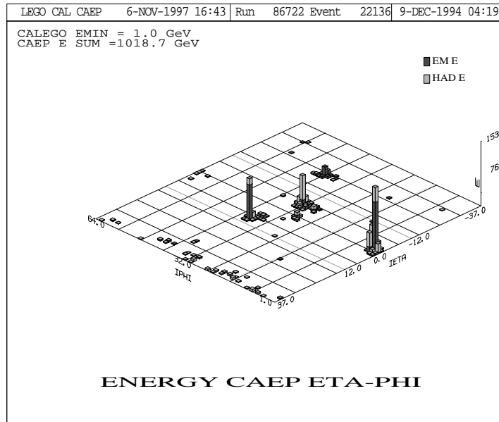
Figure 3.4: "Lego plot" of the D\bar{0} event.
