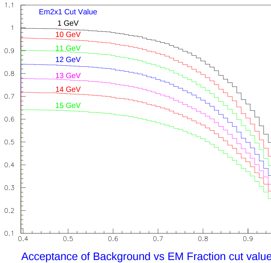
Figure G.3: The family of acceptance curves for di-electron events. A cut of 1 GeV shows the EM fraction acceptance without an Em2x1 cut.
