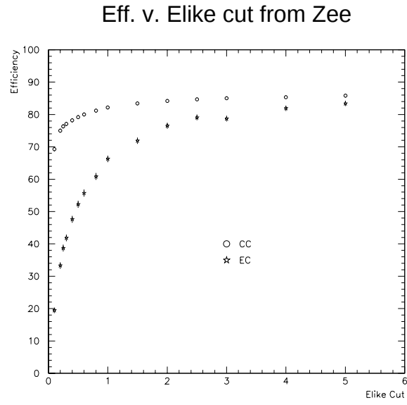
Figure 3.12: Efficiency spectra of electron likelihood cut. CC is the 5 variable, and EC is the 4 variable.
