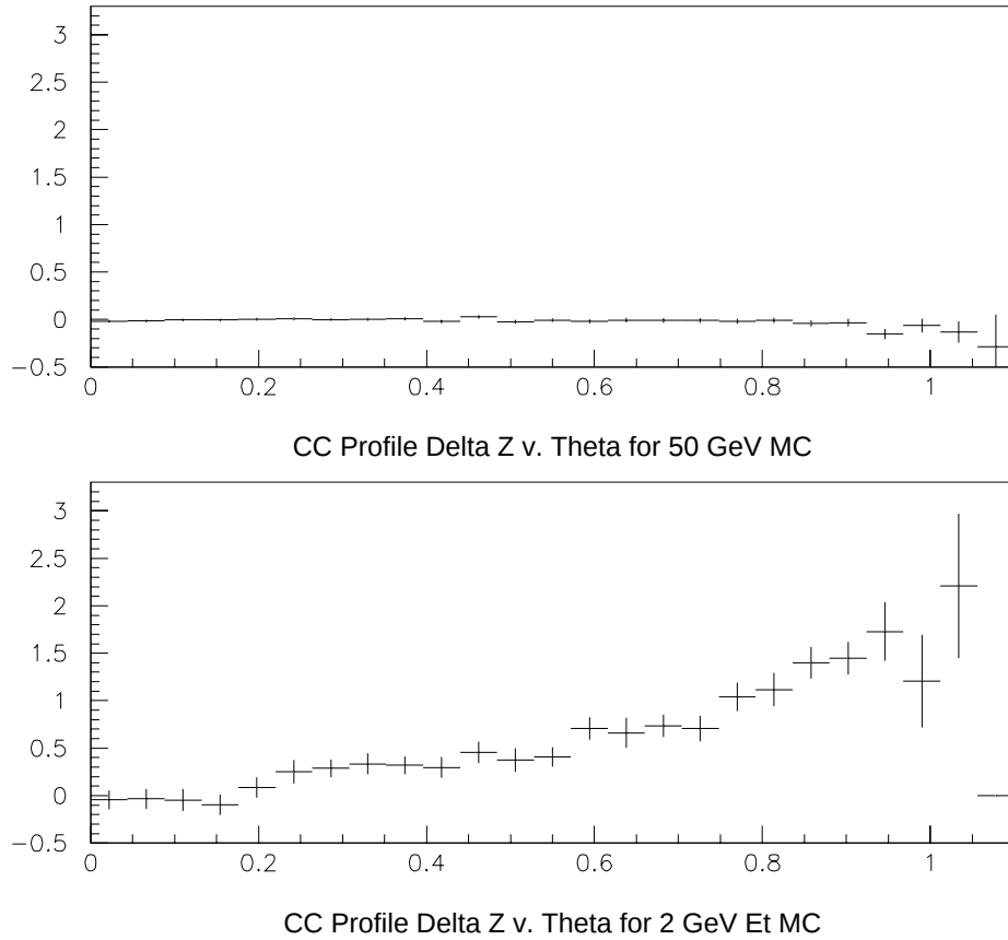
Figure H.1: Profile histograms for two samples of CC Monte Carlo electrons. The x-axis is the angle relative to normal incidence into EM3 in radians. The y-axis is the cluster determined z position in EM3 minus the Monte Carlo z position.
