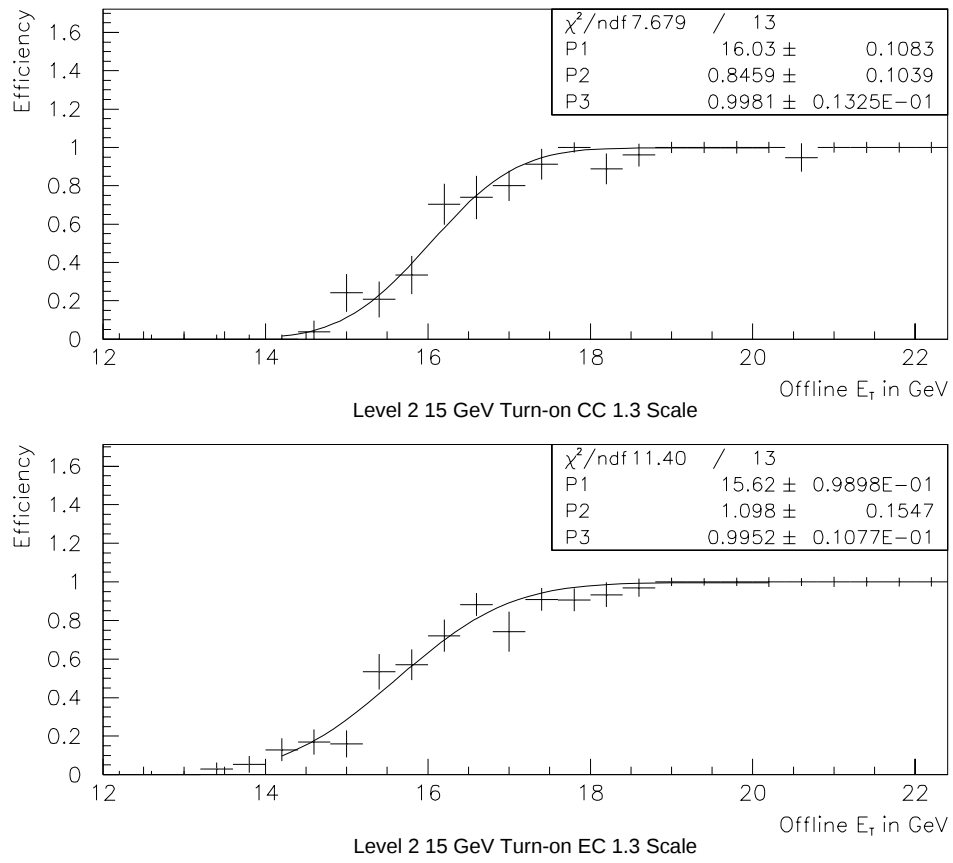
Figure 4.6: 15 GeV Level 2 threshold using a 30% scaling factor.
