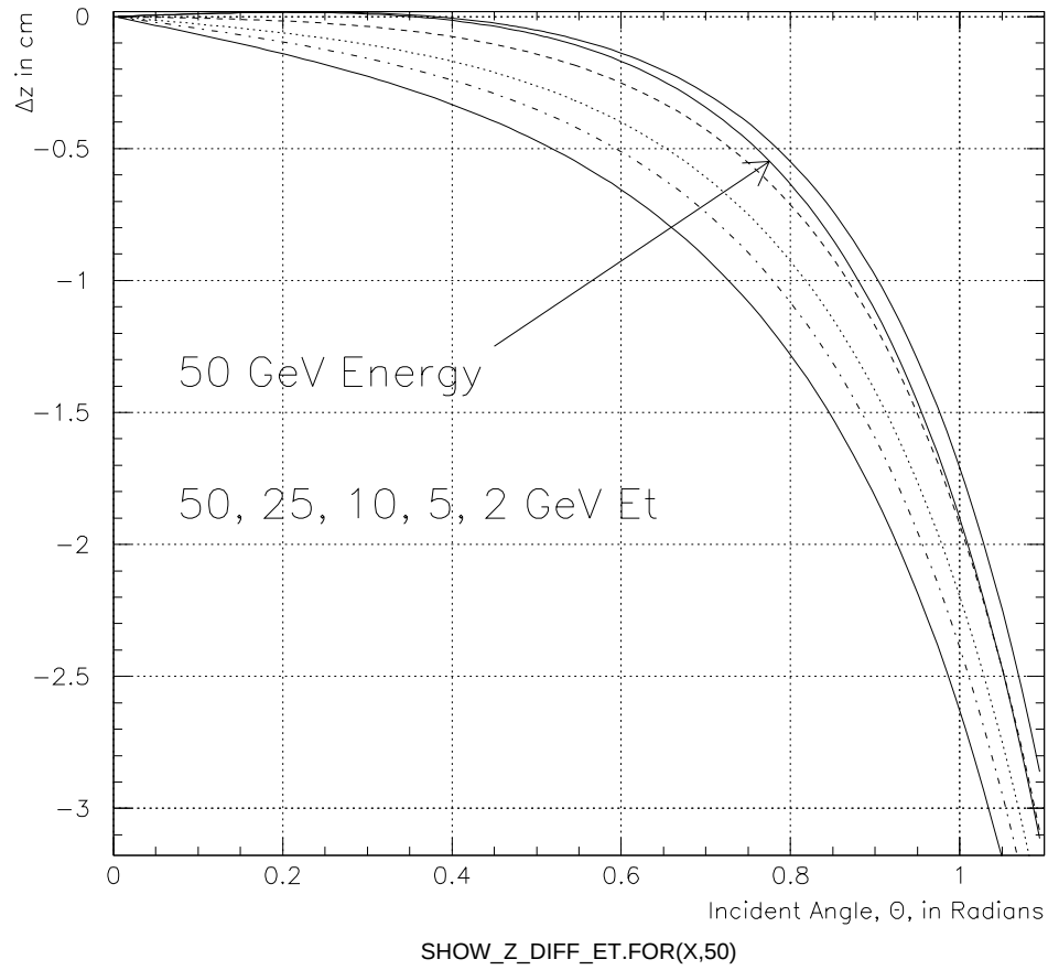
Figure H.7: Difference between EM3 z position at nominal and calculated radius, in cm, as a function of incident angle for transverse energies 50 (top curve), 25, 10, 5, and 2 GeV. Note the difference, about a mm, from the 50 GeV energy curve, and the two high E_T curves as compared with the Figure H.6
