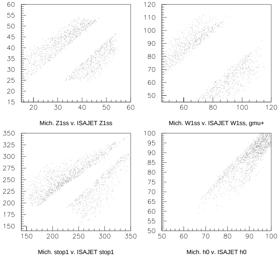
Figure C.10: Sample of mass spectra for \mu_G = \mu_H . The dearth of points along the diagonal indicates that the model generators use a different sign convention.
