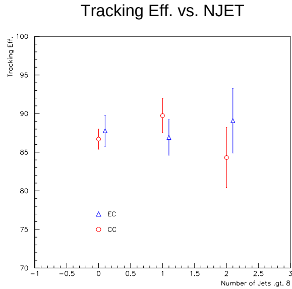
Figure 3.13: Tracking efficiency verses number of jets with E_T greater than 8 GeV.
