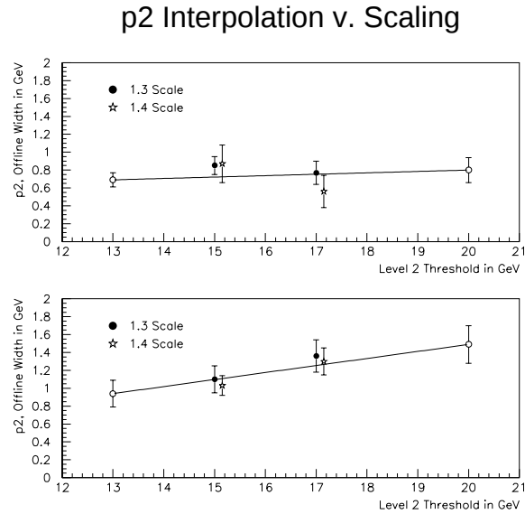
Figure 4.11: Comparison of results for p_2 between scaling and a linear interpolation between 13 and 20 GeV thresholds.
