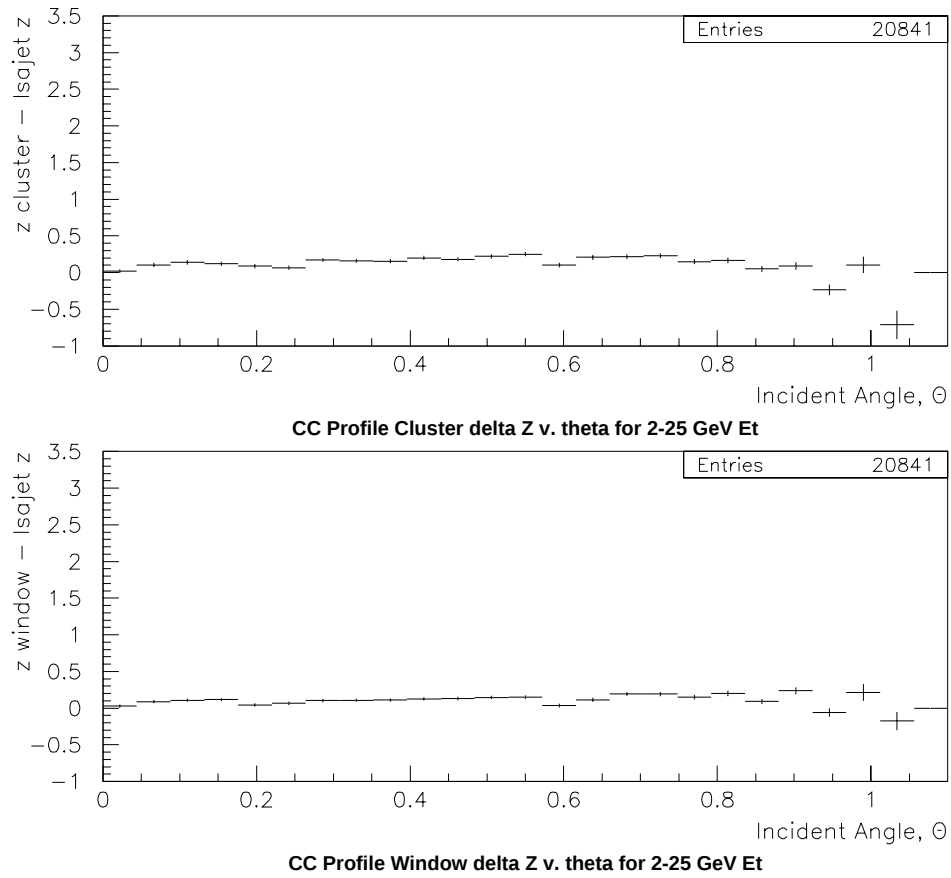
Figure H.12: Corrected z positions for 2 to 25 GeV E_T Monte Carlo, shown as a function of incident angle. Above is corrected for standard clusters, while below is for 1.5 \times 1.5 tower clusters.
