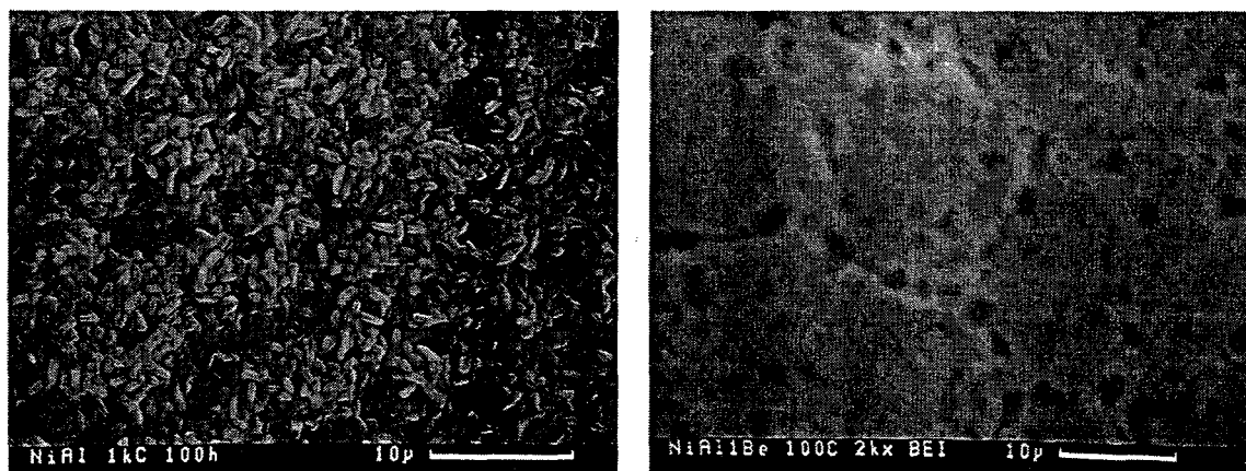
Figure 2: SEM (backscatter mode or secondary mode?) surface micrographs of \beta -NiAl (left) and Ni-49Al-1Be (right) after exposure for 100 h at 1000°C in air saturated with moisture at 20°C.
