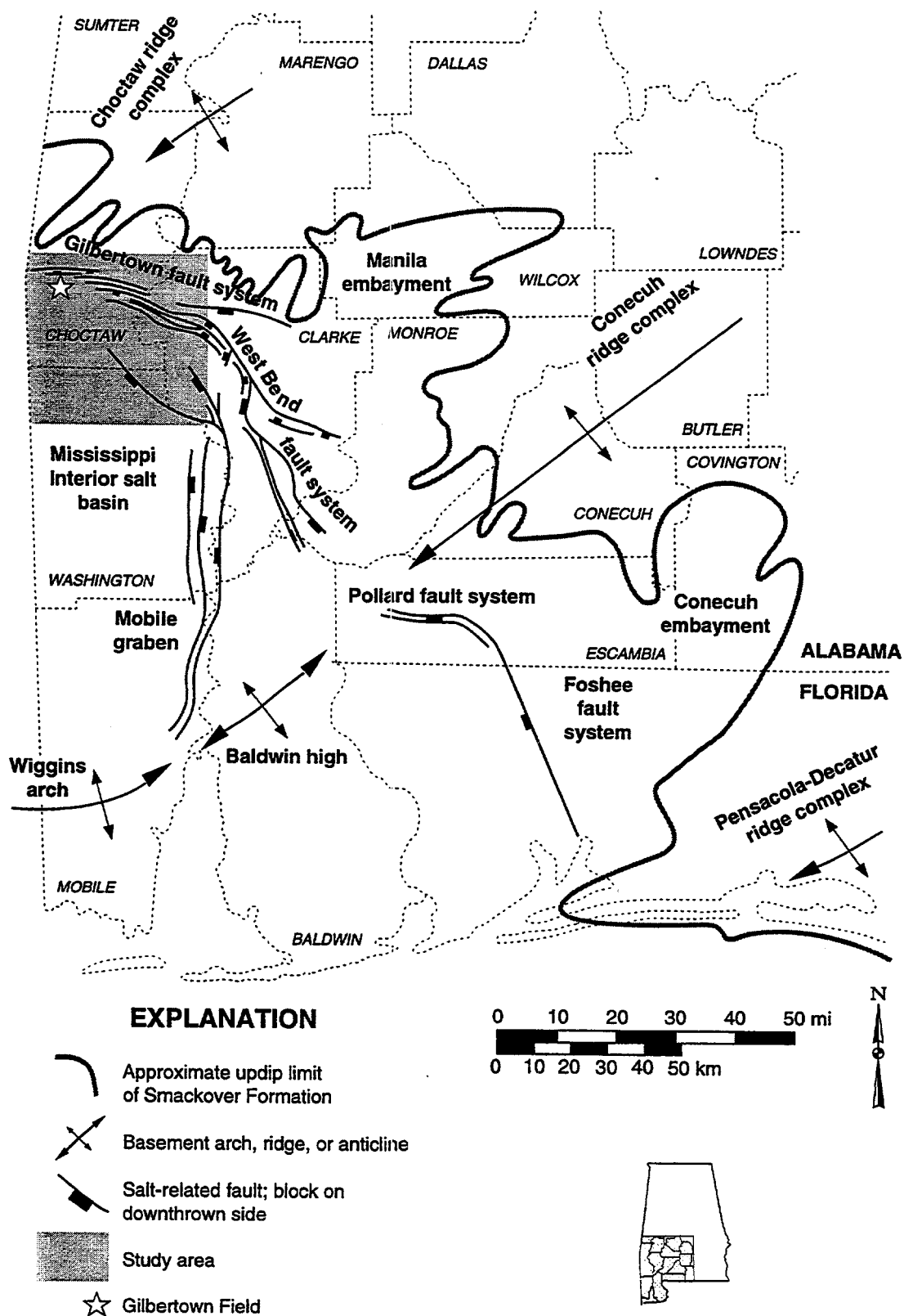
Figure 1.--Structural features in the Gulf Coast basin of southwest Alabama with location of study area and Gilbertown Field (modified from Mancini and others, 1991).
