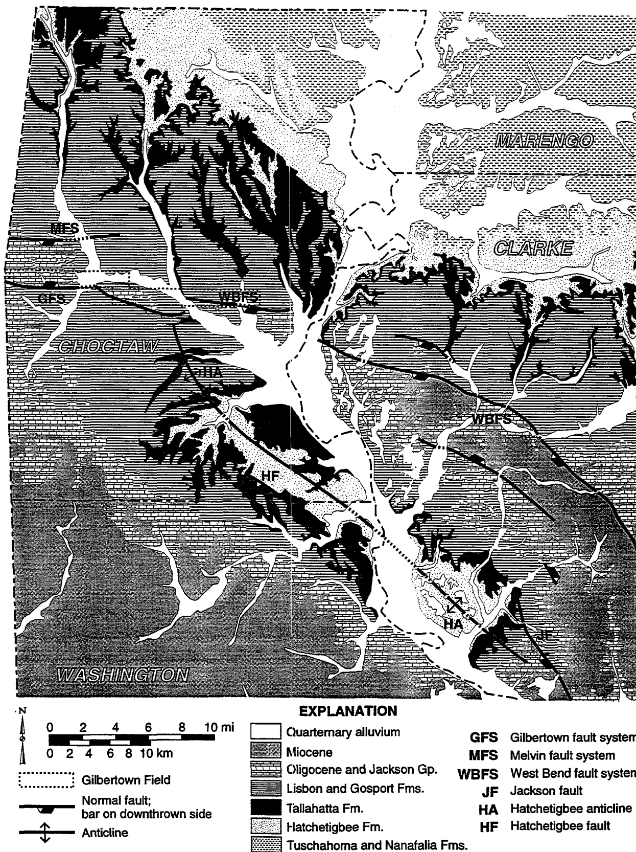
Figure 29.--Generalized geologic map of the Gilberttown fault system and Hatchetigbee anticline (modified from Szabo and others, 1988).
