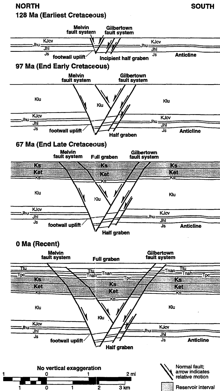
Figure 28.--Sequential restoration showing evolution of the graben formed by the Gilberttown and Melvin fault systems. Restoration based mainly on cross section E-E' (fig. 15).
