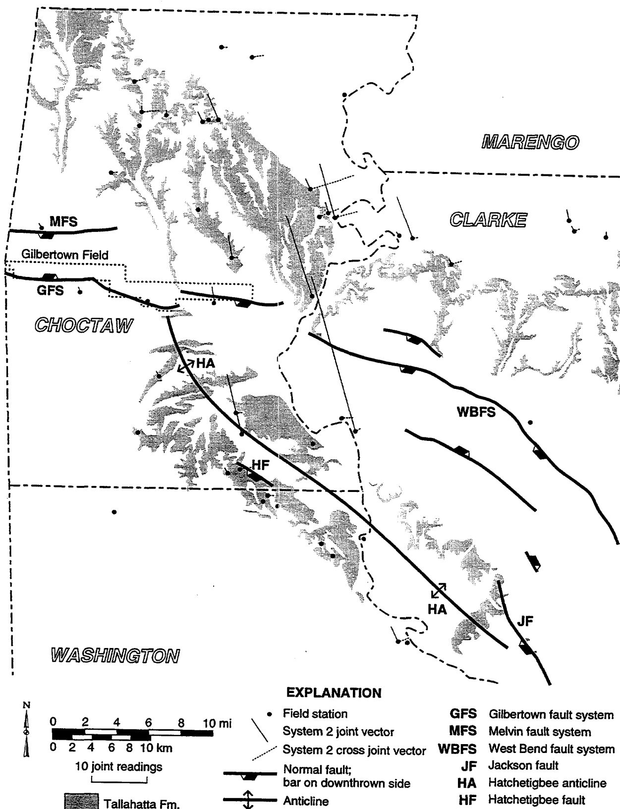
Figure 35.--Map of weighted system 2 joint vectors in the Gilbertown area.
