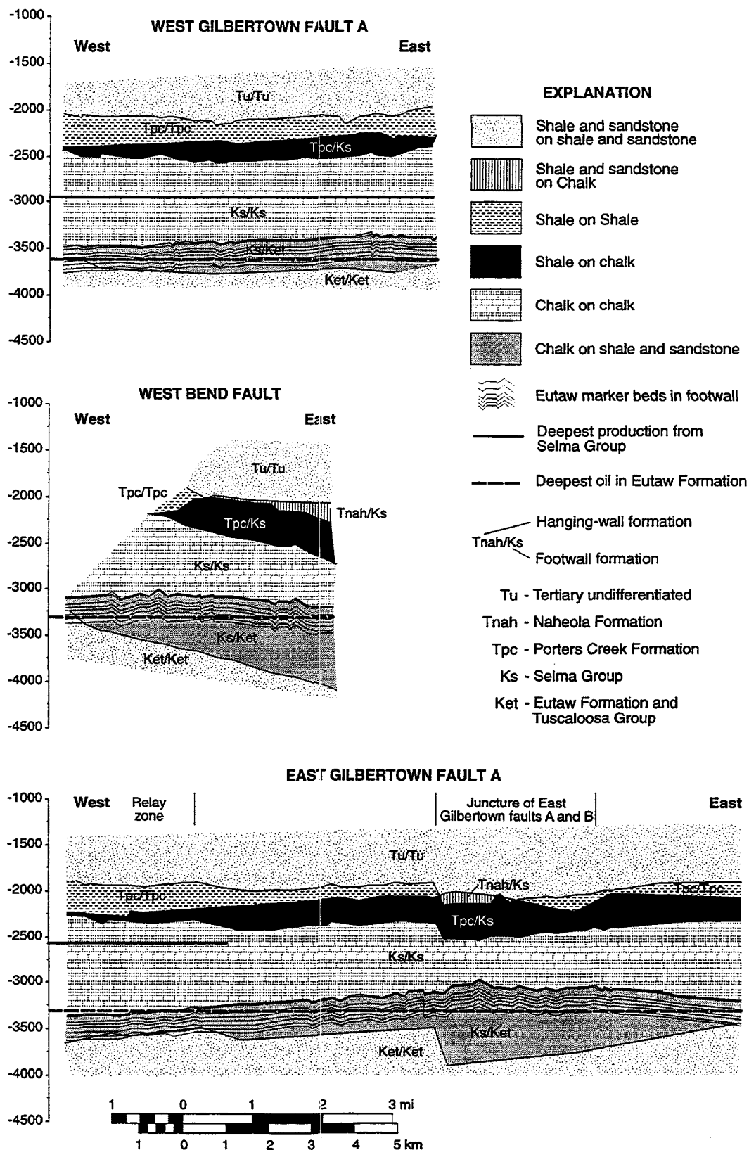
Figure 86.--Juxtaposition diagrams showing formations in contact along the Gilbertown and West Bend fault systems. Data projected to vertical planes striking east.
