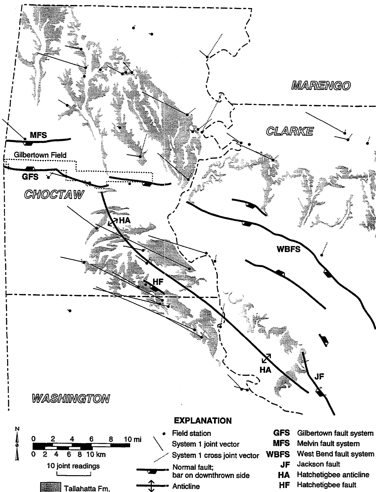
Figure 33.--Map of weighted system 1 joint vectors in the Gilberttown area.
