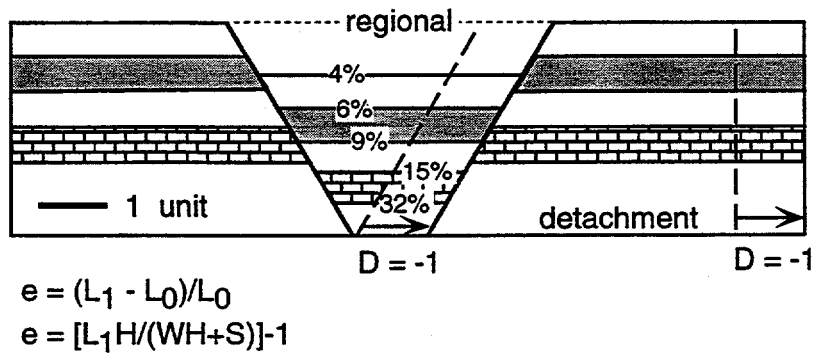
Figure 8.--Structural diagrams showing area-depth-strain relationships in extensional structures (modified from Groshong, 1994, Pashin and others, 1995).
