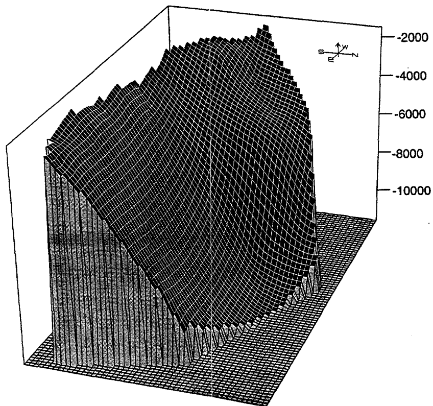
Figure 82.--Three-dimensional grid plots of faults where oil has been produced from the Selma Group in Gilbertown Field. Plots generated using Geographix Isomap.
