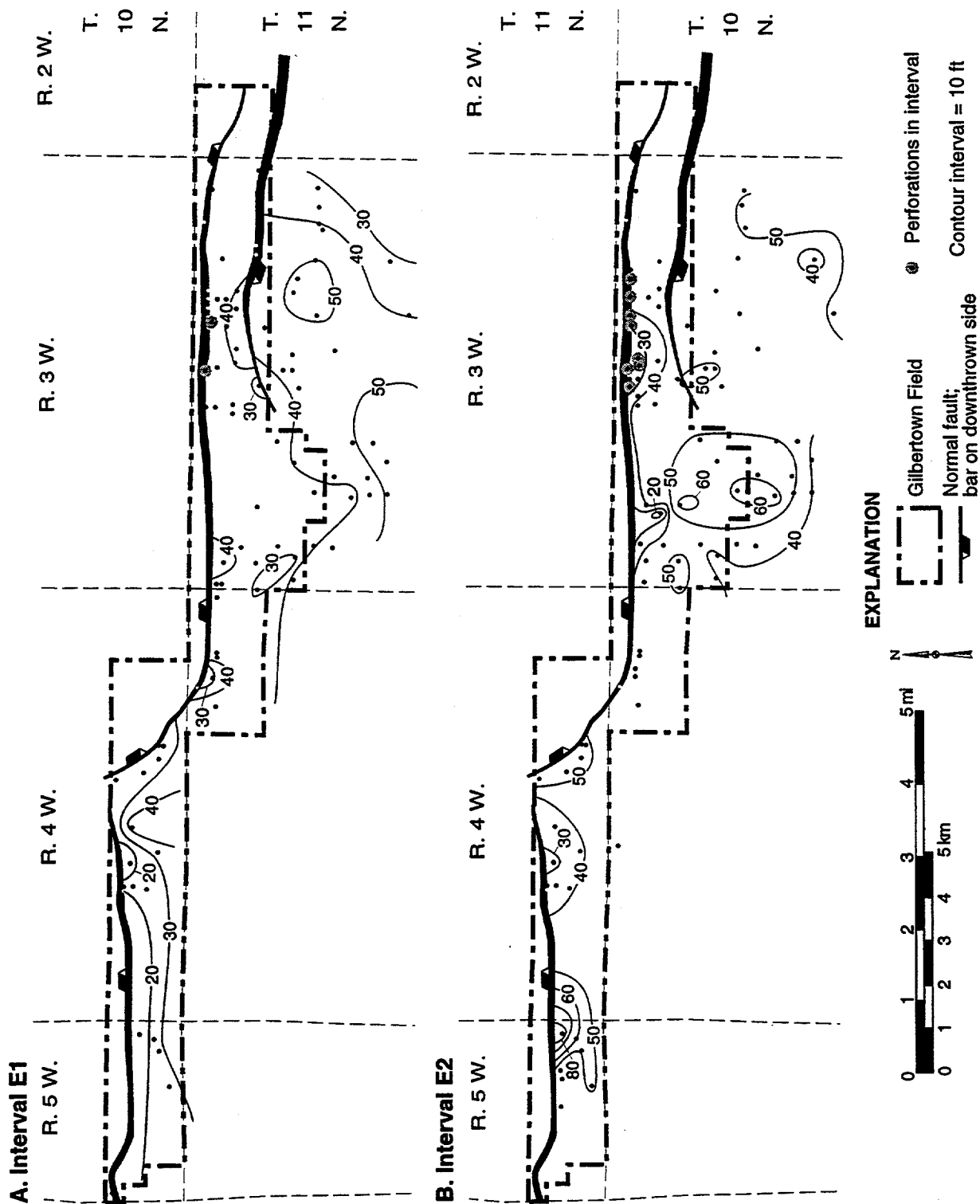
Figure 53.--Net sandstone isolith maps of intervals E1 and E2, Gilbertown Field and adjacent areas.
