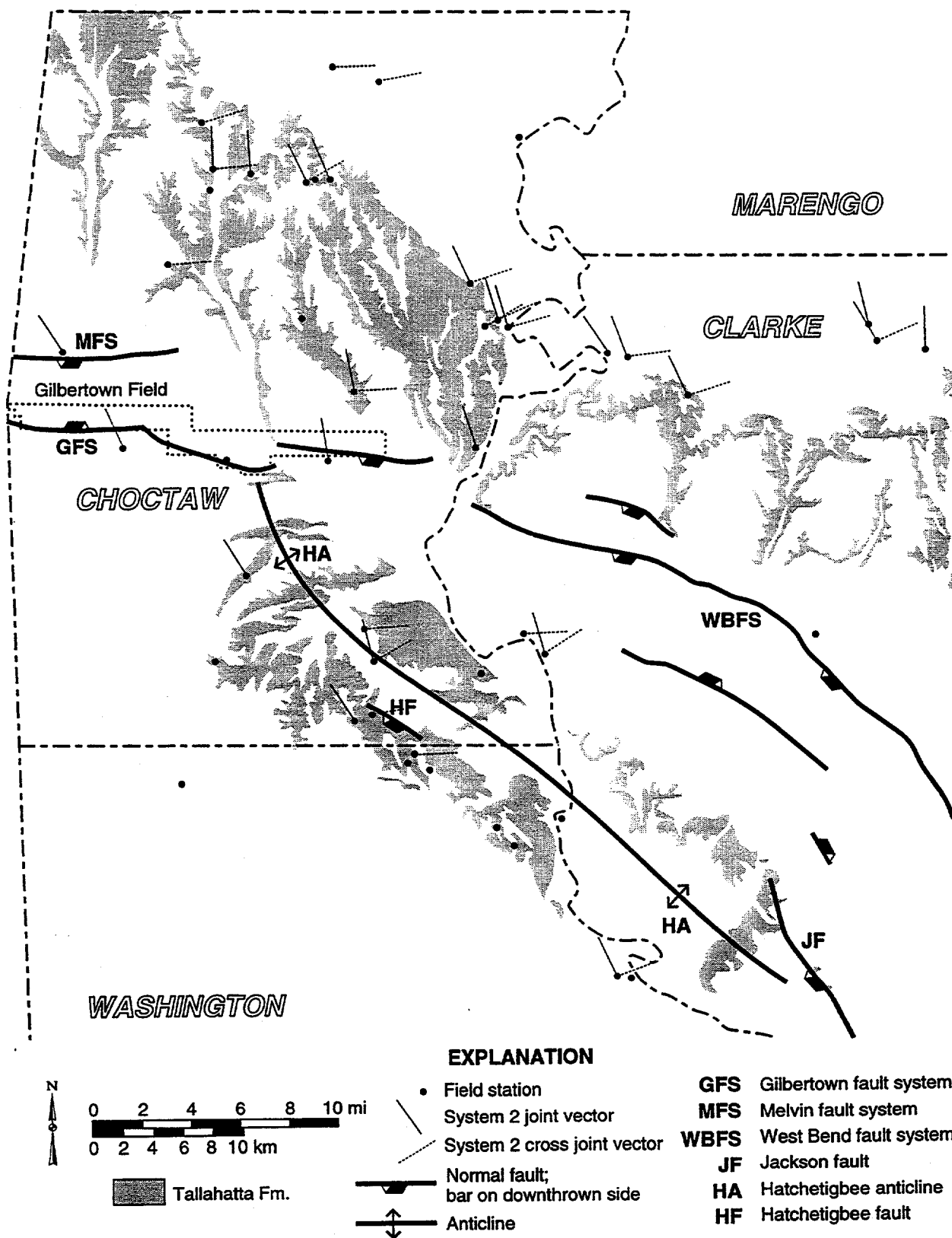
Figure 34.--Map of raw system 2 joint vectors in the Gilbertown area.
