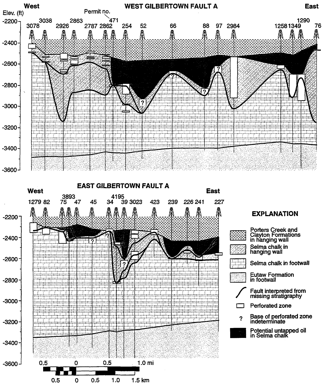
Figure 98.--Strike cross sections showing distribution of completed zones in the Selma Group and possible untapped oil column below reservoir topseal.
