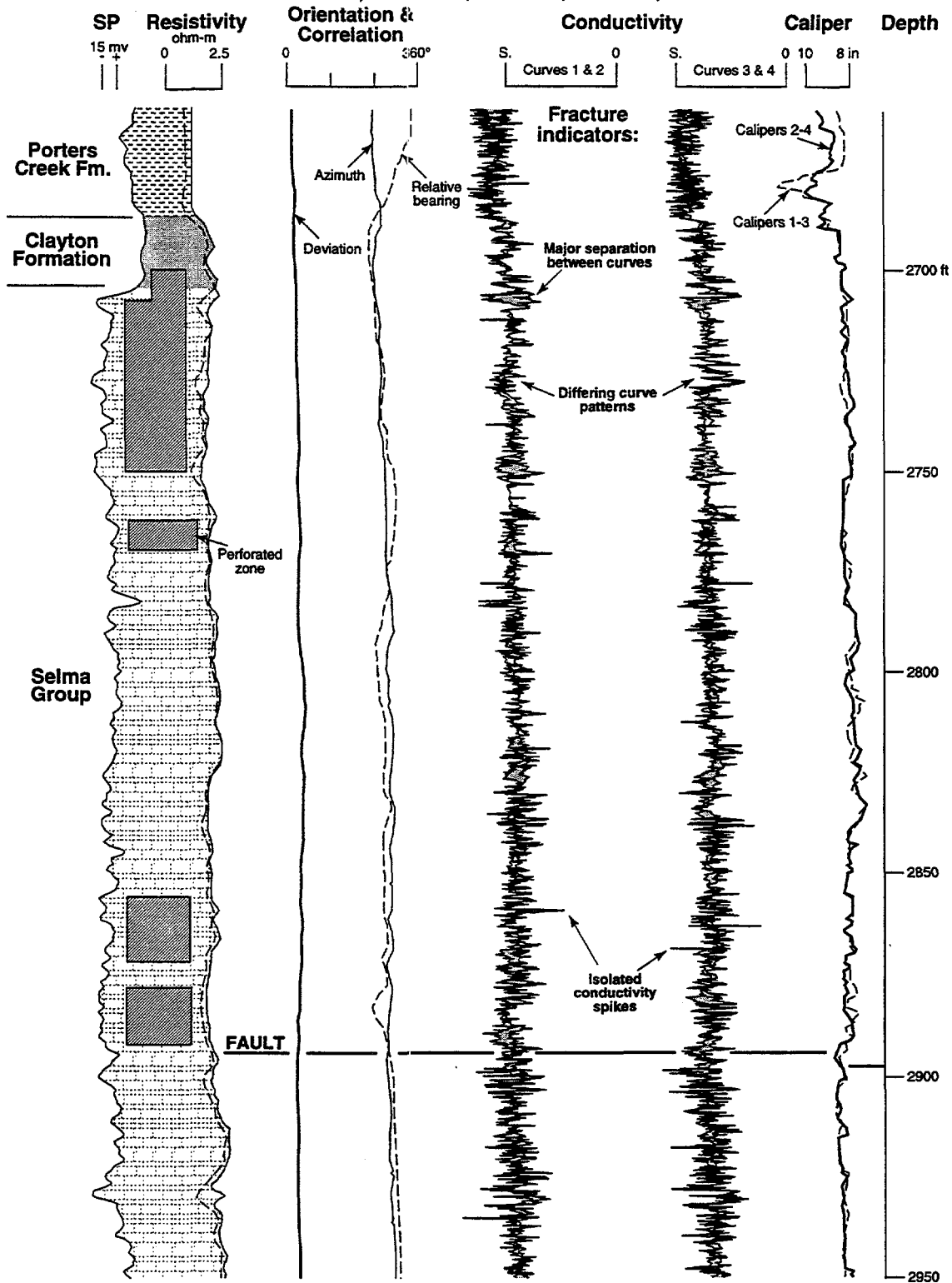
Figure 72.--Fracture identification log (FIL) of the upper part of the Selma Group in Gilbertown Field. Perforated zones were chosen on the basis of FIL characteristics.
